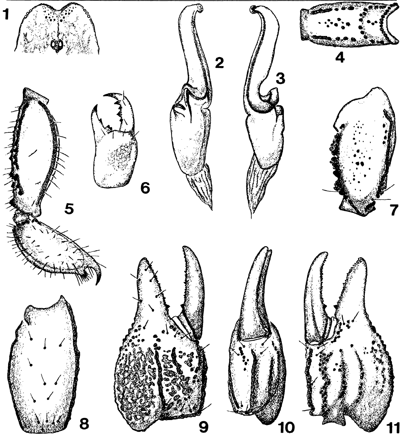
Figs. 1-5. Morphology of Diplocentrus colwelli , new species: 1, anterior portion of carapace; 2, right hemisphermatophore, mesal view; 3, right hemisphermatophore, lateral view; 4, ventral aspect of metasomal segment V; 5, lateral aspect of metasomal segment V and telson.
