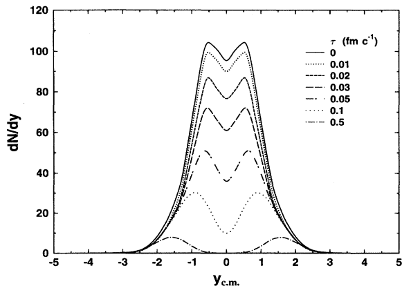
FIG. 14. Antiproton rapidity spectra in central Au+Au collisions at RHIC bombarding energy for different values of deceleration time. In all cases the rapidity shift \delta y=2.4 is assumed.
