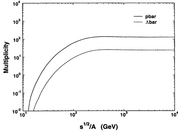
FIG. 9. Excitation functions of antiprotons (solid line) and anti-lambdas (dashed line) produced by the bremsstrahlung mechanism in central Au+Au collisions.
