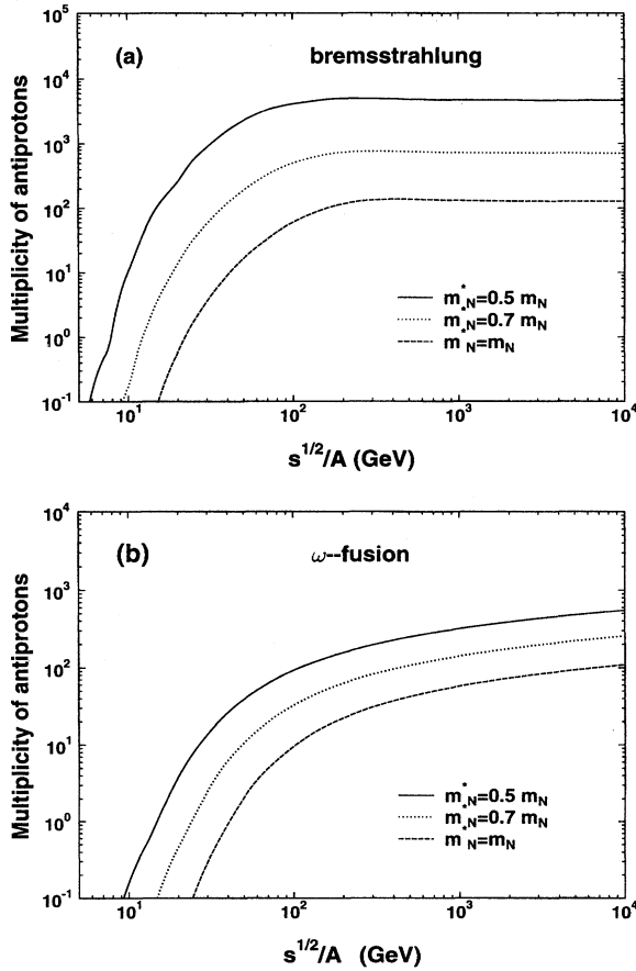
FIG. 10. Excitation functions of antiprotons in central Au+Au collisions produced by the bremsstrahlung (a) and \omega -fusion (b) mechanisms. Results are shown for three different values of the nucleon effective mass m_N^* .
