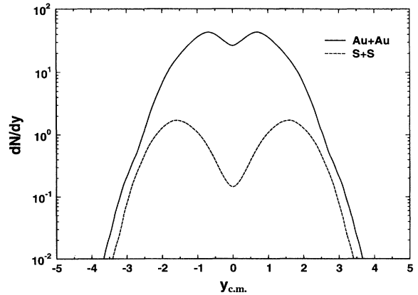
FIG. 12. Antiproton rapidity spectra in central Au+Au (solid line) and S+S (dotted line) collisions at RHIC energy \sqrt{s}=200A GeV. Only bremsstrahlung contributions are shown. The rapidity shifts are \delta y=2.4 (Au+Au) and 1.6 (S+S).
