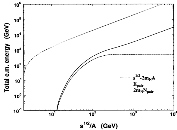
FIG. 6. Total c.m. energy E_{\text{pair}} of N\bar{N} pairs produced by bremsstrahlung in central Au+Au collisions (solid line). Dotted and dashed lines correspond to total available energy, \sqrt{s} - 2m_N A and total mass of pairs, 2m_N N_{\text{pair}} , respectively.
