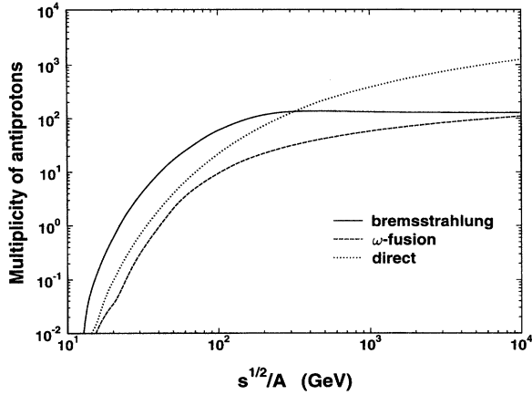
FIG. 5. Antiproton multiplicity in central Au+Au collisions versus c.m. bombarding energy per baryon. Solid and long dashed show the bremsstrahlung and \omega -fusion contributions. Dotted line represents the direct \bar{p} yield.
