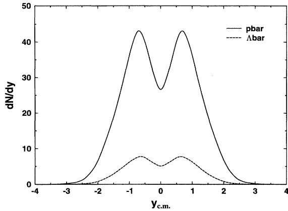
FIG. 13. Rapidity spectra of antiprotons (solid line) and anti-lambdas (dashed line) produced by the bremsstrahlung mechanism in central Au+Au collisions at RHIC energy.
