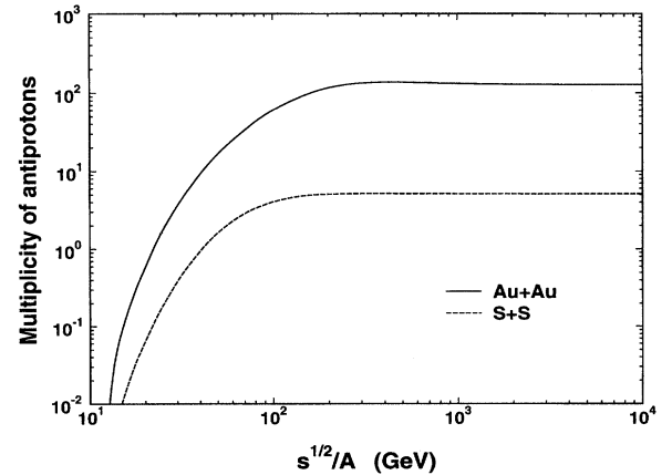
FIG. 8. Excitation functions of antiprotons (bremsstrahlung contribution) in central Au+Au and S+S collisions.
