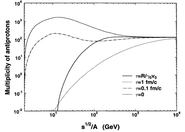
FIG. 7. Excitation function of antiprotons produced by bremsstrahlung in central Au+Au collisions. Solid line corresponds to the deceleration time \tau equal to half of the passage time. Dotted and dashed-dotted lines are calculated for constant deceleration times \tau = 1 and 0.1 fm/c. Dashed line corresponds to the instantaneous deceleration ( \tau = 0 ).
