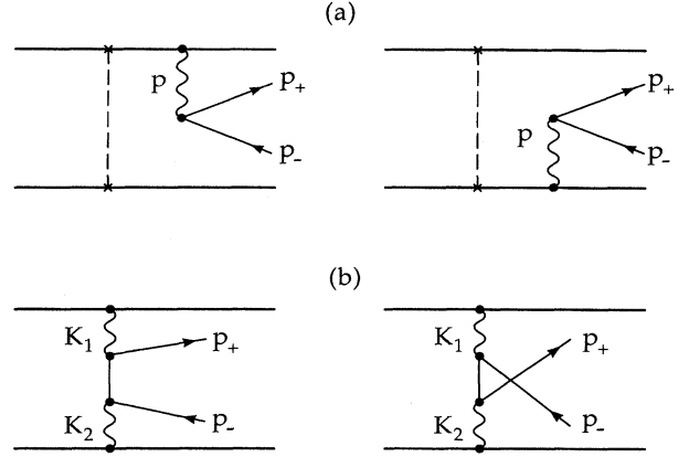
FIG. 1. Lowest order Feynman diagrams for the production of N\bar{N} pair in nuclear collisions. Parts (a) and (b) correspond, respectively, to bremsstrahlung and second order (fusion) processes. Wavy lines denote mean-field interaction. Thin solid lines denote propagation of fermions. Upper and lower thick lines correspond to projectile and target nuclei, respectively. Dashed line shows an arbitrary interaction which causes mutual deceleration of nuclei.
