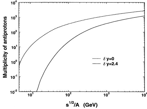
FIG. 4. Multiplicity of direct antiprotons in central Au+Au collisions as a function of c.m. bombarding energy per nucleon. Dashed line shows the result of calculation in the free-streaming approximation. Solid line is calculated with inclusion of deceleration effects assuming the rapidity loss \delta y = 2.4 .
