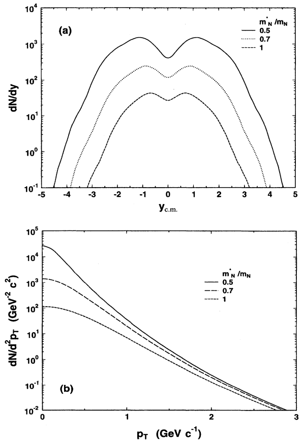
FIG. 16. Rapidity (a) and transverse momentum (b) spectra of antiprotons produced by the bremsstrahlung mechanism in central Au+Au collisions at RHIC energy. Results are shown for three different choices of the nucleon effective mass m_N^* .
