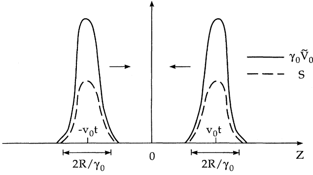
FIG. 2. Scalar (dashed line) and vector (solid line) meson potentials before a central collision of identical nuclei shown as a function of longitudinal coordinate z in the equal velocity frame (schematic view). Only time-like component of vector potential is shown ( \tilde{V}_0 is the corresponding potential in the nucleus rest frame).
