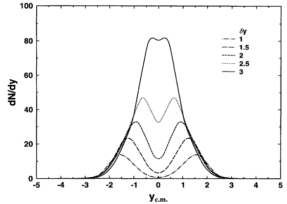
FIG. 15. Same as in Fig. 14, but for different values of rapidity shift \delta y .
