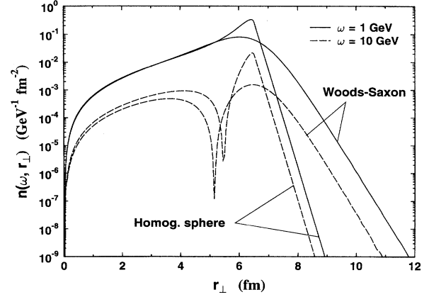
FIG. 3. Spectral density of virtual vector mesons for gold nucleus as function of distance r_{\perp} from the beam axis ( \sqrt{s} = 200A GeV). Solid and dashed lines correspond to the meson energy \omega = 1 and 10 GeV in the equal velocity frame.
