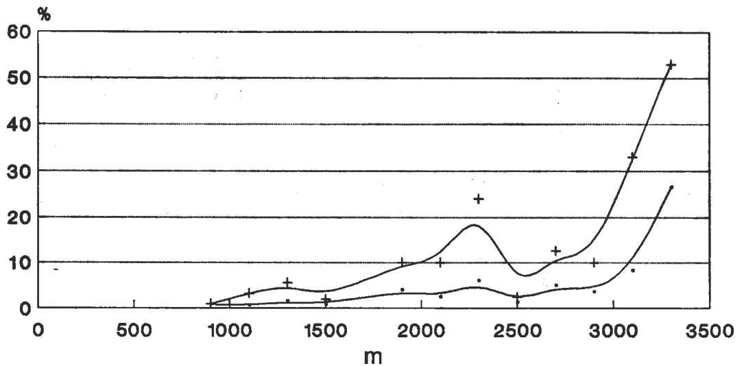
Fig. 6.5: Minima and maxima of relative light intensity in percent (as compared to the situation outside the forest) at the bottom of rain forests in Eastern Cong/Uganda. The light increases slightly from the montane to the high montane forest and reaches maxima in the subalpine forest.
