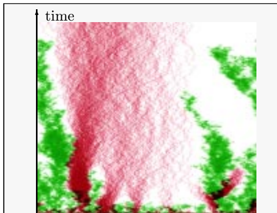
Figure 2 CBRW on the torus \mathbb{Z}/(500) . a and b are symmetric simple. The catalyst (green) is the same realization as in Figure 1. The reactant (red) survives. See Theorem 2 (a).
