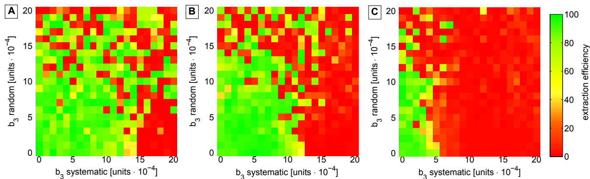
Figure 5: 2D histograms showing the extraction efficiency as a function of the systematic and random sextupole field components in the dipole magnets. A: the systematic and random components are known and have been compensated. B: only the systematic component is known and has been compensated. C: no component is known, and no compensation is applied. A different random seed has been used for each grid point
