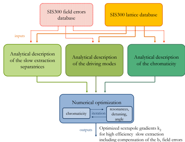
Figure 1: Scheme of the optimization procedure.
