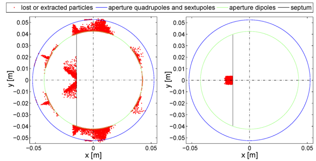
Figure 3: Left: Losses produced in the apertures of the magnets and on the electrostatic septum, for the original lattice. No beam can be extracted in this case. Right: No losses are produced in the magnet apertures of the optimized lattice. All the beam is extracted at the electrostatic septum, where an extraction efficiency of 96.4% is reached.
