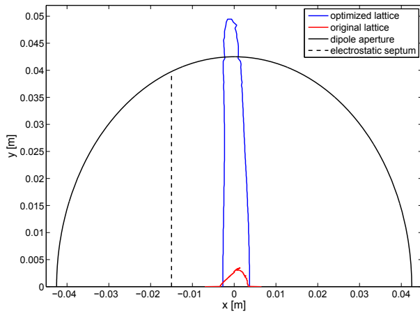
Figure 2: Short-term dynamic apertures of the original and optimized lattices, represented together with the apertures of the dipole magnets and electrostatic septum.
