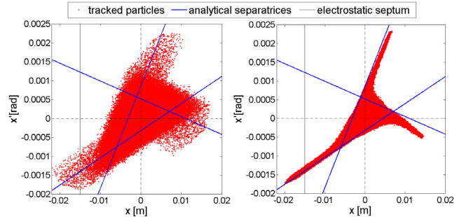
Figure 4: Phase-space plots of a multi-particle simulation for slow extraction. The left figure shows the widening of the separatrices caused by the b_3 field errors in the dipole magnets. The extraction efficiency in the presence of the predicted field error decreases down to 80%. The right figure shows the effect of the compensation by means of a new set of optimized gradients for all sextupole families. An extraction efficiency of 93.6%, similar to that of the lattice with ideal magnets is recovered.
