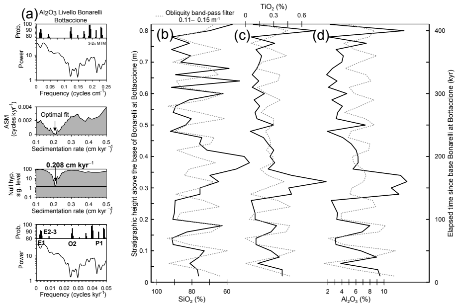
Figure 5. (a) Duration estimate of Livello Bonarelli at Bottaccione based on the average spectral misfit (ASM) method. (b–d) SiO 2 , TiO 2 and Al 2 O 3 data show ~8 cm thick cycles, interpreted as obliquity. The duration of the Livello Bonarelli at Bottaccione is estimated at 410 kyr.
