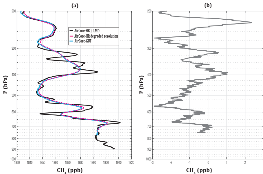
Figure 14. (a) \text{CH}_4 vertical profiles from AirCore-HR in full resolution (black), from AirCore-HR in “degraded resolution” (pink) and from AirCore-GUF (blue). (b) Residual of the difference AirCore-GUF–AirCore-HR in “degraded resolution”.
