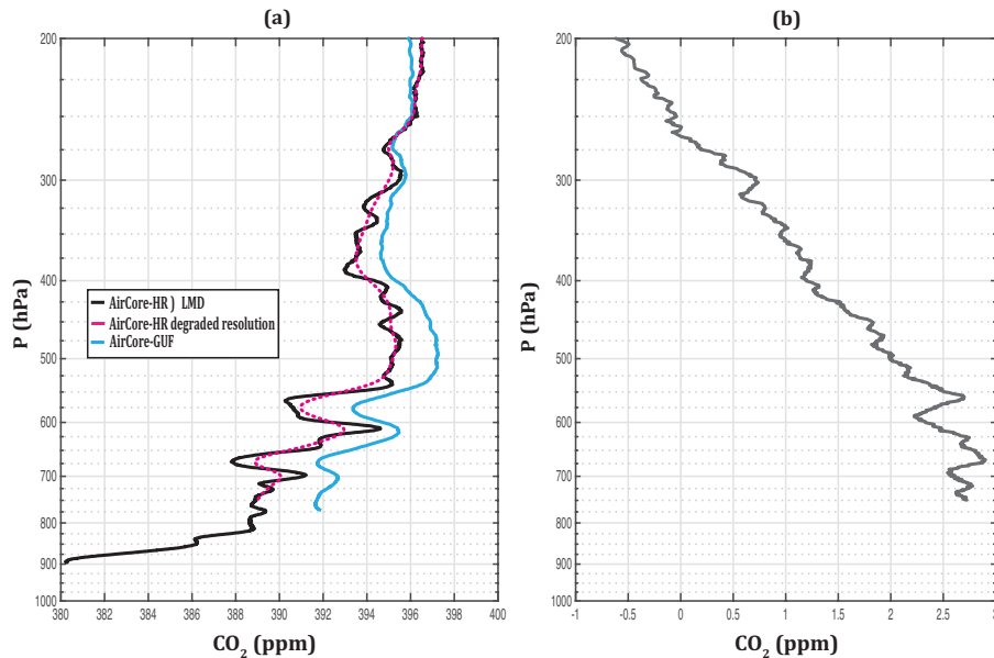
Figure 13. (a) \text{CO}_2 vertical profiles from AirCore-HR in full resolution (black), from AirCore-HR in “degraded resolution” (pink) and from AirCore-GUF (blue). (b) Residual of the difference AirCore-GUF–AirCore-HR in “degraded resolution”.
