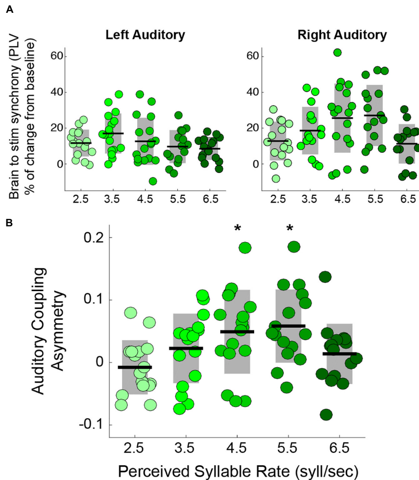
FIGURE 1 | Rightward dominance is affected by speech rate during a syllable perception task. (A) PLV between auditory cortices and speech envelope, increment from resting state. Mean PLV around the syllable rate of each condition (syllable rate \pm 0.5 Hz). Left auditory synchronization shows no change between conditions (Kruskal-Wallis test: \chi^2(4) = 5.6 , two-sided p = 0.23 ). However, the right auditory cortex does (Kruskal-Wallis test: \chi^2(4) = 12.45 , two-sided p = 0.014 ) (Adapted from Assaneo and Poeppel, 2018). (B) Auditory coupling asymmetry for the different syllable rate conditions: the degree of asymmetry is modulated by the syllable rate (Kruskal-Wallis test: \chi^2(4) = 13.63 , two-sided p = 0.008 ). The asymmetry is significantly above zero only for 4.5 and 5.5 syllables per second. * Stands for two-sided p < 0.05 (Wilcoxon Signed-Rank test, FDR corrected). Dots: individual participants, the scattering in the X-axis is for visualization purposes. Black lines: mean across participants. Shaded region: SD. N = 17 .
