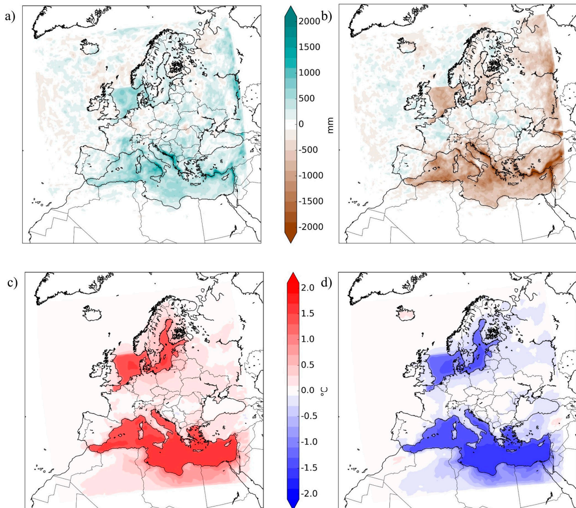
Figure 3. Difference between the SST_0 and the SST -2 (left column, a,c) or the SST +2 (right column, b,d) simulations. The first row (a,b) shows the difference of the precipitation sums during the whole time period (2000–2003) and the second row (c,d) shows the differences in 2 m temperature mean.
