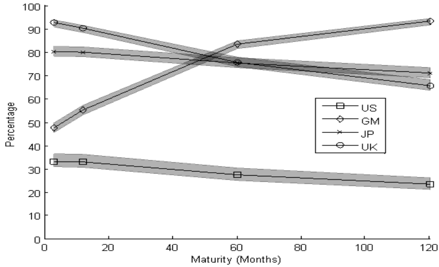
Figure 6a Variance Decomposition of Country Yields, 1985:09-1995:08
