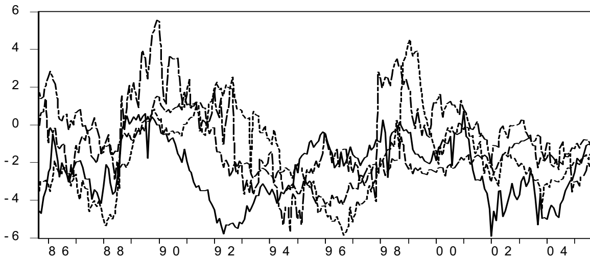
Figure 2b: Estimated Country Slope Factors
