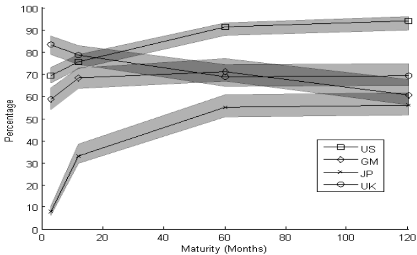
Figure 6b Variance Decomposition of Country Yields, 1995:09-2005:08
