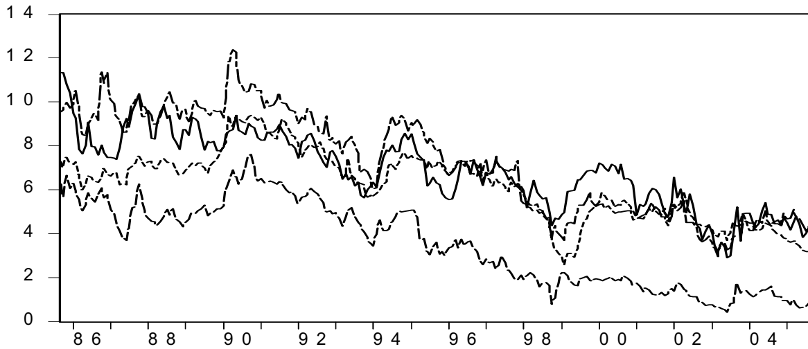
Figure 2a Estimated Country Level Factors
