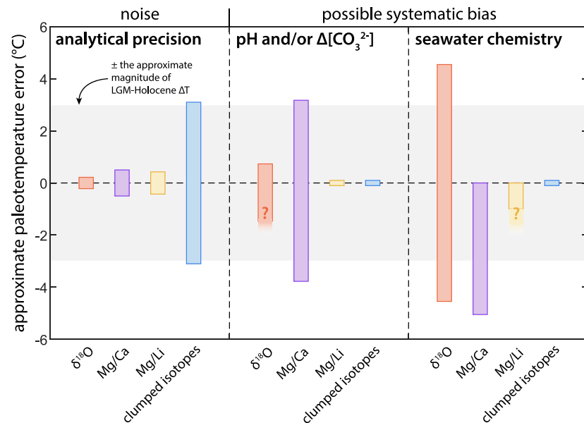
Figure 1. The approximate magnitude of the various sources of uncertainty affecting some common deep ocean temperature proxies based on the geochemistry of benthic foraminifera. Note that this assumes the worst-case scenario that no constraints on these nonthermal controls exist, which is often not the case. In addition, relative temperature reconstructions can be much more precise than this figure implies (e.g., relative changes cannot be biased if the study interval is shorter than that over which seawater chemistry can change, although the absolute temperature reconstructions may be biased if seawater chemistry was different to modern). The magnitude of the bars relating to seawater chemistry reflect both the degree and the direction which these parameters have varied in the Neogene only. The figure is intended as an approximate guide; these values may be species/site specific. A pH ( \text{CO}_3^{2-} ) effect on foraminifera \delta^{18}\text{O} has been suggested (Zeebe, 1999) but not (yet) found in benthic species (Marchitto et al., 2014). The effect of seawater chemistry on the Mg/Li proxy is not constrained (little is known about the possible secular evolution of seawater [Li]).
