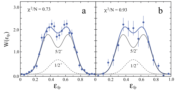
Fig. 3. Fractional energy spectra W(\epsilon_{fp}) in the Y-system for the region of 15 O + p + p internal energy 0 \leq E_{fpp} \leq 1.4 MeV from the CH 2 target (a) and Pb target (b). The distributions stem from the unresolved resonances 17 Ne( 5/2^- ) and 17 Ne( 1/2^+ ) decaying to the 16 F ground state. A fit with only one free parameter gives their relative contributions.
