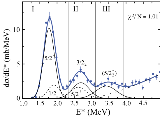
Fig. 2. Narrow resonance states in the low-energy region, 0 < E^* < 4 MeV excited in the CH 2 target. The thin solid lines show negative-parity states, dashed lines stem for positive-parity states and the dash-dotted line is physical background. For energy regions I, II and III the fractional energy spectra are analysed as shown in Figs. 3, 4 and 5, respectively.
