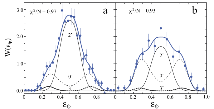
Fig. 4. Fractional energy spectra W(\epsilon_{fp}) in the Y-system for the region of 15 O + p + p internal energy 1.4 \leq E_{fpp} \leq 2.2 MeV from the CH 2 target (a) and Pb target (b). Thin solid and thick dashed lines show decays through the intermediate 16 F( 2^- ) and 16 F( 3^- ) states, respectively. These states have the structure of 15 O with one proton in the d-shell. The dashed lines represent decays to the 16 F( 0^- ) state with the structure 15 O with one proton in the s-shell.
