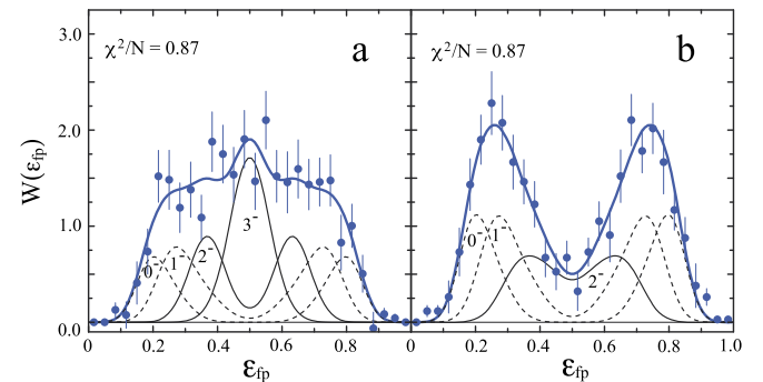
Fig. 5. Fractional energy spectra in the Y-system W(\epsilon_{fp}) for the region of 15 O + p + p internal energy 2.2 \leq E_{fpp} \leq 3.0 MeV from the CH 2 target (a) and Pb target (b). The thin solid lines show decays to 16 F( 2^- and 3^- ) states and the dashed lines represent decays to 16 F( 0^- and 1^- ) states.
