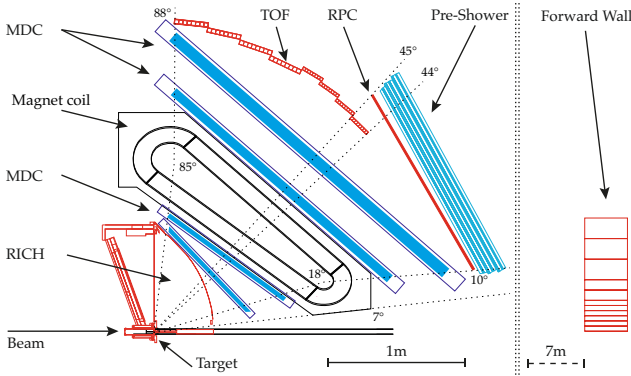
Fig. 1. Cross section of one sector of the HADES spectrometer. The segmented target irradiated by the beam, the RICH detector, the magnet spectrometer consisting of four layers of drift chambers (MDC) and the magnet coils, the two time-of-flight detectors (TOF and RPC) and the Forward Wall (FW) are shown. The maximal acceptance in polar angle for charged particles, defined by the coverage of the magnetic field, is between 18^\circ and 85^\circ , which corresponds to a rapidity range for protons of -0.6 < y - y_{cm} < 0.8 ( y_{cm} = 0.74 ).
