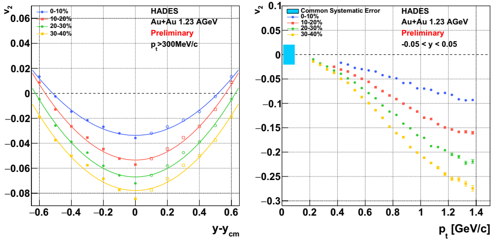
Fig. 4. Preliminary data on elliptic flow ( v_2 ) of protons measured with HADES in different centrality intervals of Au+Au collisions at 1.23A GeV. The left panel shows the p_T integrated v_2 as a function of the centre-of-mass rapidity, while in the right panel v_2 at mid-rapidity is presented as a function of p_T .
