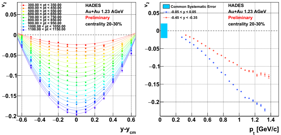
Fig. 3. Preliminary data on elliptic flow ( v_2 ) of protons measured with HADES in semi-central (20 – 30%) Au+Au collisions at 1.23A GeV. The left panel shows v_2 as a function of the center-of-mass rapidity in transverse momentum intervals of 50 MeV/c (lines are to guide the eye). The right panel displays the p_t dependence of v_2 in two different rapidity intervals.
