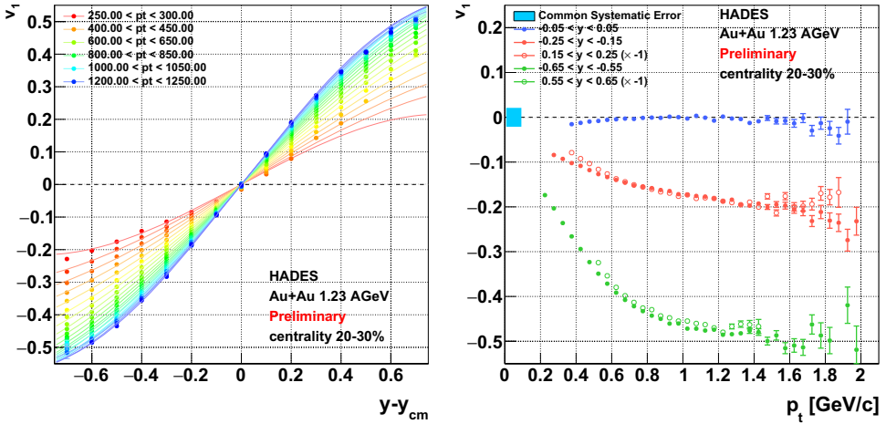
Fig. 2. Preliminary data on directed flow ( v_1 ) of protons measured with HADES in semi-central (20 – 30%) Au+Au collisions at 1.23A GeV. The left panel shows v_1 as a function of the center-of-mass rapidity in transverse momentum intervals of 50 MeV/c (lines are to guide the eye). In the right panel, a comparison of the p_t dependence of v_1 in five rapidity intervals, symmetric around mid-rapidity, is presented.
