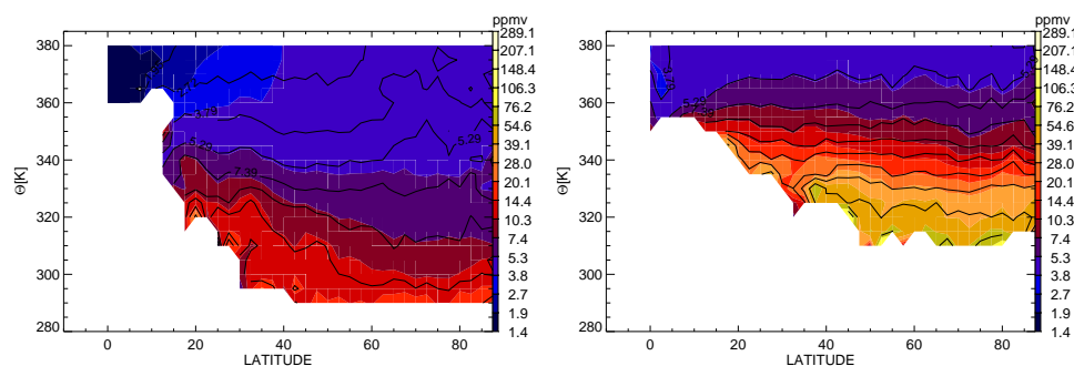
Fig. 9. Mean saturation mixing ratio of the TST trajectories according to their LCP and non-TST trajectories, assuming 5 ppmv H 2 O for stratospheric background for northern winter (left) and summer (right), colours as in Fig. 8. Contours show the H 2 O LCP,sat from Fig. 8 for comparison.
