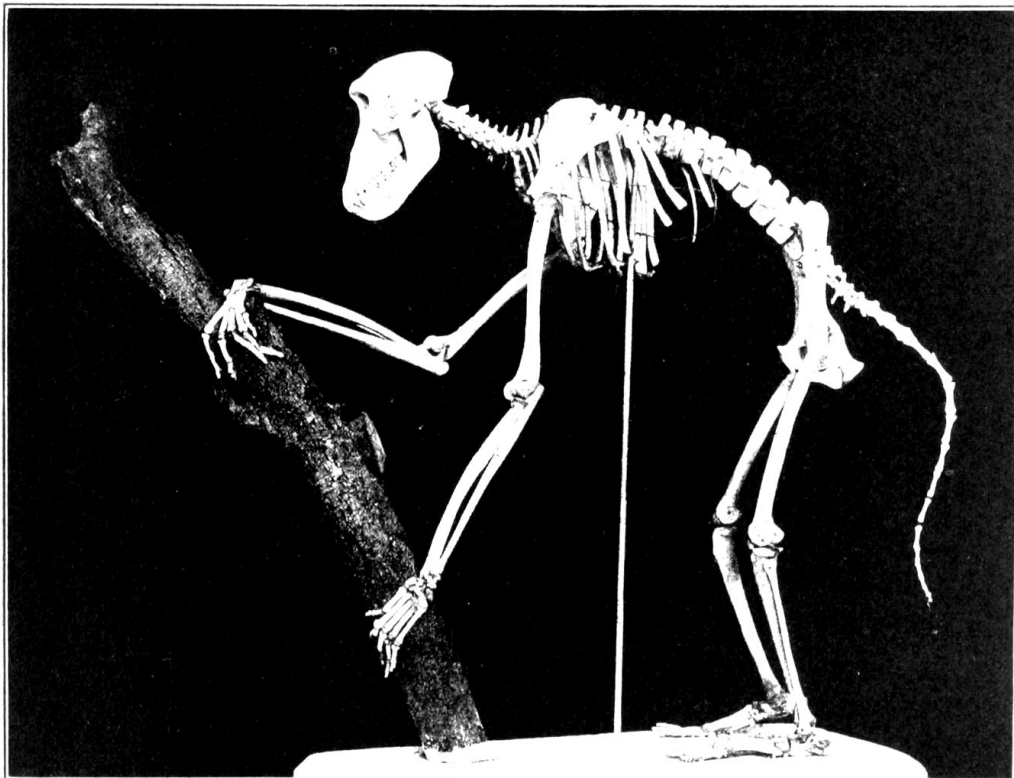
The complete skeleton of one of the Baboonfolk ( Papio papio ). All our bones are the same as yours, excepting the tail. Scientific fellows say you have lost yours because your ancestors ceased to use it. (From skeleton in Port Elizabeth Museum.)
