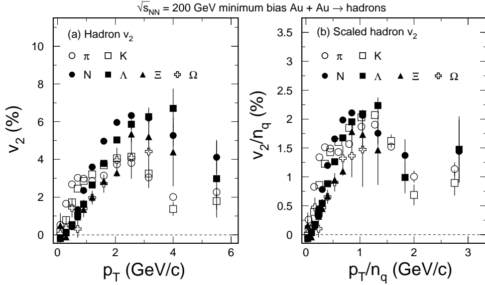
Figure 4. (a) Hadron v_2 from minimum bias Au+Au collisions at \sqrt{s_{NN}} = 200 GeV; (b) Scaled hadron v_2 results are shown. The n_q refers to the number of constituent quarks. Symbols represent results from the UrQMD (v2.2) model for various hadron species. At low p_T/n_q \leq 0.5 GeV/c, \pi does not follow the scaling perhaps caused by the resonance decay [14]. In higher p_T region, K meson seems to fall off the scaling curve due to the comparatively small hadronic cross sections in the model.
