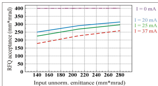
Figure 2: “High current” acceptance of the RFQ as a function of the input beam current and emittance.
