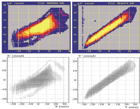
Figure 1: Measured horizontal and vertical beam emittances (top) and related particle distribution (bottom) generated for beam dynamics simulations.
