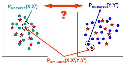
Figure 3: A coupling of the 2D particle distributions, generated from emittance measurements, to a 4D one.
