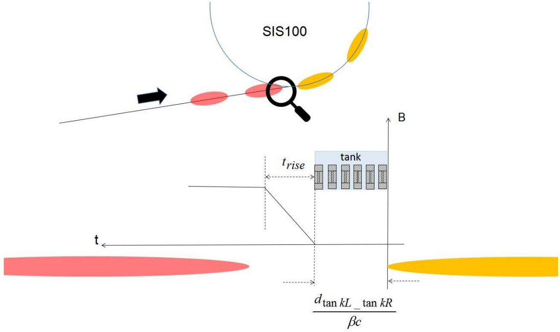
Figure 5.26: SIS100 injection kicker.
