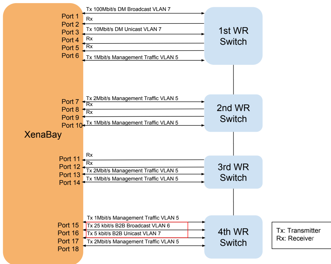
Figure 5.14: Connection between WR switches and the XenaBay of the test setup.
