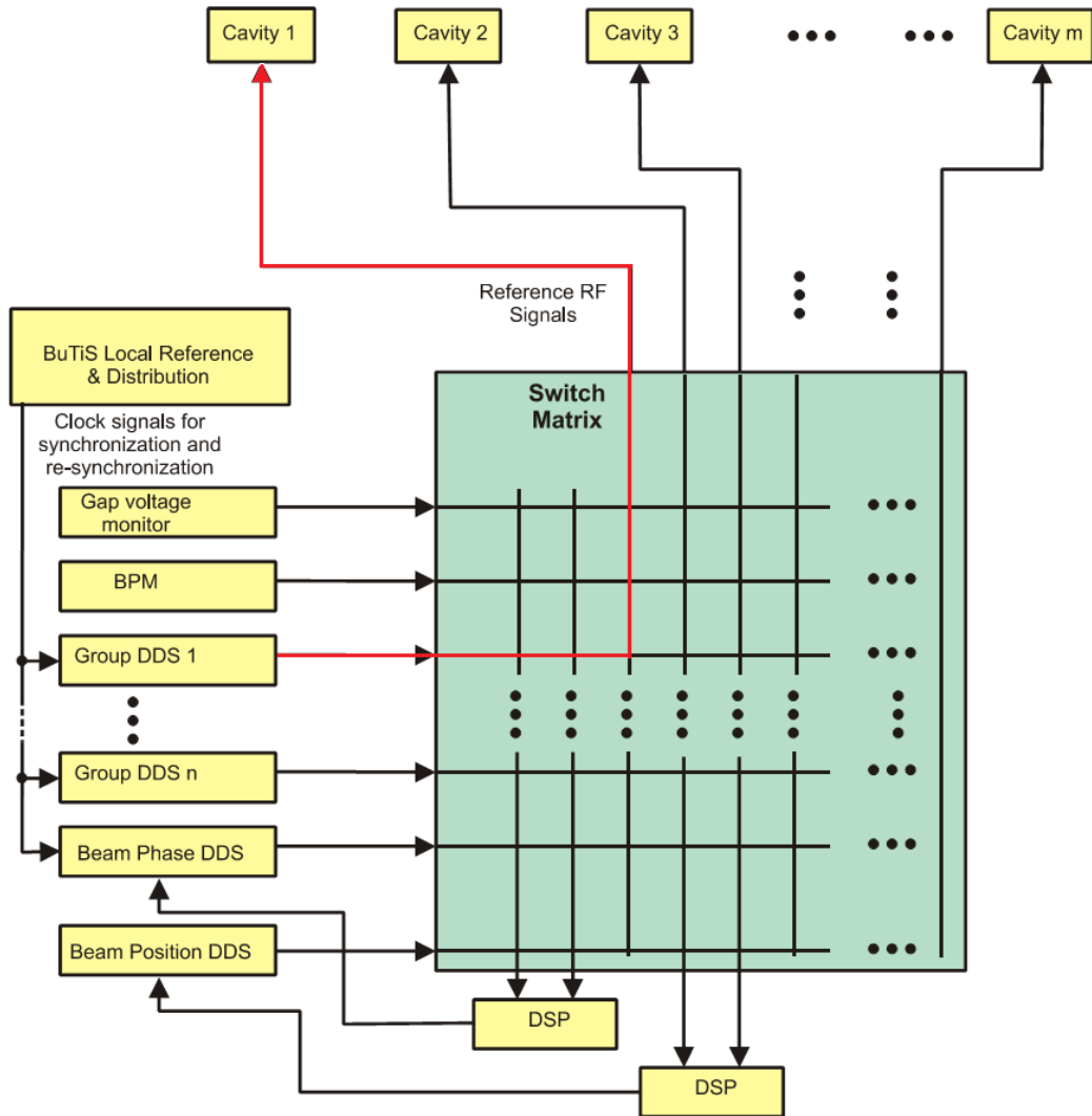
Figure 3.1: Reference rf signal distribution system
