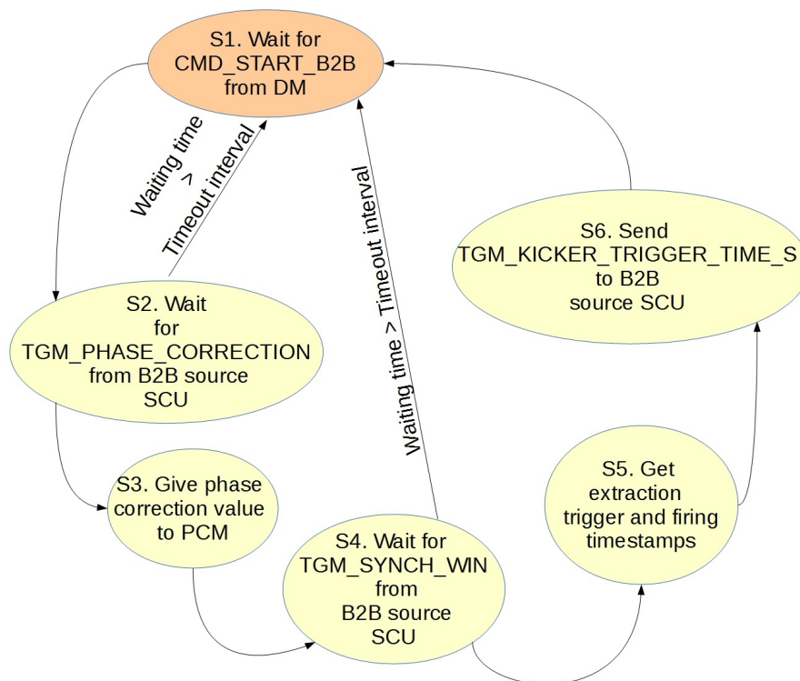
Figure 5.19: Flowchart of the B2B Trigger SCU.
