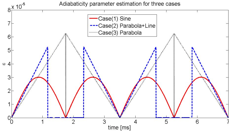
Figure 5.9: Adiabaticity parameter of three cases.
