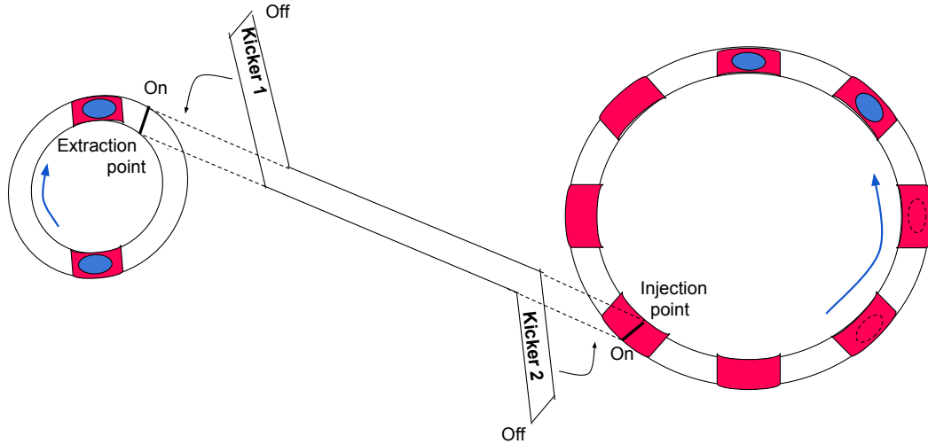
Figure 1.1: Illustration of a bunch-to-bucket transfer.
