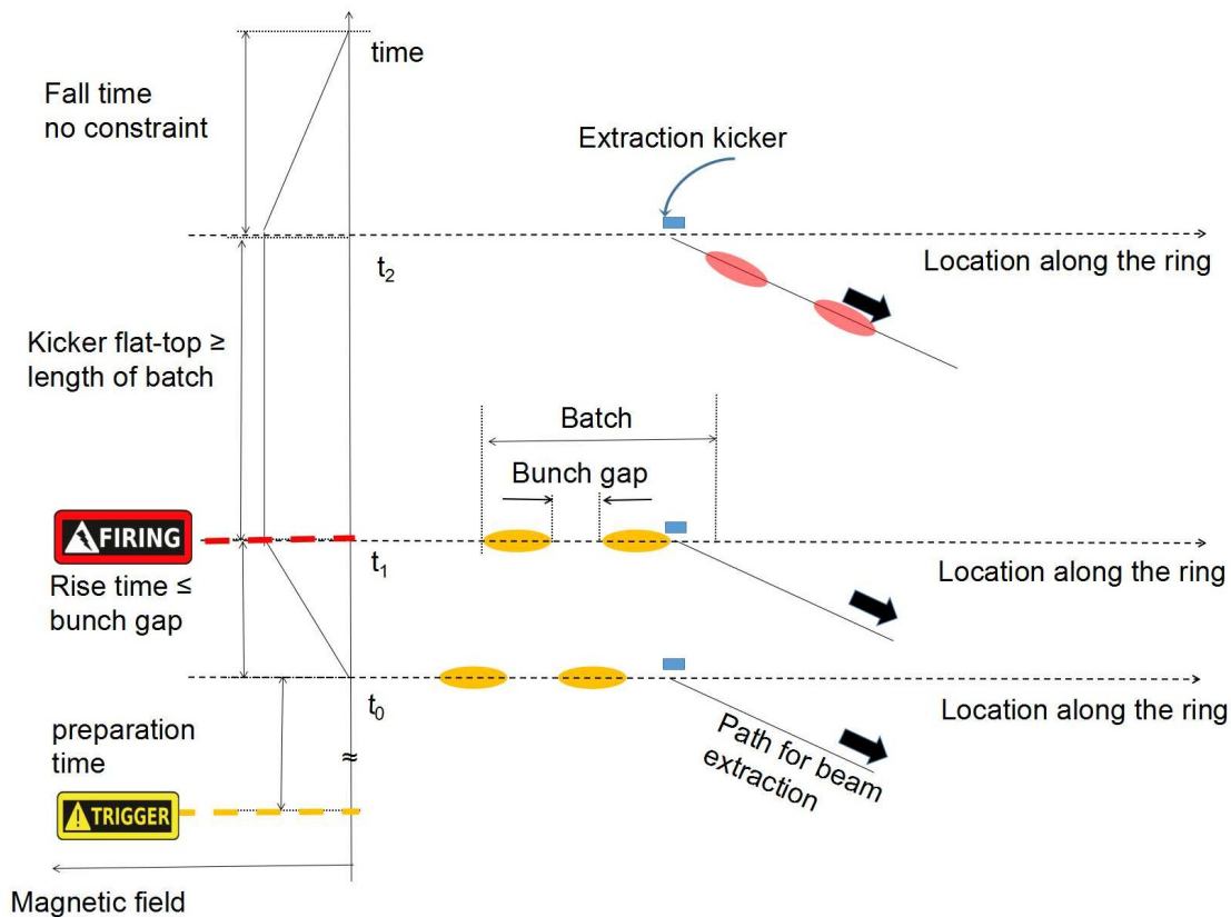
Figure 2.12: The rise time, kicker flat-top and fall time of an extraction kicker.
