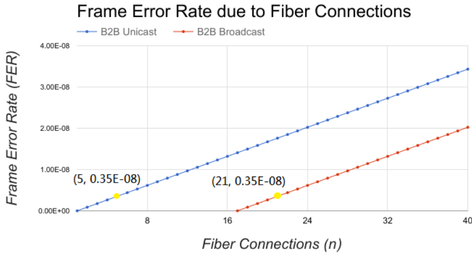
Figure 5.13: Relation between the FER and the fiber connections for B2B Unicast and Broadcast traffics.
