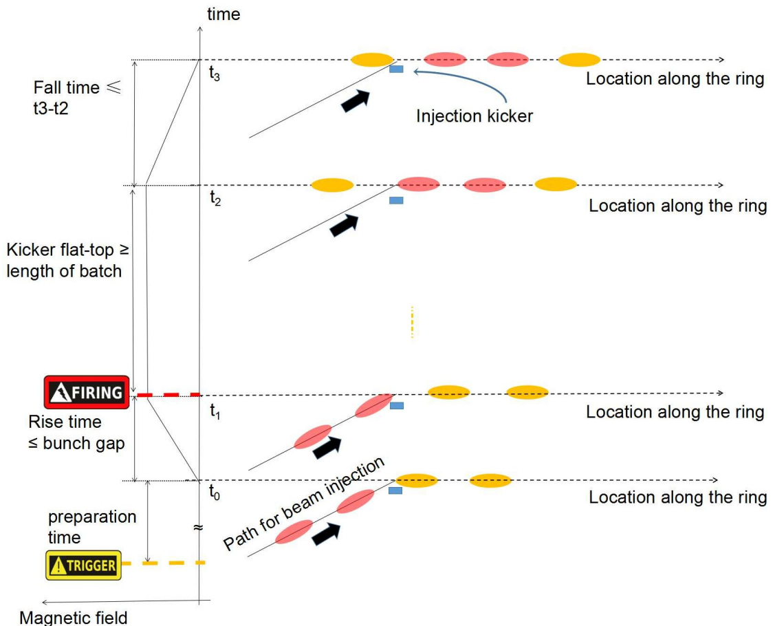
Figure 2.13: The rise time, kicker flat-top and fall time of an injection kicker for multiple batches injection.
