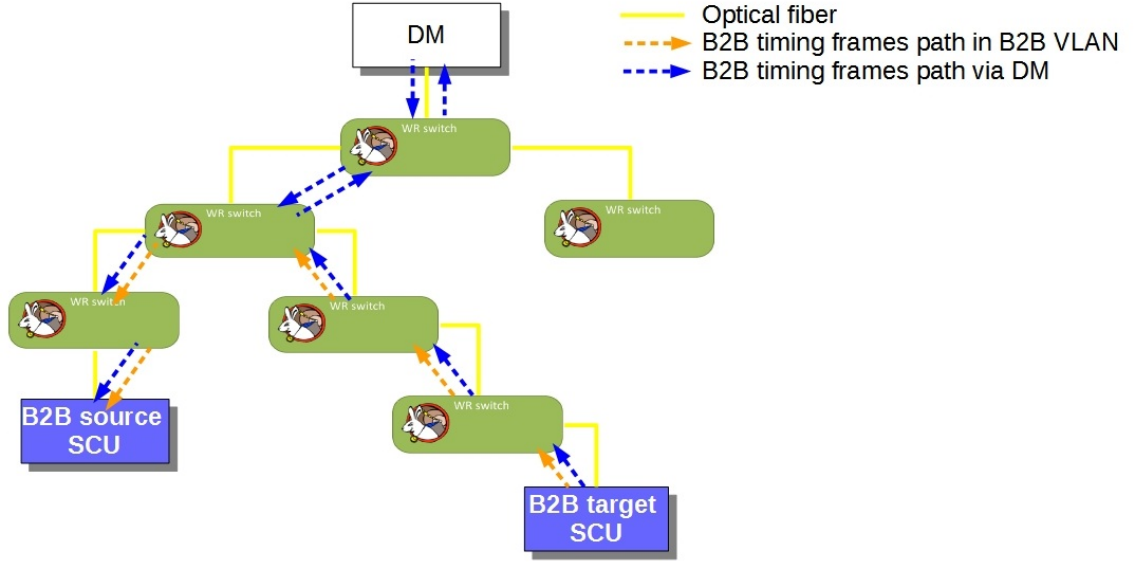
Figure 4.9: Example of the transfer path of the B2B timing frames on the WR network.
