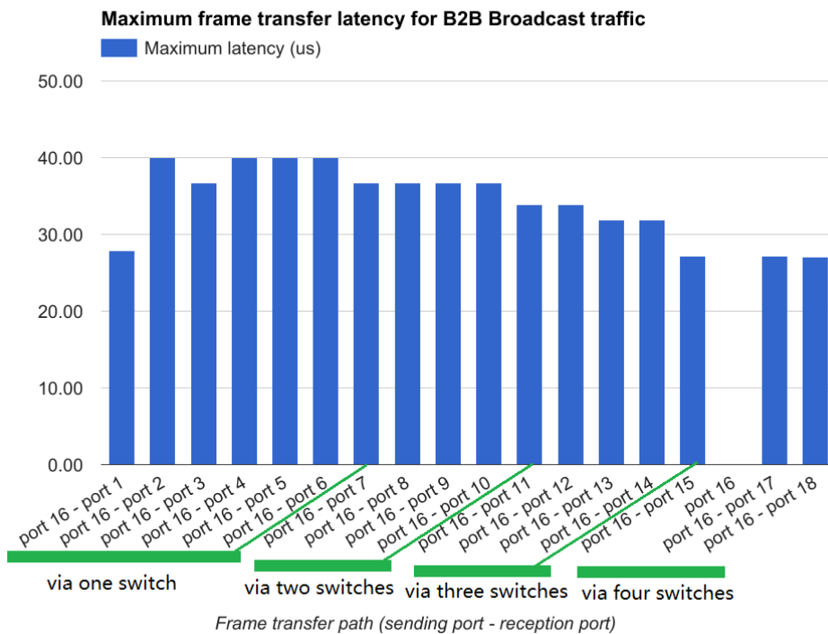
Figure 5.16: Maximum frame transfer latency for B2B Broadcast frames.
