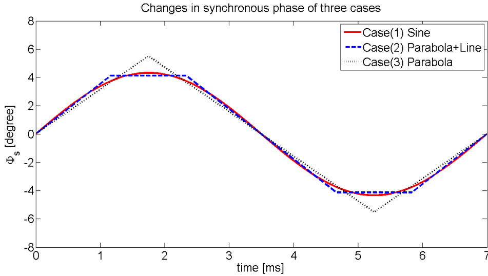
Figure 5.7: Changes in synchronous phase of three cases.
