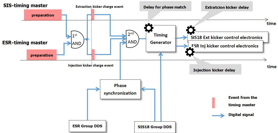
Figure 4.16: Current realization of the bunch-to-bucket transfer between the SIS18 and the ESR with the GSI control system.
