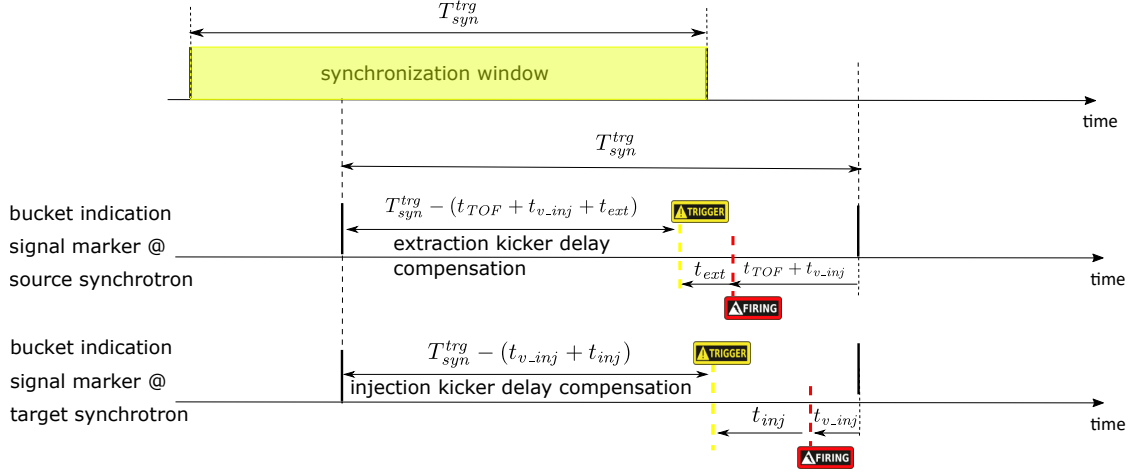
Figure 4.14: Illustration of the kicker delay compensation when the bucket indication signal has the frequency of f_{syn}^{trg} .
