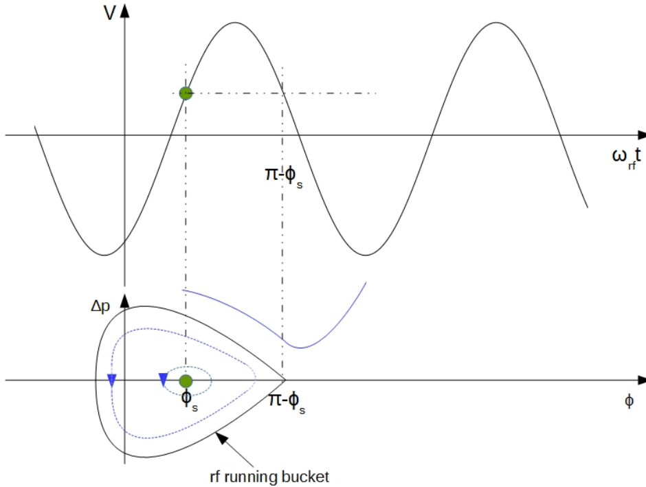
Figure 2.4: Running rf bucket.
