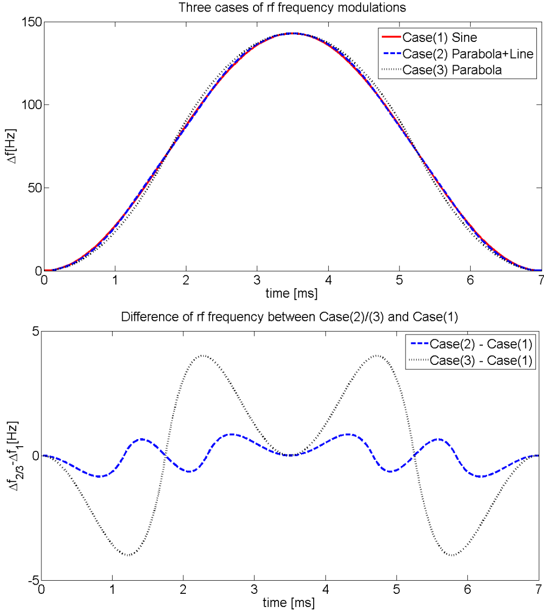
Figure 5.1: Examples of rf frequency modulations.
