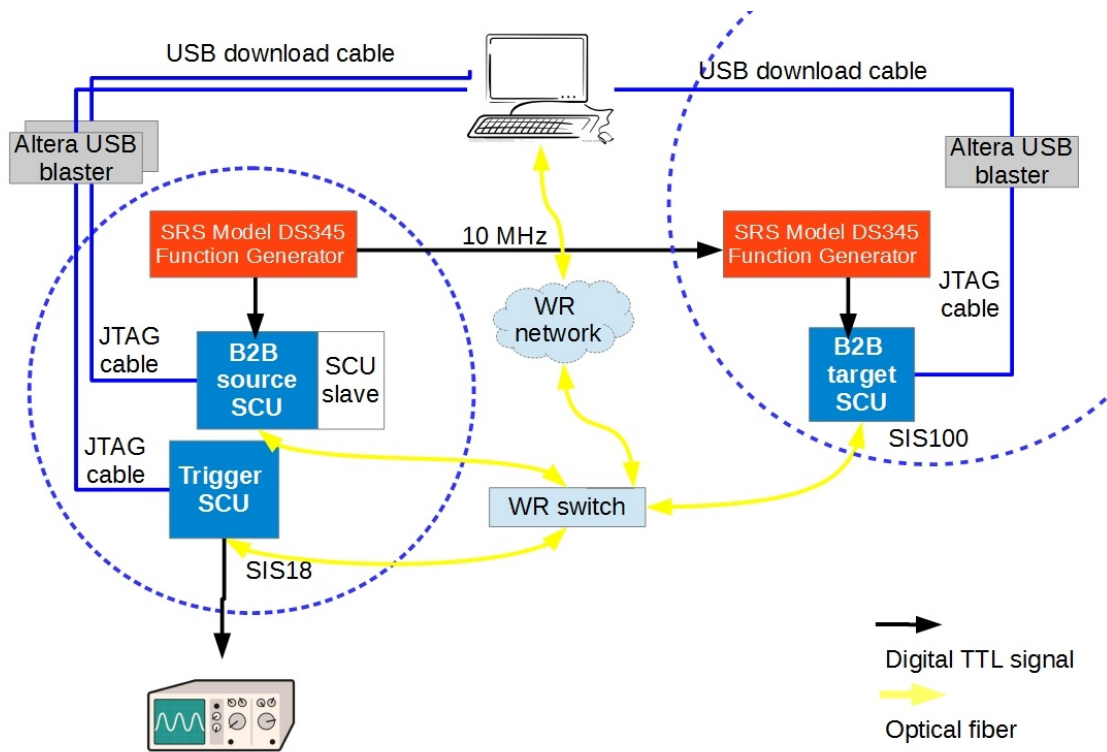
Figure 5.27: Schematic of the test setup.
