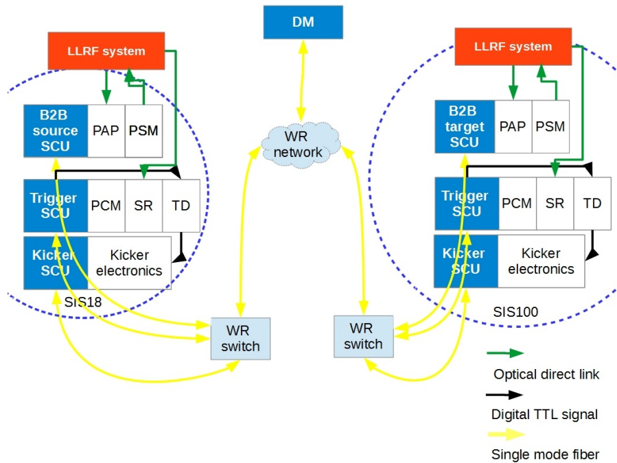
Figure 5.29: Schematic of the final setup.
