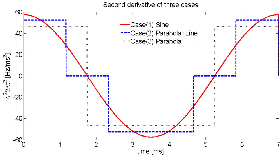
Figure 5.3: Second derivative of three cases.
