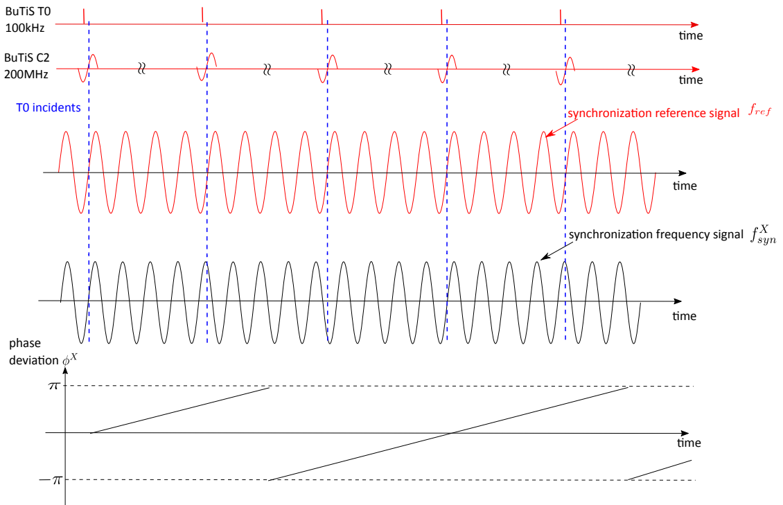
Figure 4.5: Phase deviation between the synchronization frequency and the synchronization reference signal.
