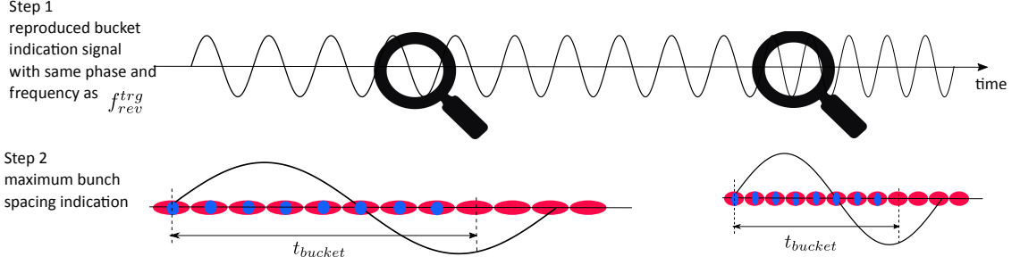
Figure 4.13: Realization of the maximum bunch spacing label for the emergency extraction.
