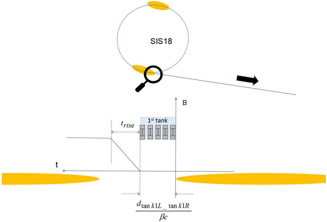
Figure 5.22: SIS18 extraction kicker.
