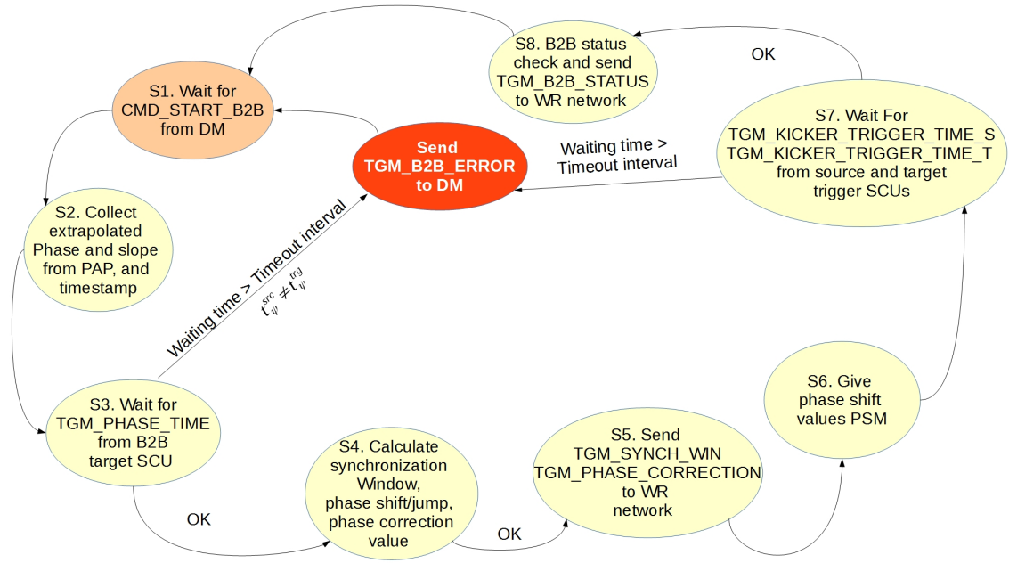
Figure 5.17: Flowchart of the B2B source SCU.
