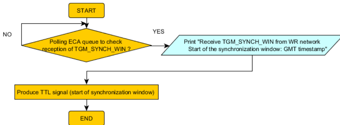
Figure 5.32: Flowchart of the firmware of the Trigger SCU for the test setup.
