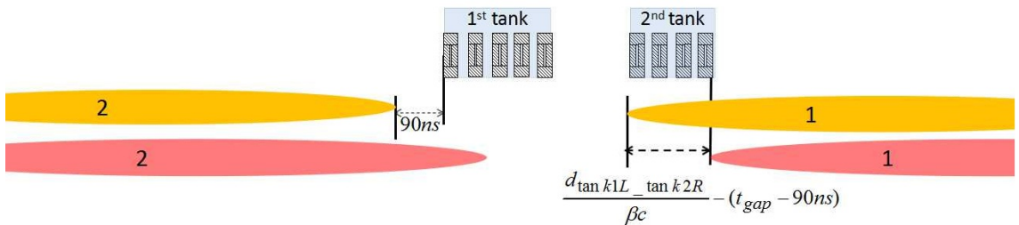
Figure 5.25: The minimum triggering delay between extraction kicker magnets in two SIS18 tanks.
