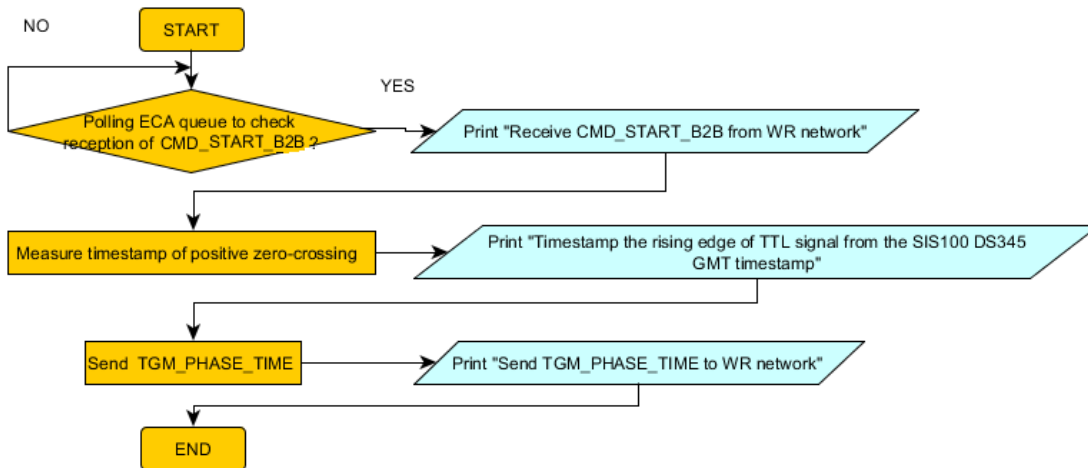
Figure 5.31: Flowchart of the firmware of the B2B target SCU for the test setup.
