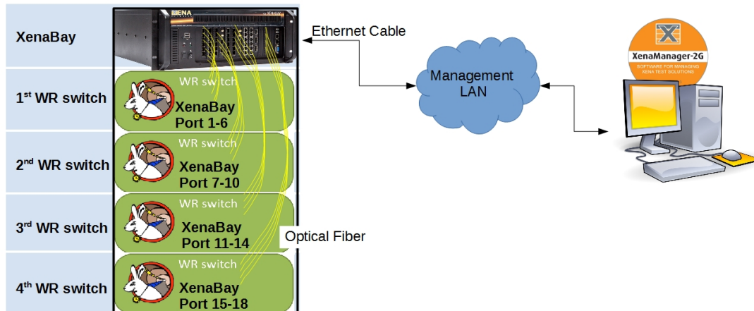
Figure 5.12: An overview of the Xena's Layer 2-3 test platform for the WR network.
