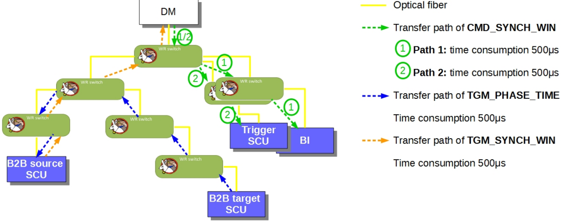
Figure 4.11: Transfer delay of the start of the synchronization window on the WR network.
