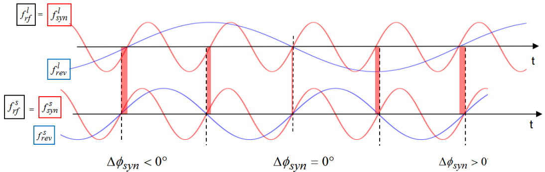
Figure 2.7: Periodically variable phase difference between two slightly different synchronization frequencies f_{syn}^l and f_{syn}^s when \kappa = 2 , \lambda = -0.003 , h_{rf}^s = 2 and h_{rf}^l = 4 .
