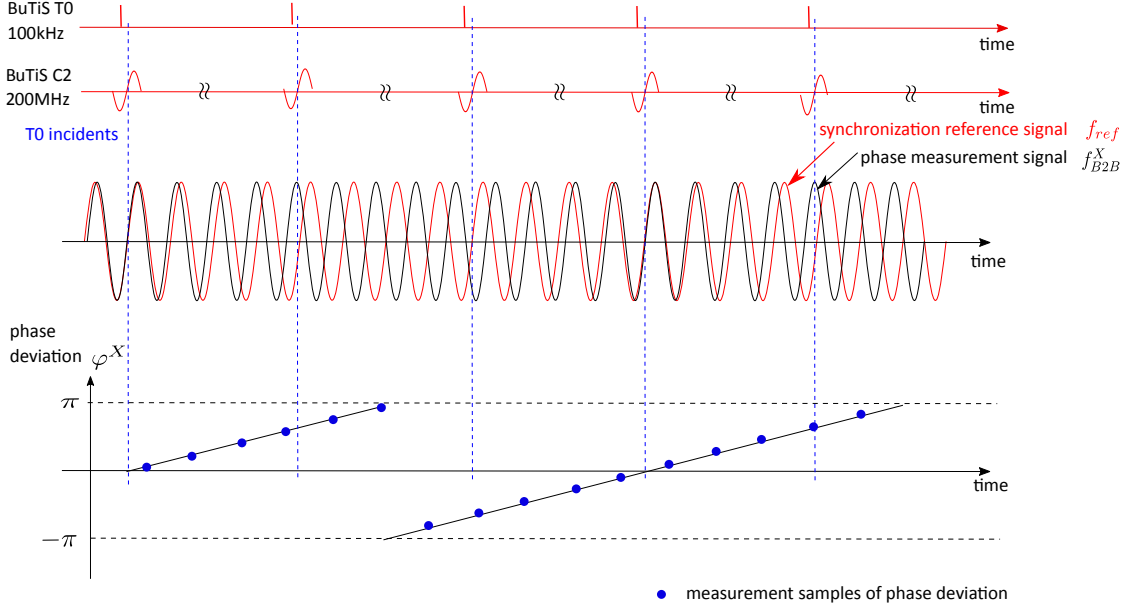
Figure 4.6: Realization of the phase deviation measurement at one accelerator.
