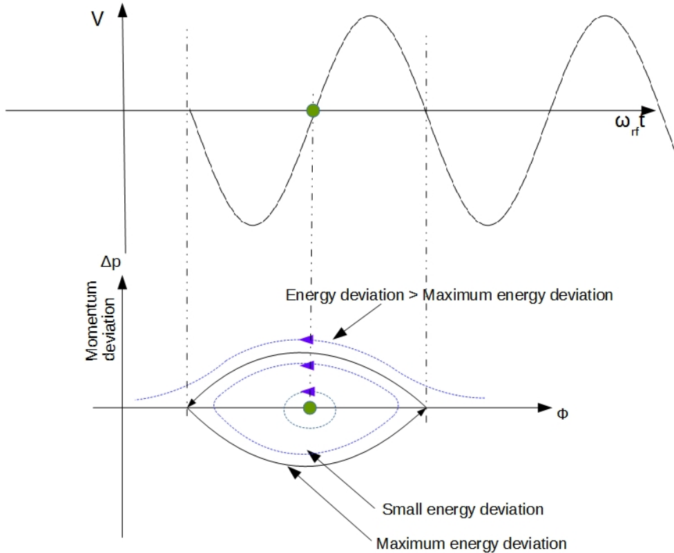
Figure 2.3: Stationary rf bucket.
