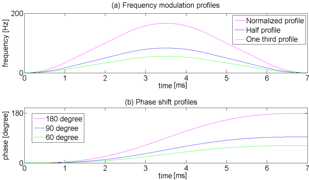
Figure 4.10: Example of normalized frequency and phase modulation profiles and the actual profiles.
