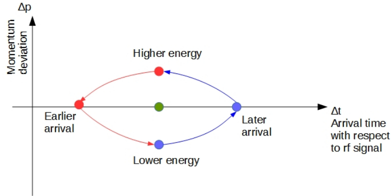
Figure 2.2: Longitudinal motion of asynchronous particles in the longitudinal phase space plane ( \eta > 0 ).
