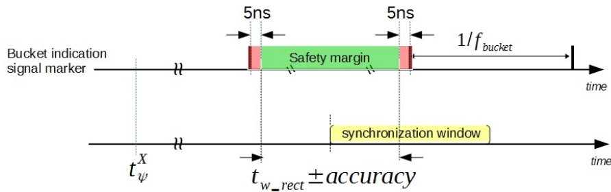
Figure 5.11: Illustration of the accuracy of the start of the synchronization window.
