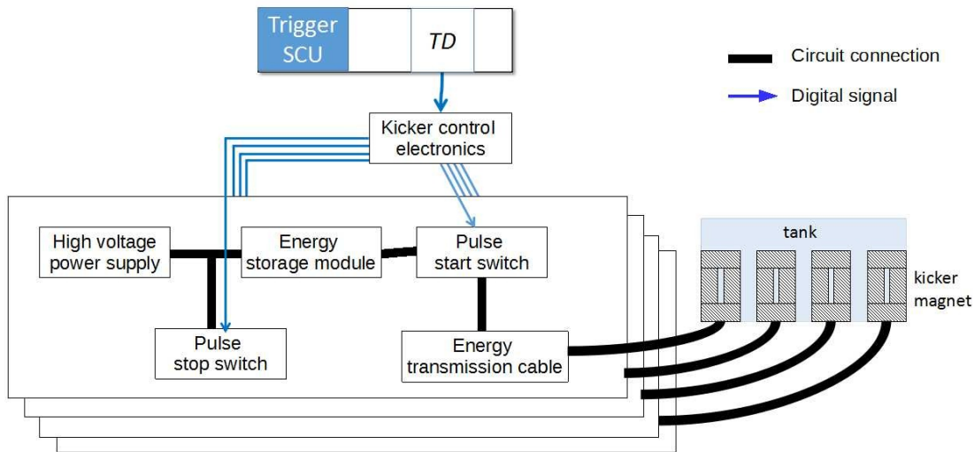
Figure 5.21: Schematic diagram of the controls and pulse electronics of the extraction kicker magnets in the SIS18 2 nd tank.
