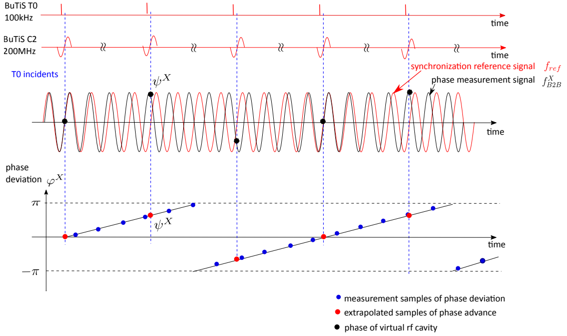
Figure 4.7: Realization of the phase advance extrapolation at one accelerator.
