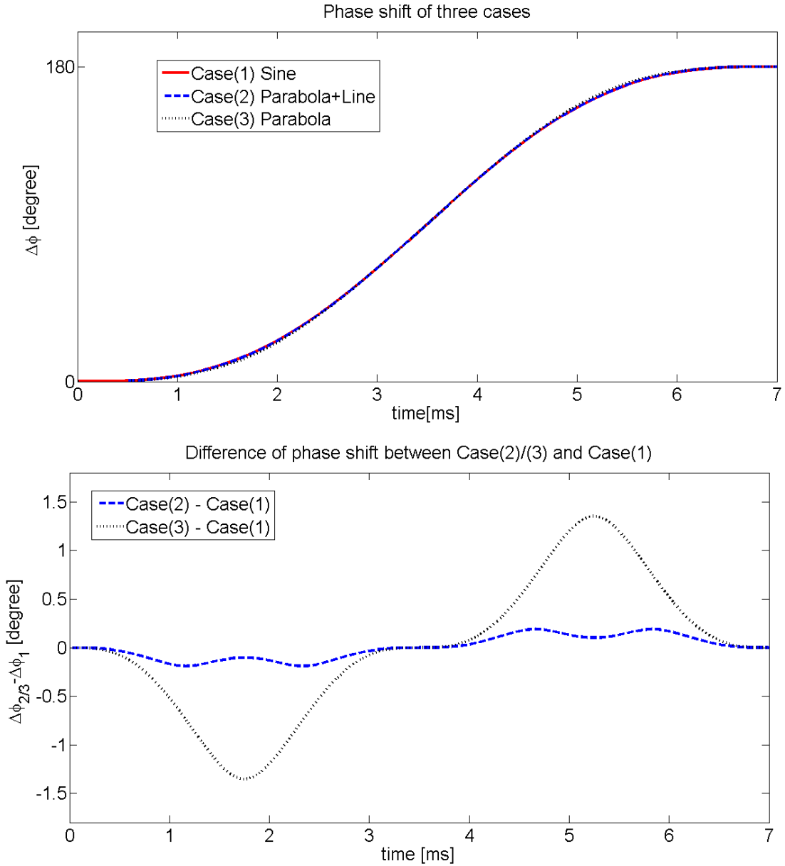
Figure 5.4: Phase shift modulation of three cases.
