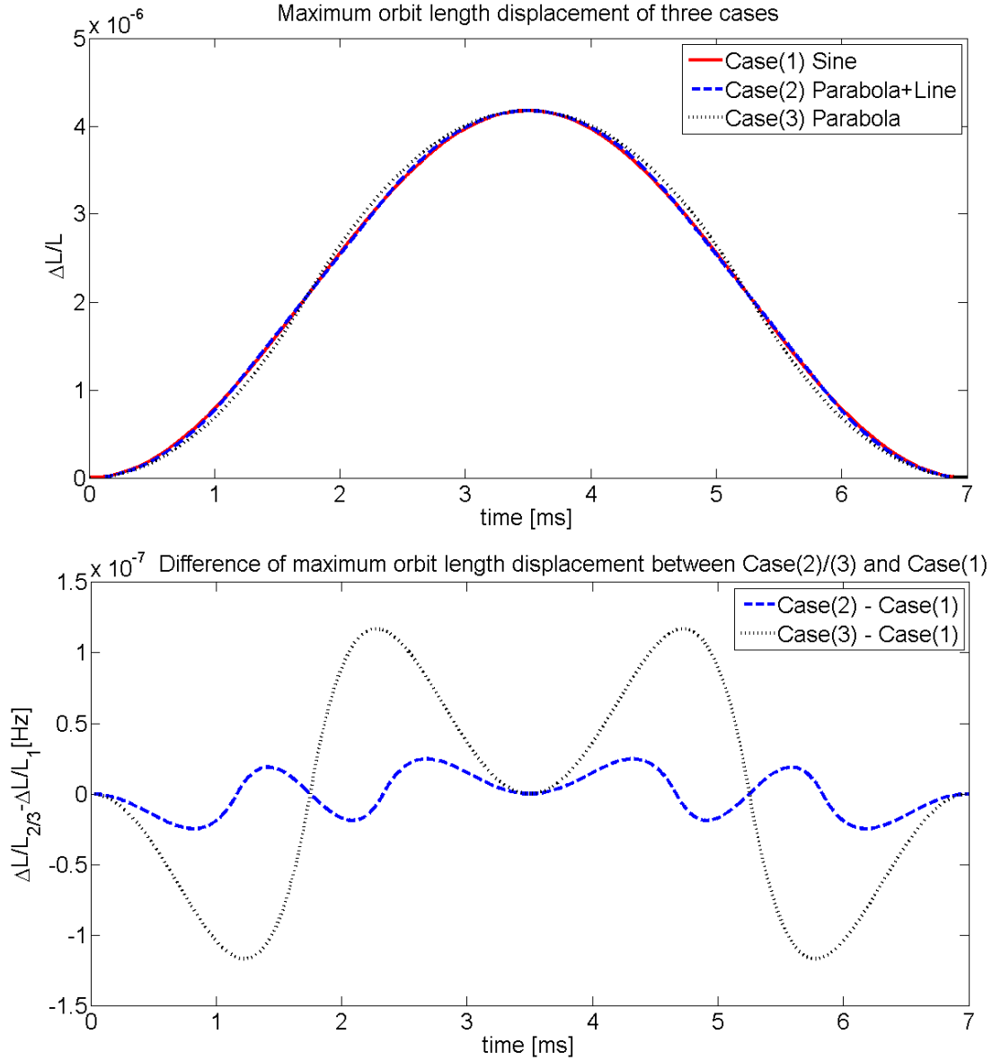
Figure 5.5: Orbit length displacement of three cases.
