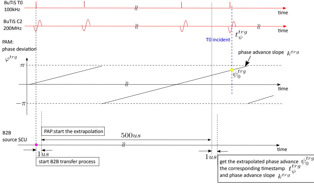
Figure 4.8: Synchronization of the extrapolated phase to the timestamp in one accelerator.
