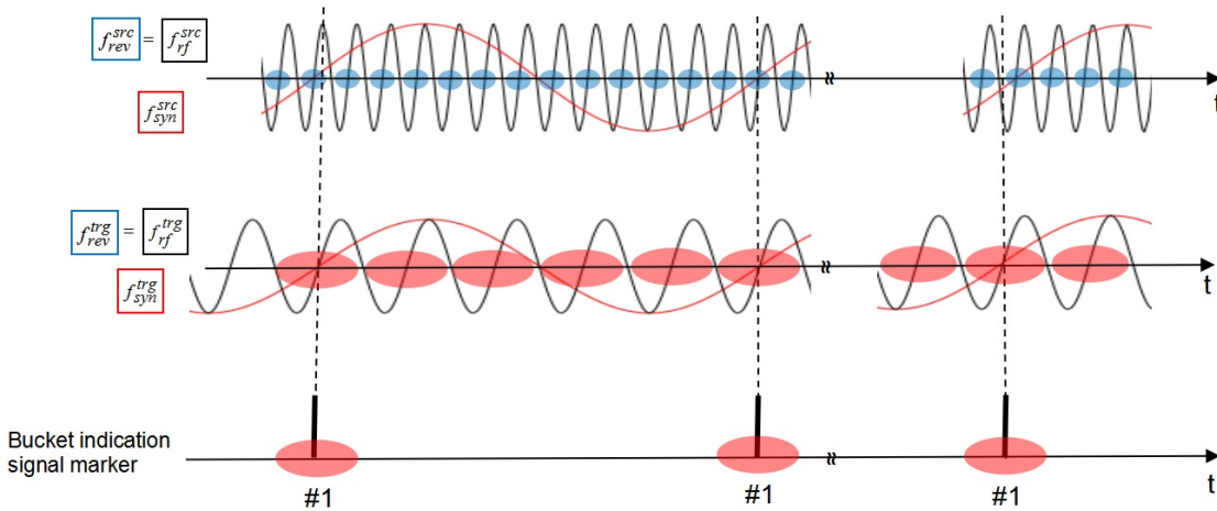
Figure 4.3: Frequency of the bucket indication signal equals to the synchronization frequency of the target accelerator.
