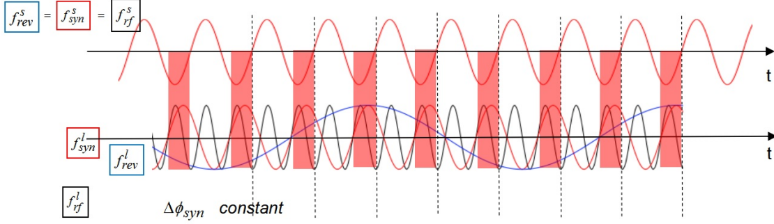
Figure 2.6: Constant phase difference between two synchronization frequencies f_{syn}^l and f_{syn}^s when \kappa = 5 , h_{rf}^s = 1 and h_{rf}^l = 10 .
