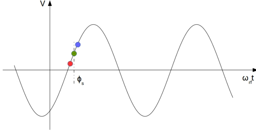
Figure 2.1: Longitudinal focusing of particles by an rf voltage ( \eta > 0 ).
