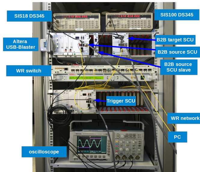
Figure 5.28: Front view of the test setup.
