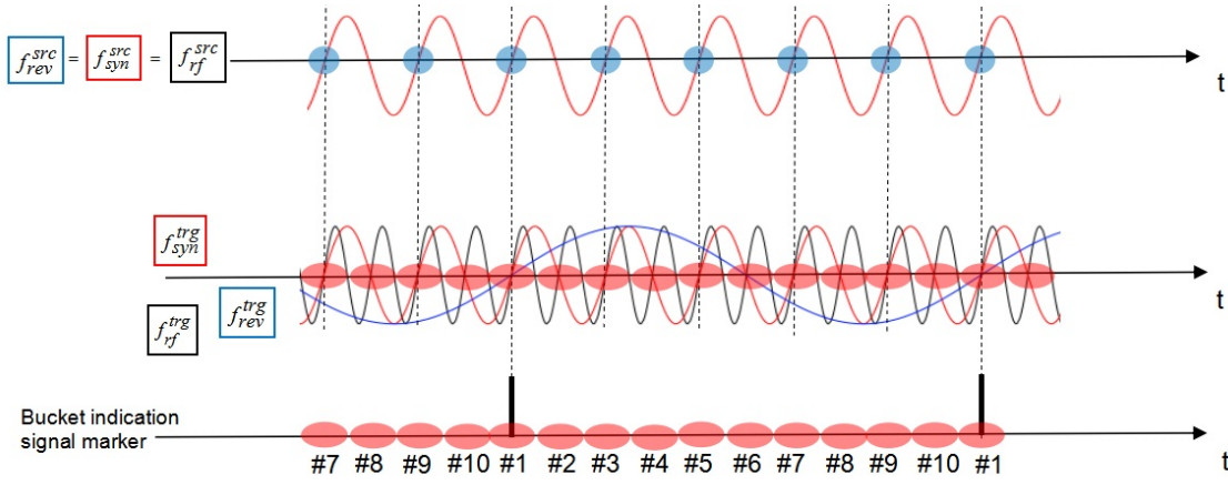
Figure 4.2: Frequency of the bucket indication signal equals to the revolution frequency of the target accelerator.
