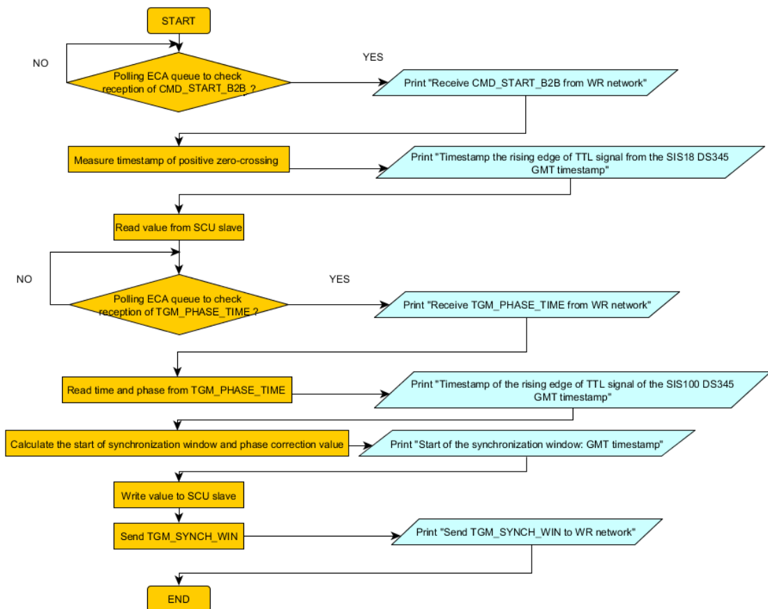
Figure 5.30: Flowchart of the firmware of the B2B source SCU for the test setup.
