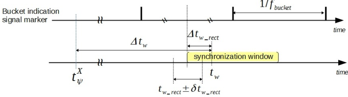
Figure 5.10: Illustration of the rectification for the start of the synchronization window.
