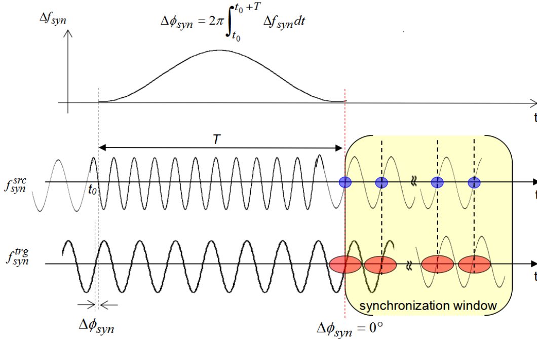
Figure 2.9: Example for the phase shift method with a sinusoidal rf frequency modulation.
