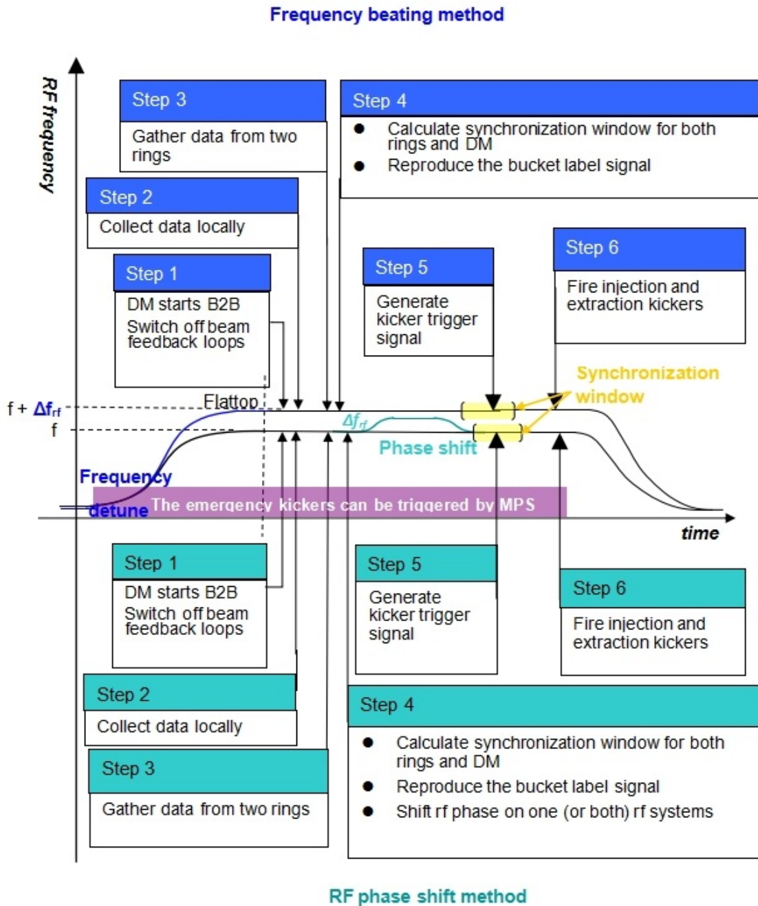
Figure 4.4: Procedure of the B2B transfer within one acceleration cycle.
