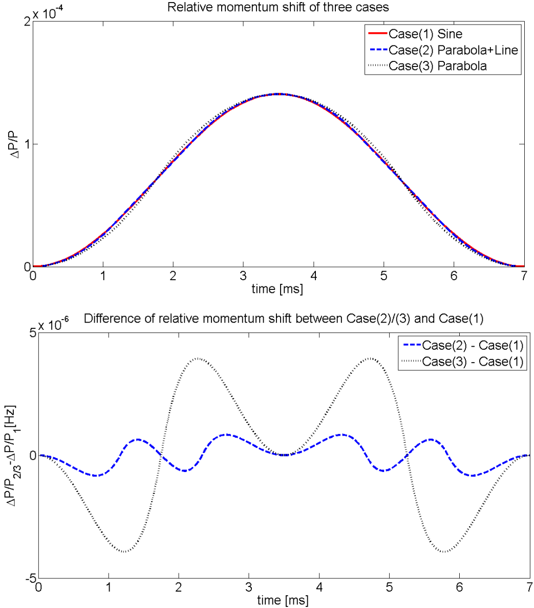
Figure 5.6: Relative momentum shift of three cases.
