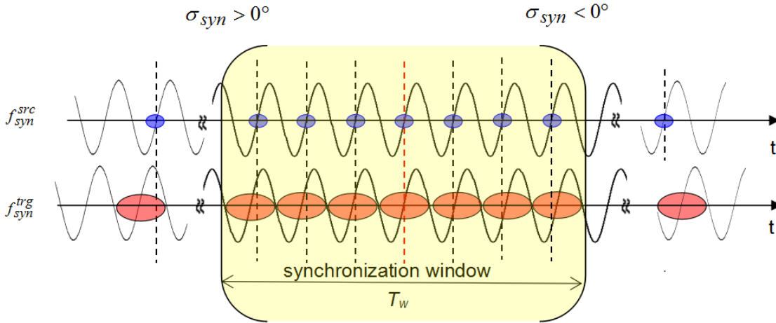
Figure 2.10: Illustration of the frequency beating method.
