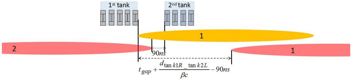
Figure 5.24: Maximum triggering delay between extraction kicker magnets in the SIS18 two tanks.
