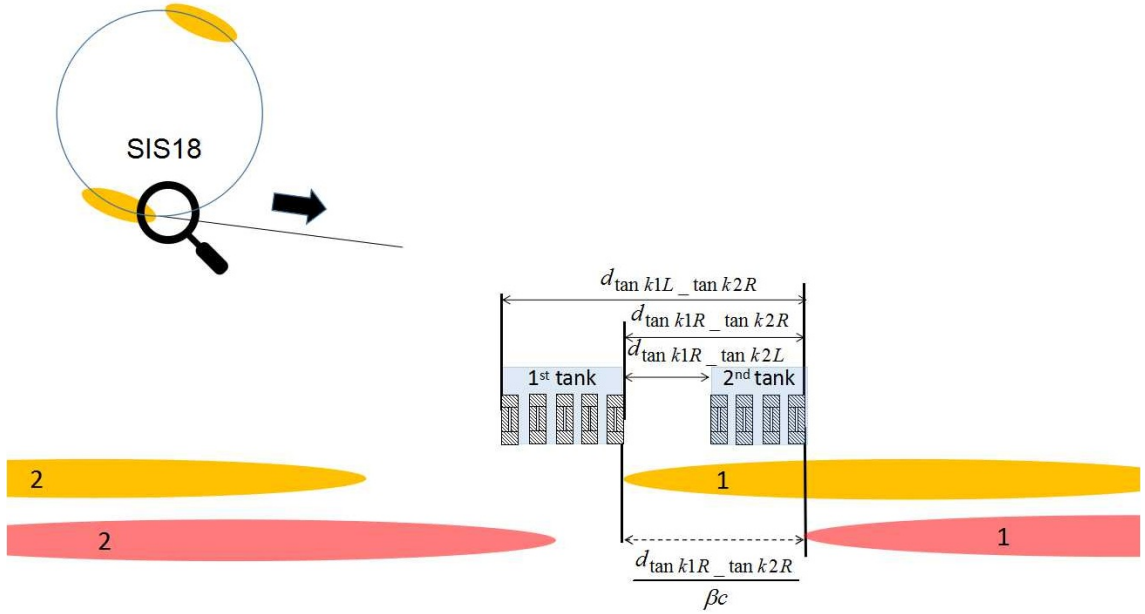
Figure 5.23: A possible triggering delay between extraction kicker magnets in the SIS18 two tanks.
