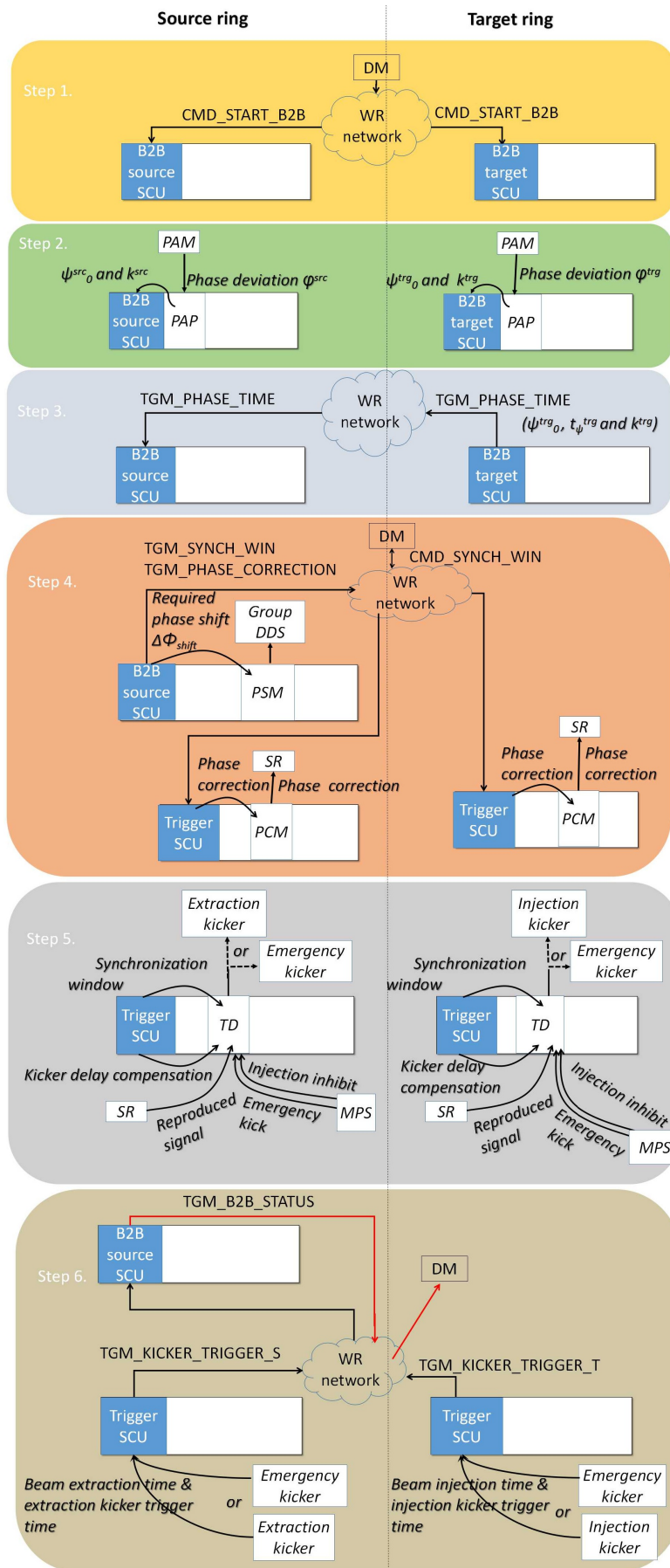
Figure 4.15: Data flow of the B2B transfer system
