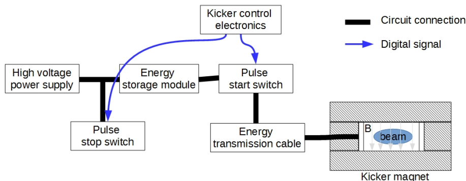
Figure 2.11: Schematic diagram of a kicker magnet.
