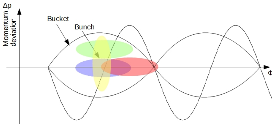
Figure 2.5: Bunch-to-Bucket injection with a phase, energy or voltage error.
