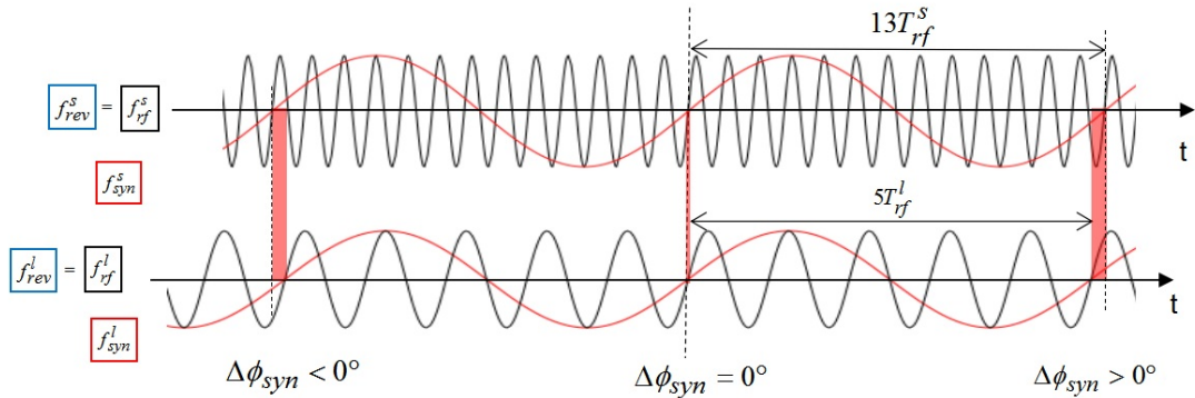
Figure 2.8: Periodically variable phase difference between two synchronization frequencies f_{syn}^l and f_{syn}^s when m = 26 , n = 10 , \lambda = -0.003 , h_{rf}^s = 1 and h_{rf}^l = 1 .
