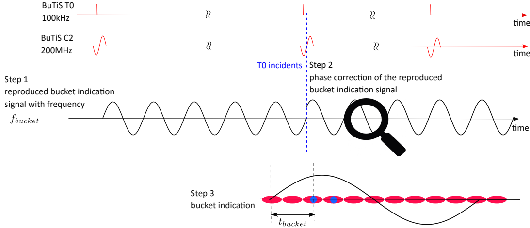
Figure 4.12: Realization of the bucket label for the normal extraction and injection.
