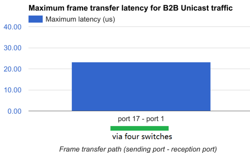
Figure 5.15: Maximum frame transfer latency for B2B Unicast frames.
