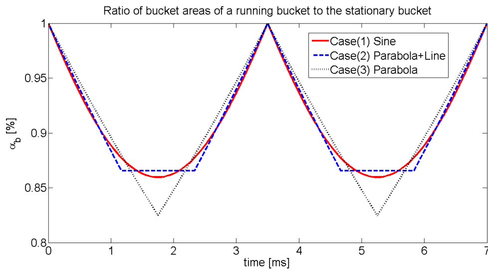
Figure 5.8: Ratio of bucket areas of a running bucket to the stationary bucket of three cases.
