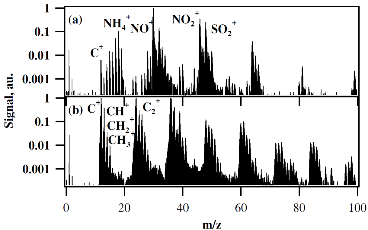
Supplemental Figure 1: Mass spectrum of an ammonium sulfate particle is shown in Panel (a). Individual ion peaks are specified in arbitrary units (au.) of detector signal versus mass to charge ratio ( m/z ). Mass spectrum of a polystyrene latex sphere is shown in Panel (b) using the same convention. Note the different peaks allow an unambiguous differentiation of these particle types.
