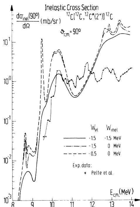
FIG. 6. The 90^\circ differential cross section for the excitation of the first 2^+ state in the ^{12}\text{C} - ^{12}\text{C} scattering. The experimental data are represented by the crosses and taken from Ref. 34. The theoretical cross sections are computed with the same choices of parameters as used for the elastic excitation function in Fig. 5. The following strengths W_0 of the imaginary potential are chosen: (i) W_{e1} = W_{i1} = -1.5 MeV (solid line); (ii) W_{e1} = -1.5 MeV, W_{i1} = 0 MeV (dotted-dashed line); (iii) W_{e1} = -0.5 MeV, W_{i1} = 0 MeV (dashed line).
