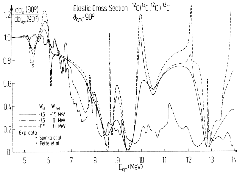
FIG. 5. The elastic excitation function (d\sigma_{el}/d\Omega)/(d\sigma_{Mott}/d\Omega) at \theta_{c.m.}=90^\circ for ^{12}\text{C}-^{12}\text{C} scattering. The experimental data are represented by the crosses and are taken from Ref. 7 for E_{c.m.} \leq 7.5 MeV and from Ref. 34 for E_{c.m.} \geq 6.5 MeV. The theoretical excitation functions are computed with the type 2 coupling potential with \alpha=-60 MeV and 2R=8.5 fm for various strengths W_0 of the imaginary potential. The following choices are made: (i) W_0=-1.5 MeV in the elastic and inelastic channels (solid line); (ii) W_0=W_{el}=-1.5 MeV in the elastic and W_0=W_{inel}=0 in the inelastic channels (dotted-dashed line); (iii) W_{el}=-0.5 and W_{inel}=0 (dashed line).
