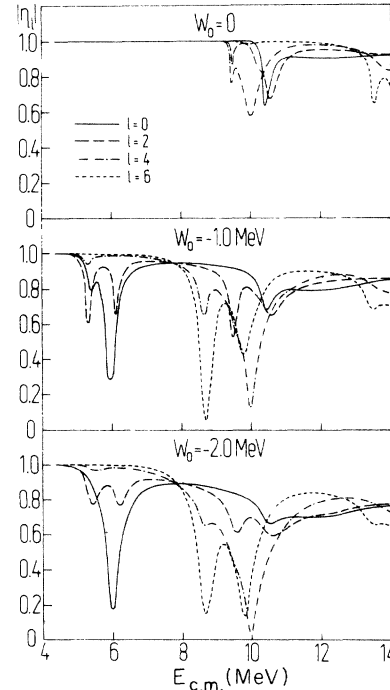
FIG. 9. Dependence of the reflection coefficients |\eta_l| on the strength of the imaginary potential W_0 = W_{e1} = W_{inel} which is chosen the same in all channels. The coupling potential is of type 2 with \alpha = -60 MeV and 2R = 8.5 fm. In the case of W_0 = 0 the absorption in the reflection coefficient is solely caused by the coupling of the first 2^+ state in ^{12}\text{C} .
