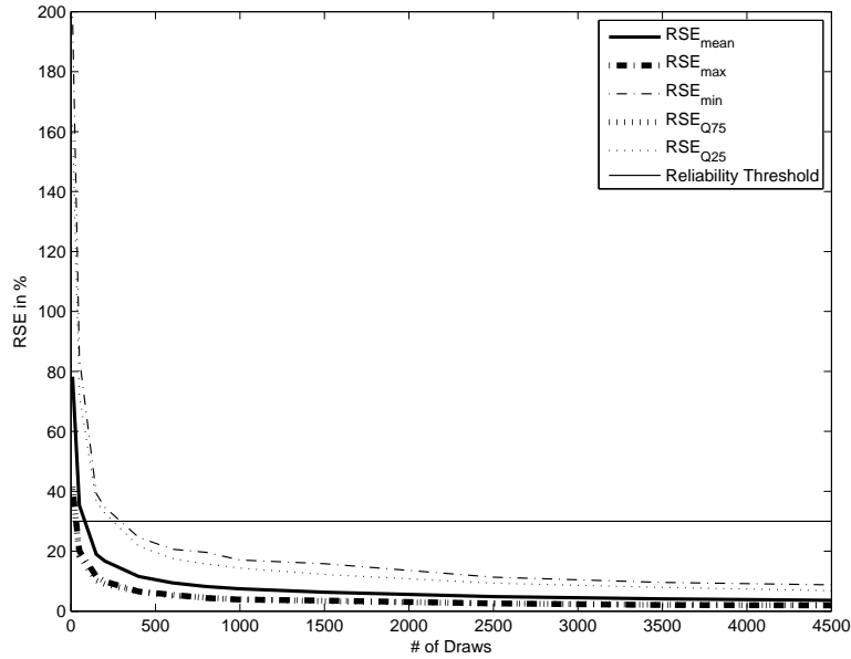
Figure 17: Relative Standard Errors at Various Sample Sizes
