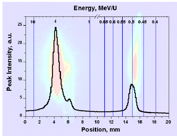
Figure 3: Typical energy spectrum of the ions after IH. Original picture from CCD camera is shown in false-colour-mode together with its projection to the X-axis.
