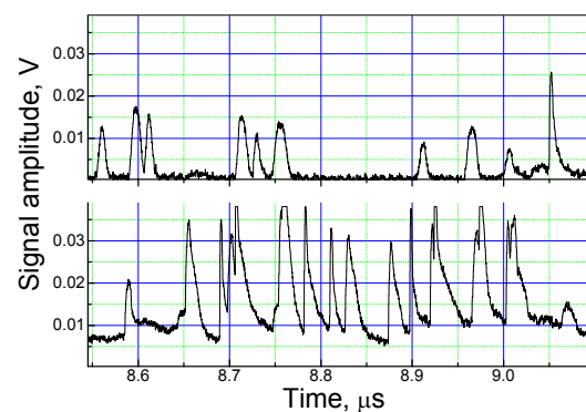
Figure 2: Signal from the single crystal diamond detector. In the upper graph the RF field of the IH was switched on; in the lower graph the IH RF was switched off.
