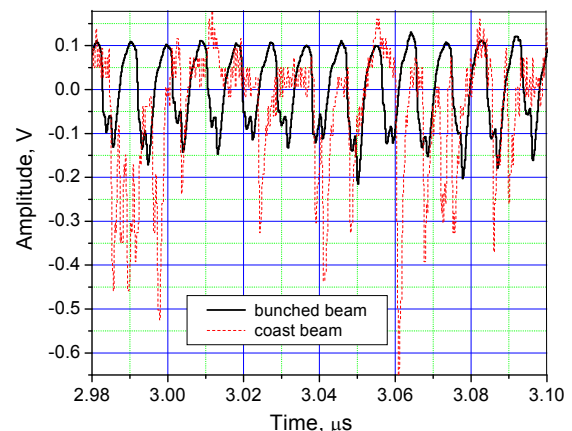
Figure 1: Signal from the polycrystalline diamond detector. The solid line shows the bunched beam, the dashed line the beam without bunching.
