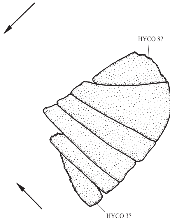
Fig. 10. Joinvillichthys lindstroemi (Davis, 1890). Hypochordal elements of sample CLC S-138. The arrows indicate the position of the most external dorsal and ventral procurent ray of the caudal fin.
