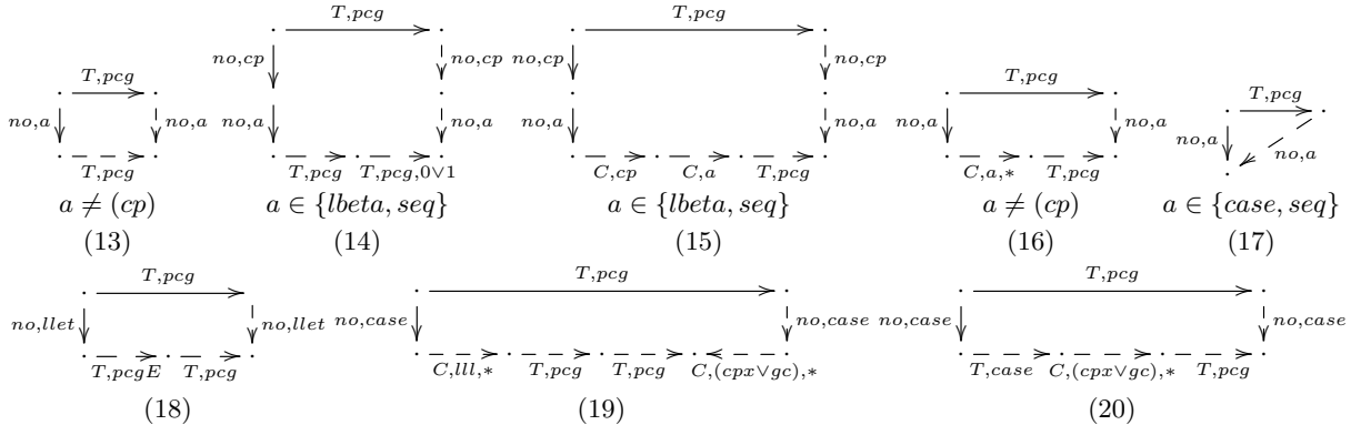
Fig. 8: Forking-diagrams for (pcg)
