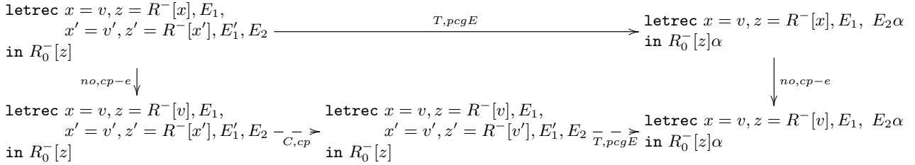
(c) Typical case for diagram (8)
