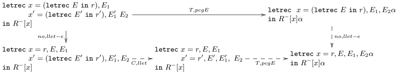
(b) Typical case for diagram (7)
