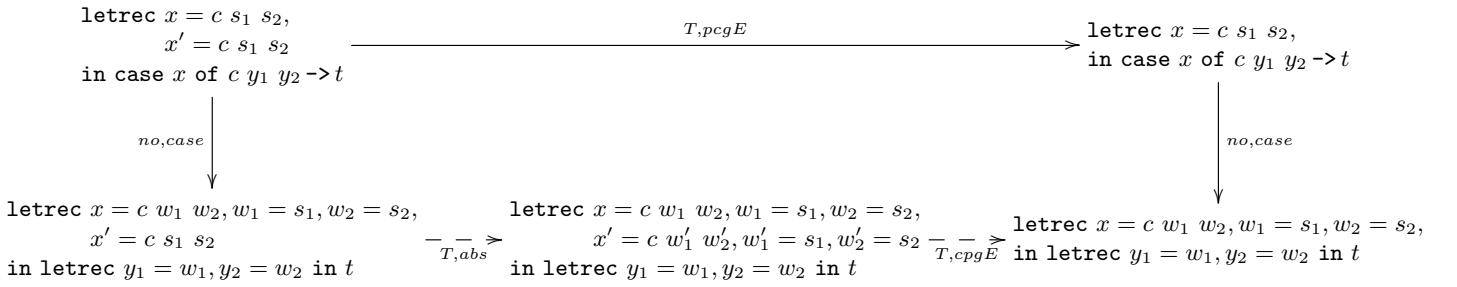
(b) Typical case for diagram (11)
