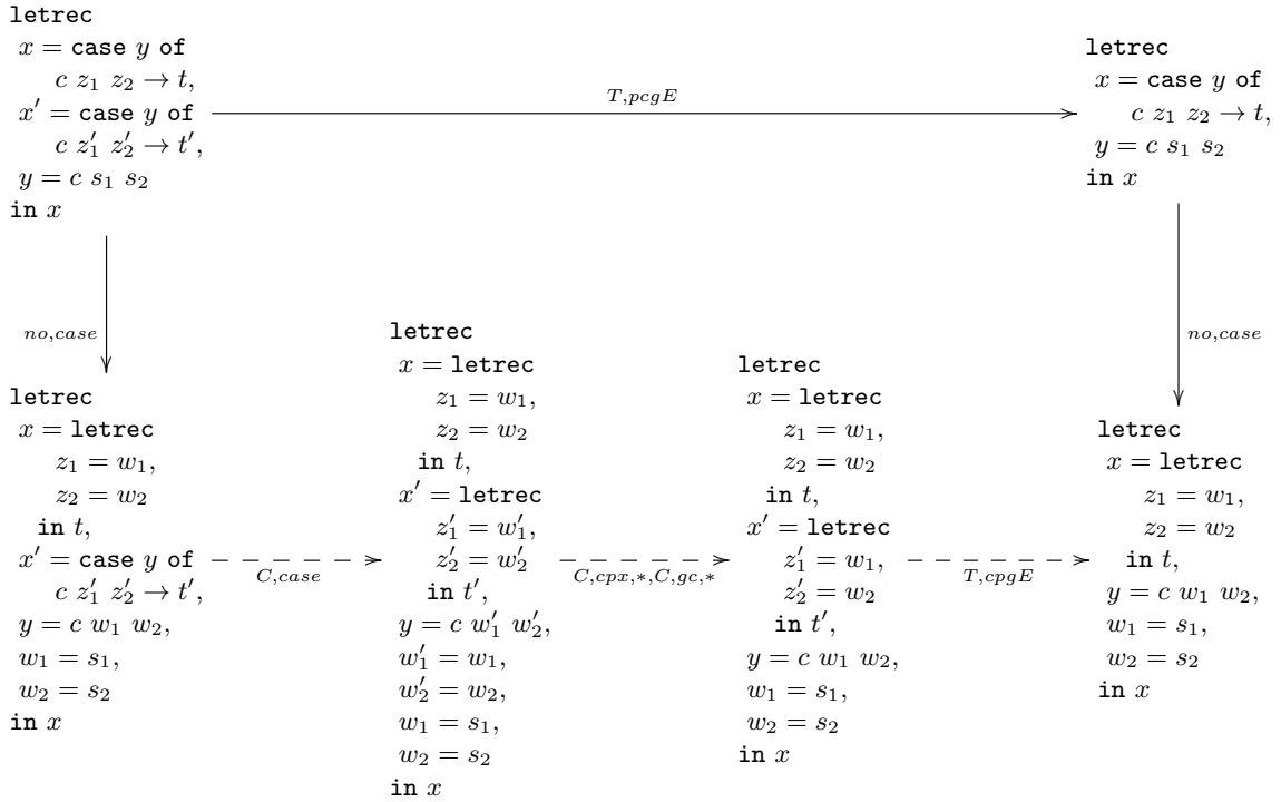
(c) Typical case for diagram (12)
