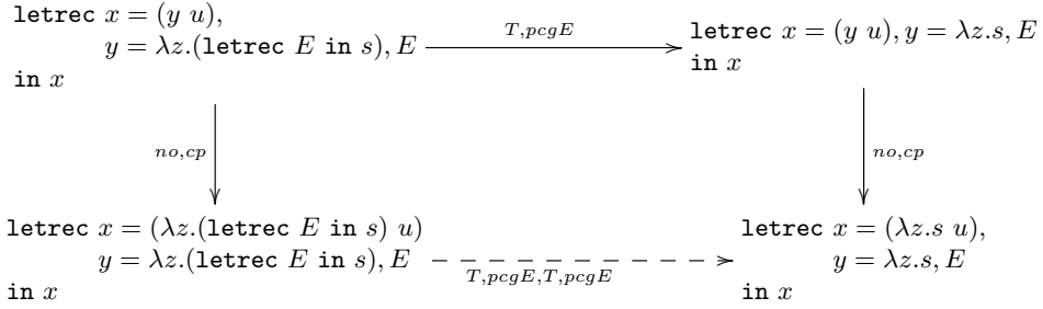
(a) Typical case for diagram (10)
