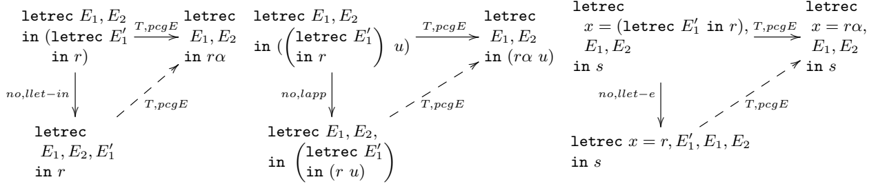
(a) Typical cases for diagram (6)
