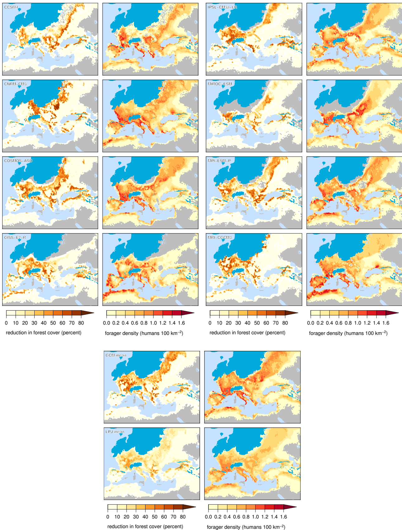
Fig. S2. Simulated forager population density and associated reduction in tree cover. The reduction in tree cover between a simulation with and without human burning ( left panels ) and the associated simulated forager population density ( right panels ). Results are shown for LPJ-LMfire runs driven by each of the eight GCM climate simulations, and the multi-model ensemble means.
