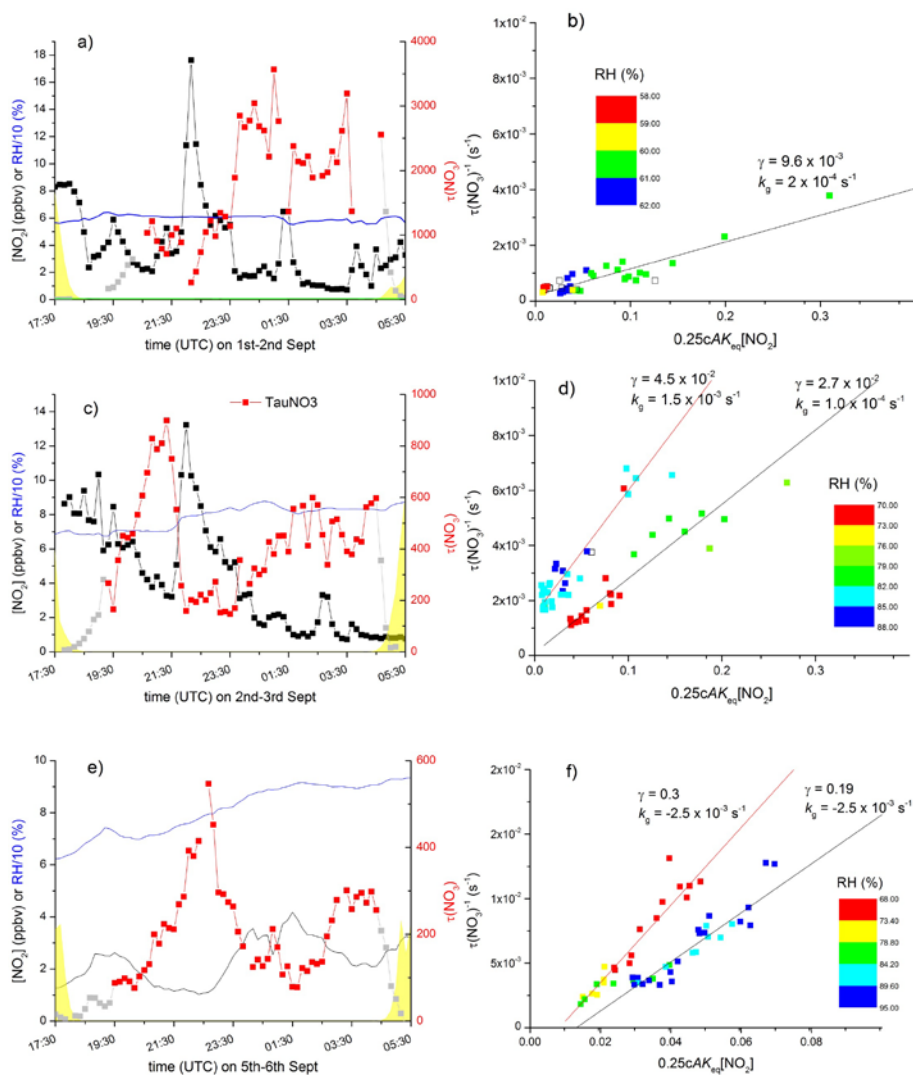
Fig. 9. Derivation of \gamma via analysis of \text{NO}_3 steady-state lifetime variation with \text{NO}_2 . The grey \tau(\text{NO}_3) data points were not considered in the analysis as \text{NO}_3 will not always be in steady state in the first hours after sunset or during sunrise.
