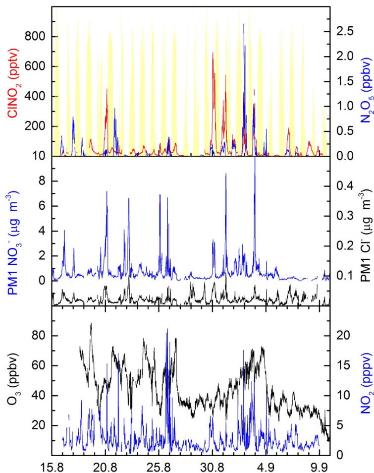
Fig. 3. Time series of \text{ClNO}_2 and its precursor, \text{N}_2\text{O}_5 . Global radiation (yellow) is plotted to separate day-night periods, and to indicate the day-to-day, relative photochemical activity. The precursors to \text{N}_2\text{O}_5 ( \text{NO}_2 and \text{O}_3 ) are shown as are the AMS measurement of particulate nitrate (as in Fig. 2) and chloride.
