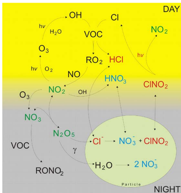
Fig. 1. Gas- and aqueous-phase chemical processes forming \text{ClNO}_2 and particulate nitrate indicating the role of \text{ClNO}_2 in modifying the effect of \text{N}_2\text{O}_5 uptake on the chemical lifetime of \text{NO}_x and photochemical \text{RO}_2 generation.
