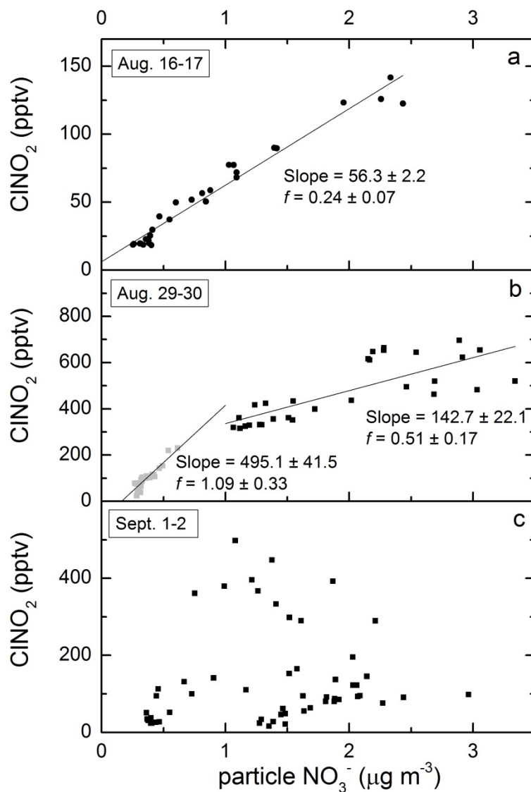
Fig. 5. Plots of \text{CINO}_2 versus \text{NO}_3^- for three different campaign nights. The slopes are converted to a fractional formation of \text{CINO}_2 ( f ) via Eq 5.
