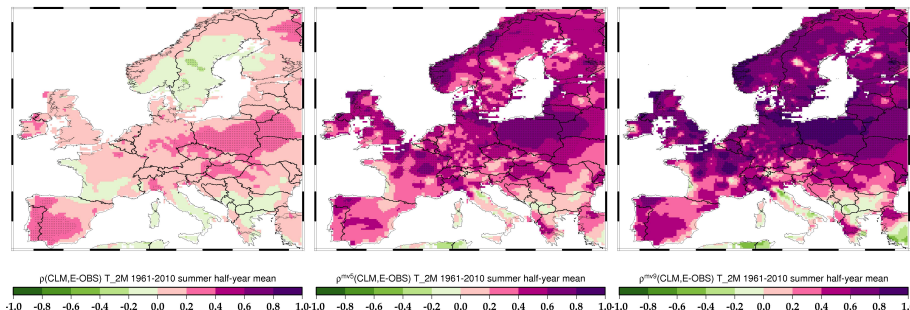
Fig. 4. Here, the summer half-year temperature correlation between E-OBS anomalies and the CCLM ensemble mean anomalies is shown. Significant correlation coefficients are represented by stippling. Left: correlation coefficients for the original unfiltered data are shown. Middle: The application of a 5 yr moving average filter is beneficial and increases the correlation coefficient. Right: A 9 yr moving average filter further increases the correlation in northern Europe, but is more or less ineffective in southern Europe.
