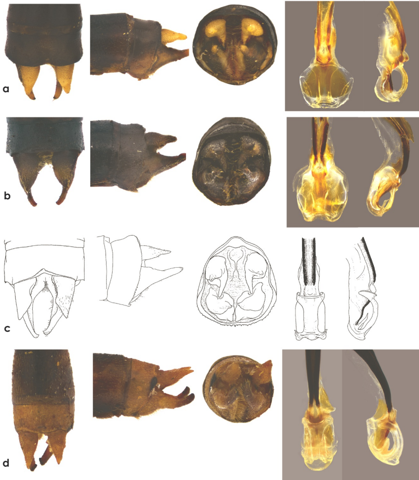
Figure 12. Comparison between the male appendages and penes of: a) Lieffinckia ulunorum , b) L. lairdi , c) L. salomonis , d) Salomoncnemis gerdae .
