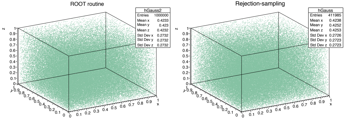
Figure 5.15: Each green dot represents an (x,y,z) -trio distributed according to a 3-D Gaussian distribution. They have been generated with the TRandom class in ROOT (left) and with our own rejection-sampling based algorithm (right). The boxes show the mean values and the standard deviations of (x,y,z) .
