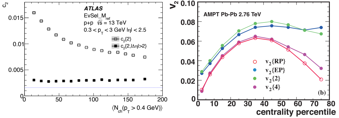
Figure 4.11: Left: c_2\{2\} measured by ATLAS in p+p collisions at \sqrt{s} = 13 TeV with and without a rapidity gap. Figure extracted from [163]. Right: elliptic flow simulated in the AMPT framework [164] with different analysis techniques covered in the text. Figure extracted from [165].
