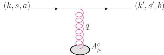
Figure C.1: One gluon exchange between a fast quark and a dense target.
