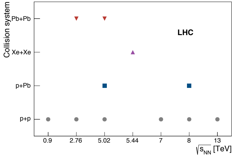
Figure 4.3: Compilation of collisions systems and energies investigated at the LHC. (Pb, Xe) stands for isotopes with atomic numbers ( ^{208}\text{Pb} , ^{154}\text{Xe} ).
