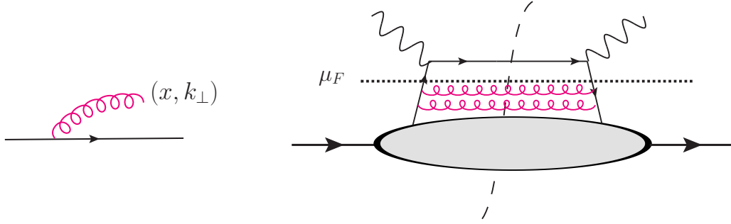
Figure 2.8: Left: a quark radiating a soft gluon with momentum components (x, \mathbf{k}_\perp) . Right: the transverse momenta of the gluons are smaller than the factorization scale so they are absorbed in the PDF via DGLAP equations. If k_\perp^2 > \mu_F^2 the gluon is a correction to the hard part.
