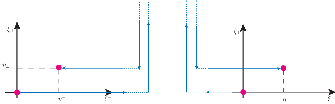
Figure 2.12: Left: Path of the gauge link in SIDIS as given by Eq. (2.32). Right: Path of the gauge link in DY as given by Eq. (2.33).
