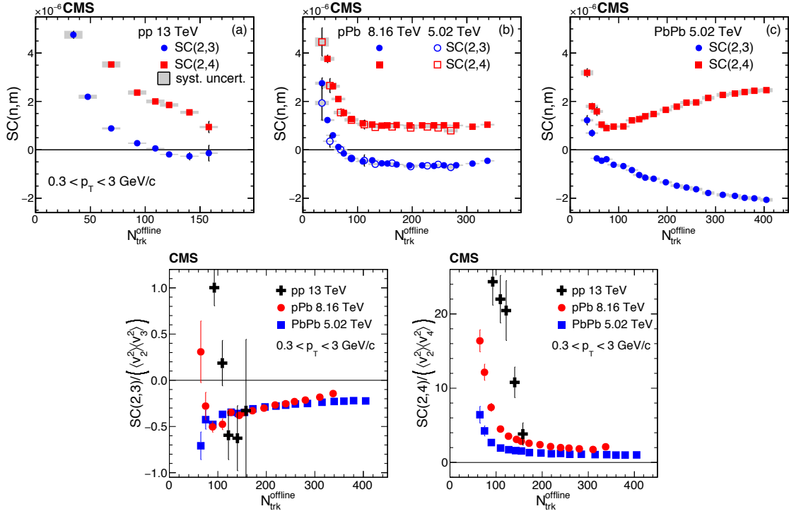
Figure 4.13: Top: SC(2,3) and SC(2,4) as a function of the multiplicity in the three collision systems. Bottom: normalized symmetric cumulants. Figures extracted from [173].
