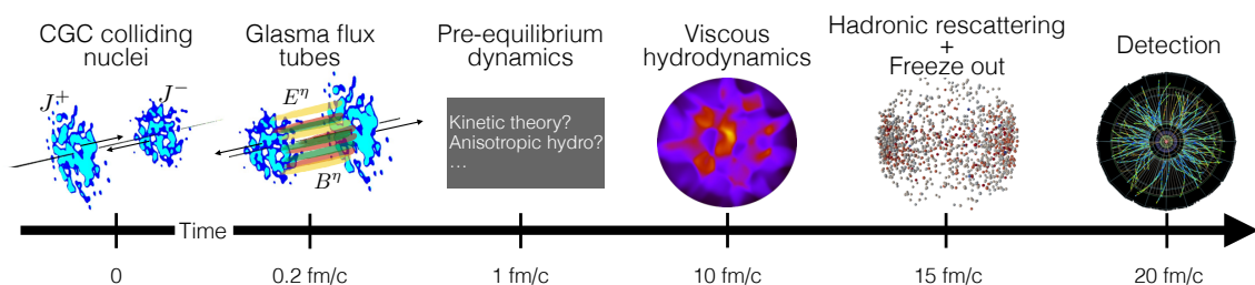
Figure 4.5: The standard model for heavy ion collisions.
