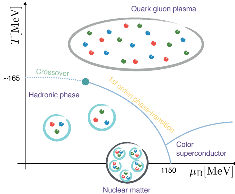
Figure 4.1: Sketch of the QCD phase diagram.
