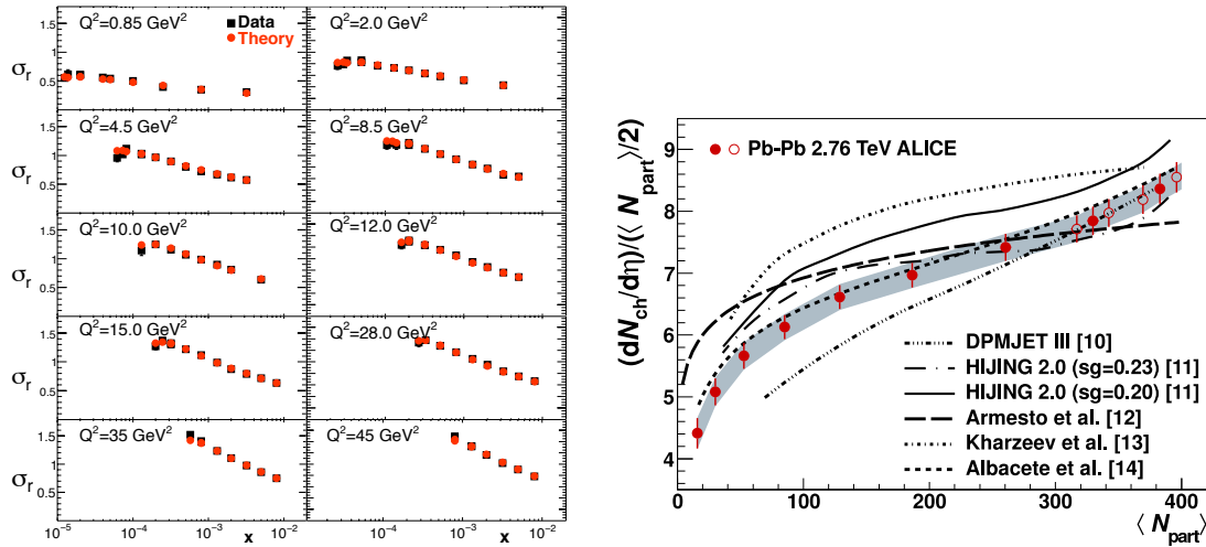
Figure 2.19: Left: Comparison of the CGC calculation of the reduced cross section, a combination of structure functions, with HERA data on electron-proton collisions. Figure extracted from [58]. Right: Measured multiplicities in a lead-lead collision at LHC energies compared to different theoretical predictions. Figure extracted from [59].
