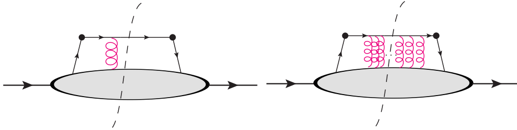
Figure 2.5: Left: One-gluon exchange between the parton and the background color field of its parent hadron. Right: n -gluon exchange as accounted by the Wilson line. The black dots represent any hard interaction that the struck quark may suffer. The dotted line represents the cut that distinguishes the scattering amplitude and its conjugate.
