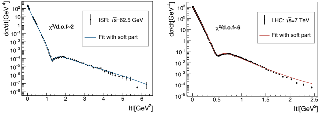
Figure 3.10: Fit to the differential elastic cross section with the T_g + T_{\text{soft}} parametrization for the two energies considered in this work. Left: ISR at \sqrt{s} = 62.5 GeV. Right: LHC at \sqrt{s} = 7 TeV.
