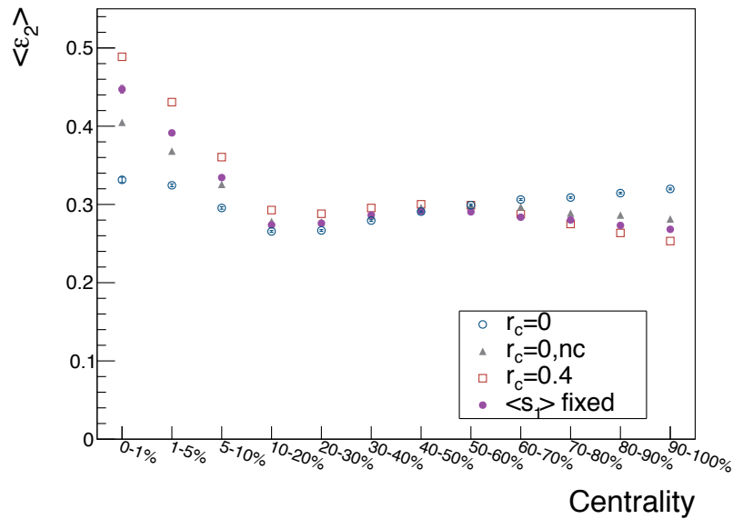
Figure 5.11: Average values of the eccentricity, \epsilon_2 , for r_c=0 (blue empty circle), r_c=0.4 fm (red empty square), r_c=0, nc (grey filled triangle) and \langle s_1 \rangle fixed (purple filled circle) as a function of the centrality range.
