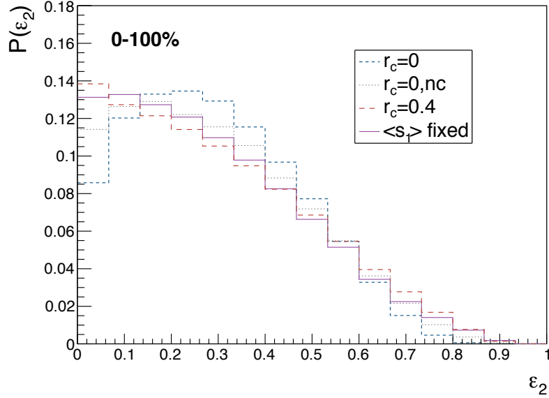
Figure 5.7: Probability distribution of the eccentricity, \varepsilon_2 , for r_c = 0 (blue short-dashed line), r_c = 0.4 fm (red long-dashed line), r_c = 0, nc (grey dotted line) and \langle s_1 \rangle fixed (purple solid line).
