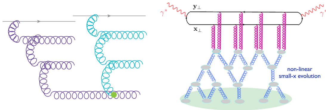
Figure 2.18: Left: Recombination of gluons coming from two different parton cascades. Right: Sketch of an electron-nucleus collision in the dipole model including multiple scatterings and non-linear small- x evolution. Figure extracted from [52].
