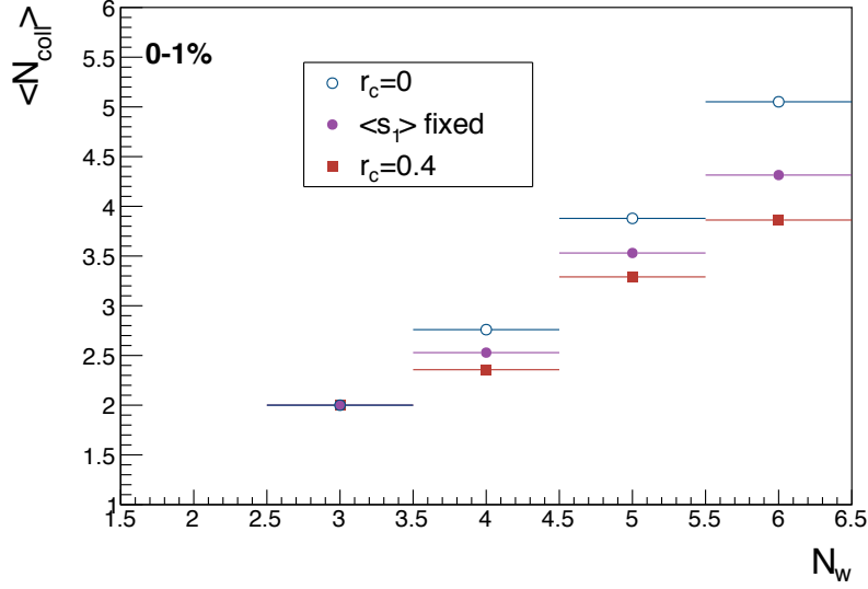
Figure 5.20: Average number of collisions as a function of the number of wounded hot spots for r_c = 0 (open blue circles), \langle s_1 \rangle fixed (filled purple circles) and r_c = 0.4 fm (filled red squares).
