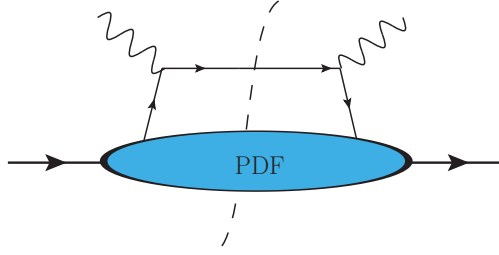
Figure 2.7: The hadronic tensor W^{\mu\nu} decomposed as the \gamma q -scattering and the parton distribution function.
