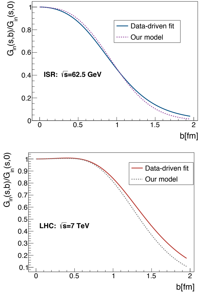
Figure 3.8: Comparison between the values G_{in} extracted from our model (dashed line) and the one obtained after fitting the experimental data (solid line) at ISR (top) and LHC (bottom) energies.
