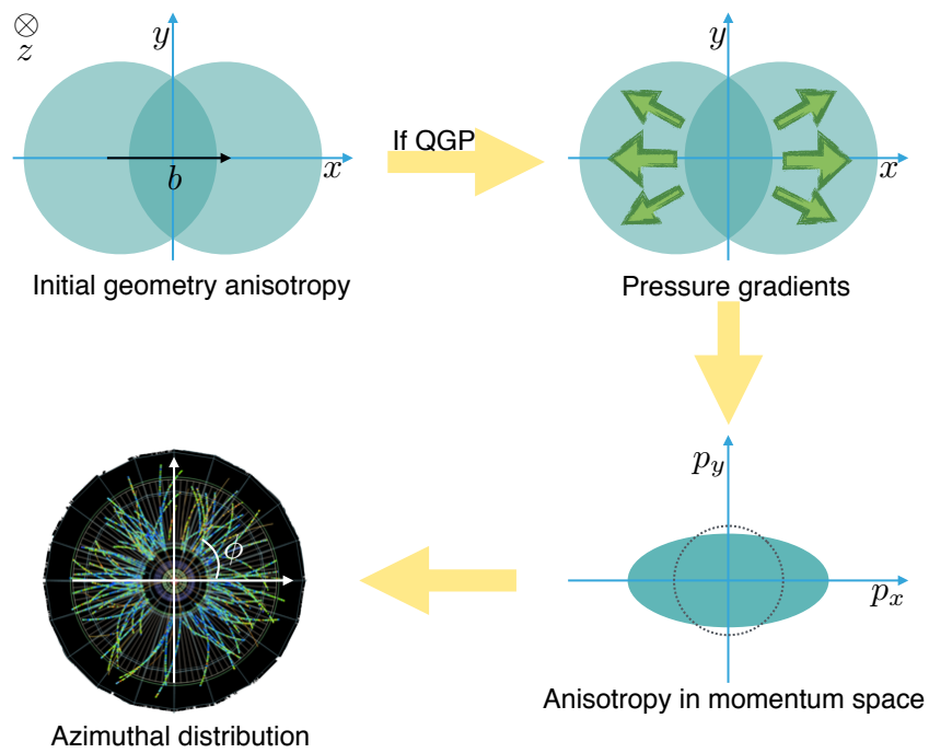
Figure 4.9: Collective flow in a peripheral heavy-ion collision. The impact parameter is directed along the x -direction and z denotes the beam axis.
