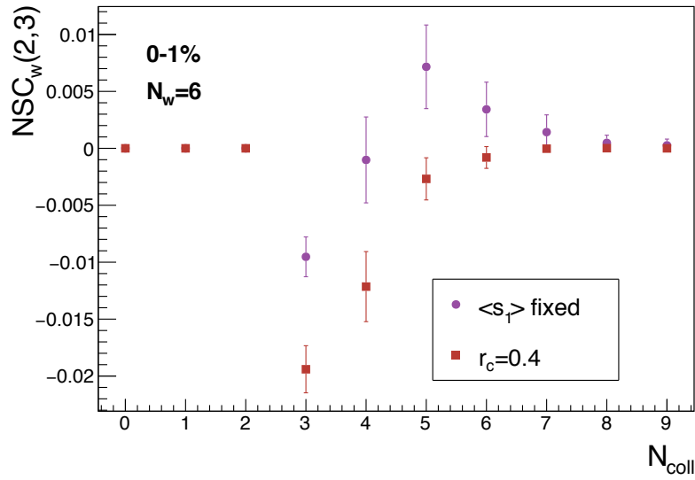
Figure 5.22: Average value of NSC_w(2,3) as a function of the number of collisions after selecting the events with N_w = 6 for \langle s_1 \rangle fixed (filled purple circles) and r_c = 0.4 fm (filled red squares).
