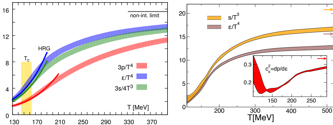
Figure 4.2: Left: pressure, energy density and entropy density as a function of the temperature. The vertical band marks the crossover region. Figure extracted from [104]. Right: energy and entropy densities. The subpanel shows the speed of sound. In both plots the arrows indicate the Stefan-Boltzmann limit i.e ideal massless gas limit. Figure extracted from [105]. This plot shows the agreement between the results obtained by the two major collaborations of the field: HotQCD (left) and Wuppertal-Budapest (right).
