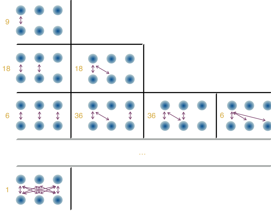
Figure 3.5: Different diagrams contributing to the multiple scattering expansion given by Eq. (3.22). The yellow numbers indicate the combinatorial factor associated to each diagram and the purple arrows the interactions between hot spots. The grey line indicates the 17 omitted diagrams.
