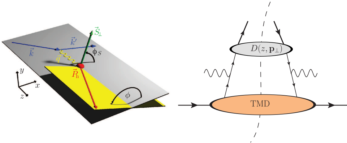
Figure 2.10: Left: Parton level SIDIS kinematics. Figure extracted from [25]. Right: SIDIS factorizes as the convolution of the TMD, the hard interaction with the virtual photon and the fragmentation function.
