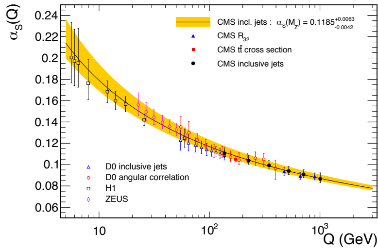
Figure 2.1: The strong coupling \alpha_s and its uncertainty (yellow band) as a function of the momentum transfer Q . Figure extracted from [9].
