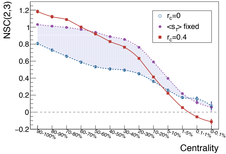
Figure 5.18: Average value of NSC(2,3) as a function of the centrality range for r_c = 0 (blue short-dashed line connecting open blue circles), \langle s_1 \rangle fixed (purple short-dashed line connecting filled purple circles) and r_c = 0.4 fm (red solid line connecting filled red squares). The error bars represent statistical uncertainties while the light violet band indicates the theoretical uncertainty associated to the choice of parameters that define the uncorrelated scenario.
