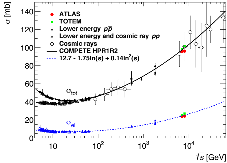
Figure 2.17: Total and elastic cross section measurements as a function of the centre of mass energy. Figure extracted from [51].
