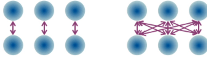
Figure 5.21: Sketch representing the interaction topologies preferred in the correlated case (left) and in the uncorrelated one (right). The purple arrows represent the collisions between the hot spots.
