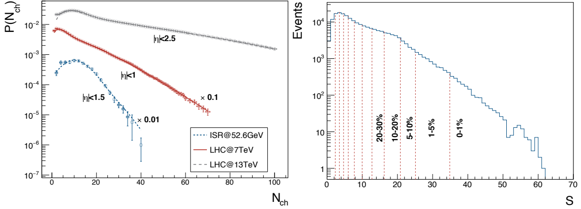
Figure 5.2: Left: Fit to the charged particle multiplicity distributions for different collision energies in the wounded hot spot model, Eqs. (5.5-5.7). The experimental data from top to bottom is taken from: ATLAS [206], ALICE [207] and ISR [208]. Note that each experiment has a different rapidity acceptance window, \eta , that influences the shape of the data. Also, the ALICE (red) and ISR (blue) curves are multiplied by 0.1 and 0.01 respectively. Right: Histogram of the integrated entropy deposition for the r_c = 0.4 fm case at \sqrt{s} = 13 TeV. Vertical red lines labelled by black numbers define centrality classes as fractions of the total number of events.
