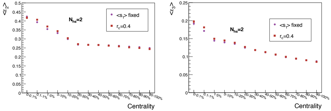
Figure 5.16: Average values of the eccentricity, \varepsilon_2 , (left) and the triangularity, \varepsilon_3 , (right) for N_{hs}=2 as a function of the centrality range.
