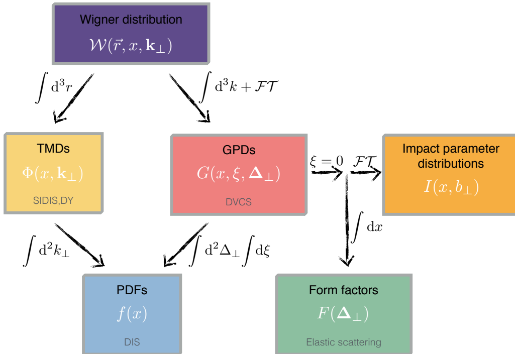
Figure 2.3: Sketch illustrating some of the quantities that can be derived from the Wigner distribution and the experimental processes where they can be measured. \mathcal{FT} denotes a Fourier transform from momentum to coordinate space.
