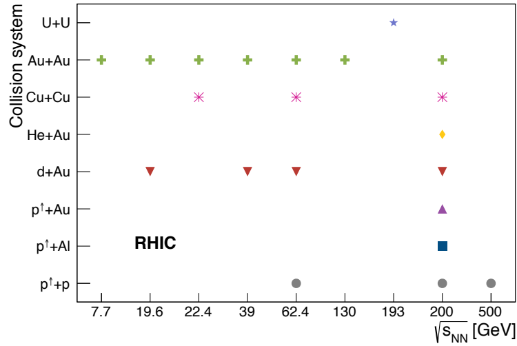
Figure 4.4: Compilation of collisions systems and energies investigated at the RHIC. (He,Al,Cu,Au,U) stands for isotopes with atomic numbers ( ^3\text{He} , ^{27}\text{Al} , ^{63}\text{Cu} , ^{197}\text{Au} , ^{238}\text{U} ). p^\uparrow indicates a polarized proton.
