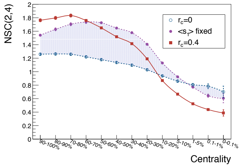
Figure 5.19: Average value of NSC(2,4) as a function of the centrality range for r_c = 0 (blue short-dashed line connecting blue open circles), \langle s_1 \rangle fixed (purple short-dashed line connecting filled purple circles) and r_c = 0.4 fm (red solid line connecting filled red squares). The error bars represent statistical uncertainties while the light violet band indicates the theoretical uncertainty associated to the choice of parameters that define the uncorrelated scenario.
