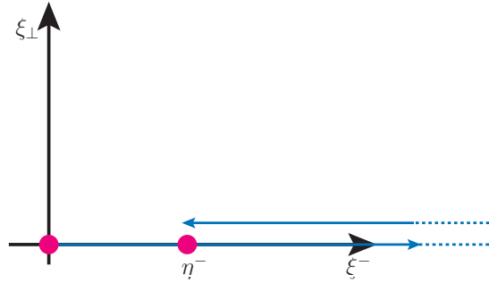
Figure 2.4: Path of the gauge link given by Eq. (2.19). The dotted lines indicate the extension up to \infty .
