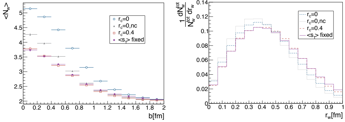
Figure 5.3: Left: Average number of wounded hot spots for different impact parameter bins of the collision. The horizontal lines indicate the width of the bins. Right: Normalized radial distribution of the wounded hot spots with respect to the reaction plane.
