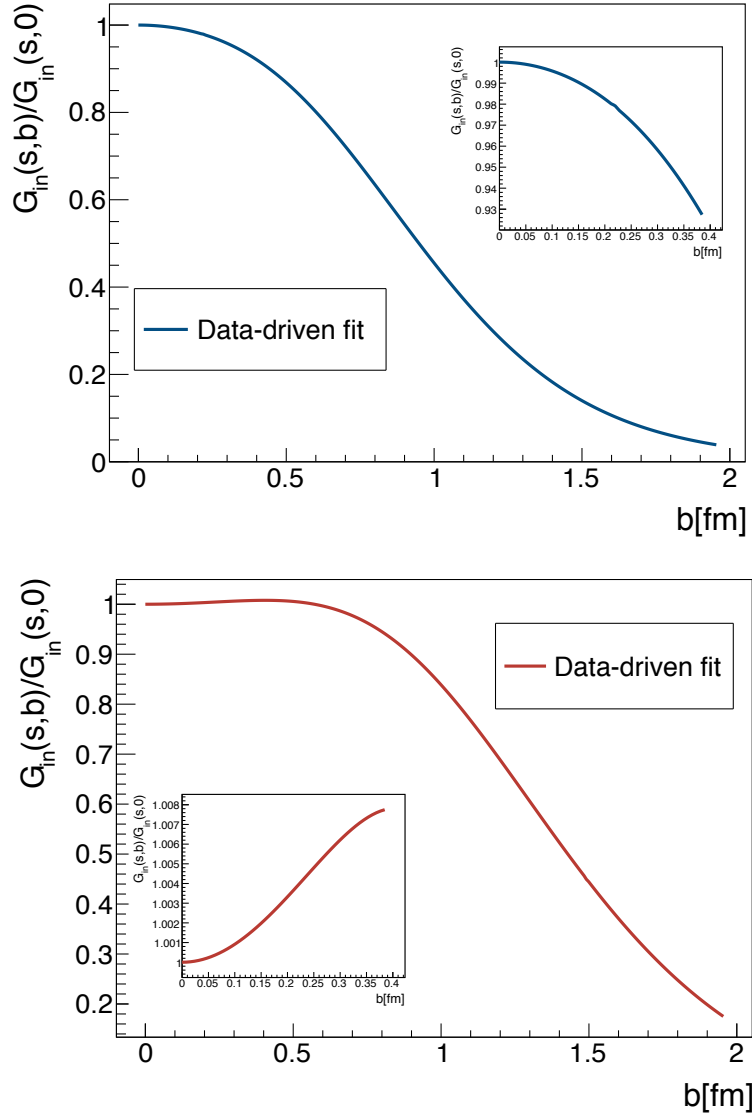
Figure 3.3: Normalized inelasticity density for \sqrt{s} = 62.5 GeV (top) and \sqrt{s} = 7 TeV (bottom). Sub-panels: zoom in the region of small b .
