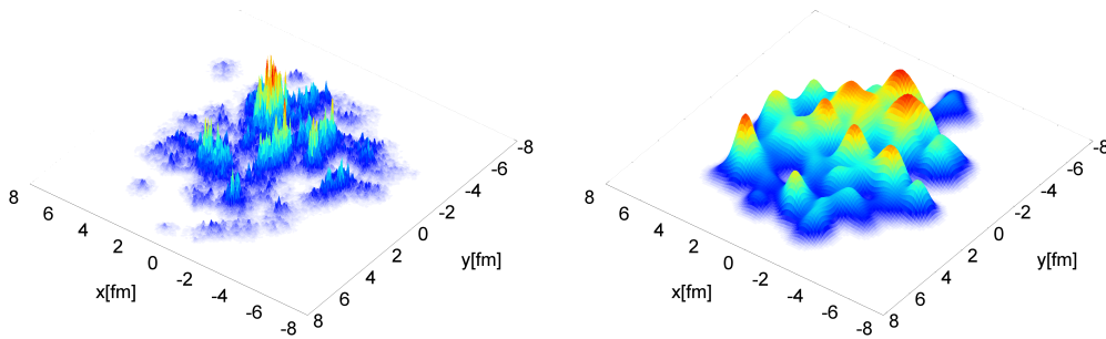
Figure 4.7: Initial energy density in the transverse plane obtained with IP-Glasma (left) and MC-Glauber (right) models. Figure extracted from [131].
