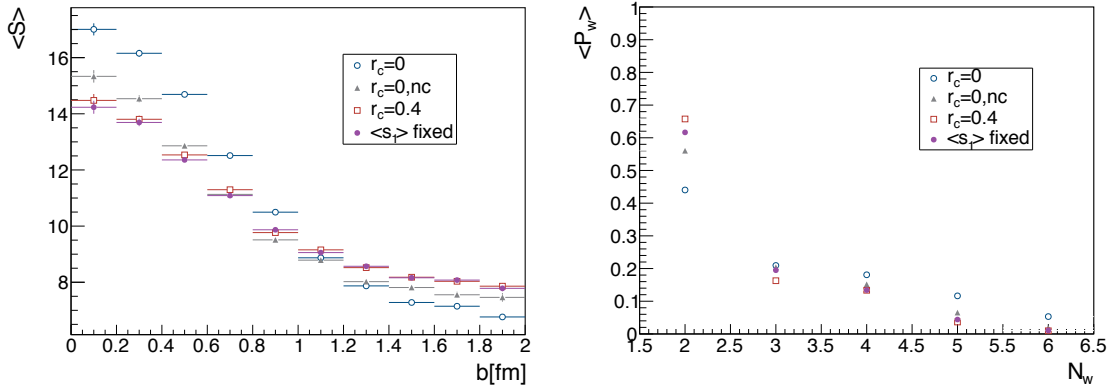
Figure 5.4: Left: Average entropy deposited as a function of the impact parameter. Right: Average probability of i hot spots to be wounded that enters into Eq. (5.5).
