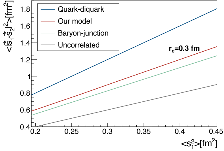
Figure 3.6: Mean transverse separation squared between pairs of hot spots as a function of the mean transverse position for different D(\{\vec{s}_i\}) as given by Eqs. (3.30), (3.34) and (3.35).
