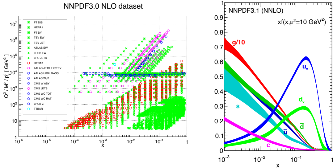
Figure 2.9: Left: Kinematic coverage in the (x, Q^2) -plane of different experiments. Right: The NNPDF3.1 NNLO PDFs, evaluated at \mu_F^2 = 10 GeV 2 . Figures extracted from [24].
