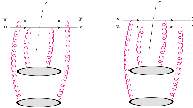
Figure 4.14: The grey blobs represent the domains of color fields in the target off which two independent quarks at transverse positions (x, u) scatter. The momentum kick is equivalent, in the conjugate coordinate space, to a shift in the positions in the amplitude and conjugate amplitude. Left: independent scattering of the two quarks. Right: connected diagram that leads to genuine correlations. Figures adapted from [183].
