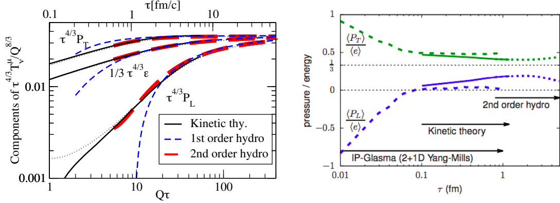
Figure 4.6: Left: Different components of the energy momentum tensor as a function of the proper time. Figure extracted from [124]. Right: Pressure evolution starting from a CGC-inspired model evolved through kinetic theory and matched to hydrodynamics. Figure extracted from [128].
