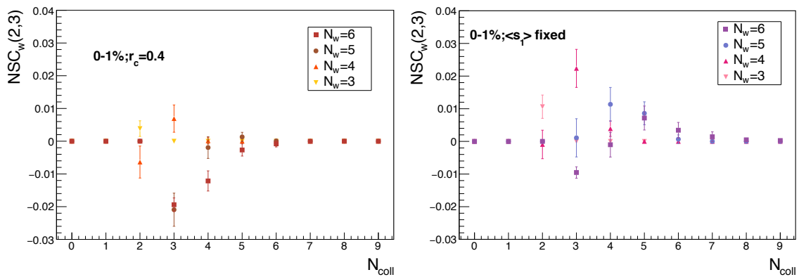
Figure 5.23: Average value of NSC_w(2,3) as a function of the number of collisions for different number of wounded hot spots. Left: r_c = 0.4 fm case. Right: \langle s_1 \rangle fixed case.
