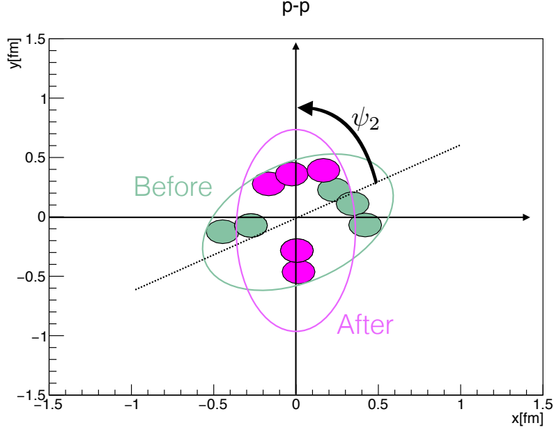
Figure 5.5: Illustrative example of a \sqrt{s} = 7 TeV p+p event with 5 wounded hot spots (green disks). The principal axes of the area formed by the wounded hot spots are tilted by an angle \psi_2 with respect to the reaction plane given by the axes ( x and y ) of the transverse plane. The purple disks represent the transformed coordinates.
