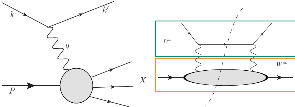
Figure 2.6: Left: Deep inelastic scattering: e(k)p(P) \rightarrow e(k')X . Right: Sketch representing the manifest separation between the leptonic tensor (green box) and the hadronic one (orange box).
