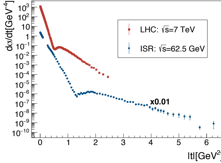
Figure 3.1: d\sigma_{\text{el}}/dt as a function of the momentum transfer at \sqrt{s} = 7 TeV (red squares) and \sqrt{s} = 62.5 GeV (blue dots). Note that the ISR data has been multiplied by 0.01 for readability. The error bars account for statistical uncertainties.
