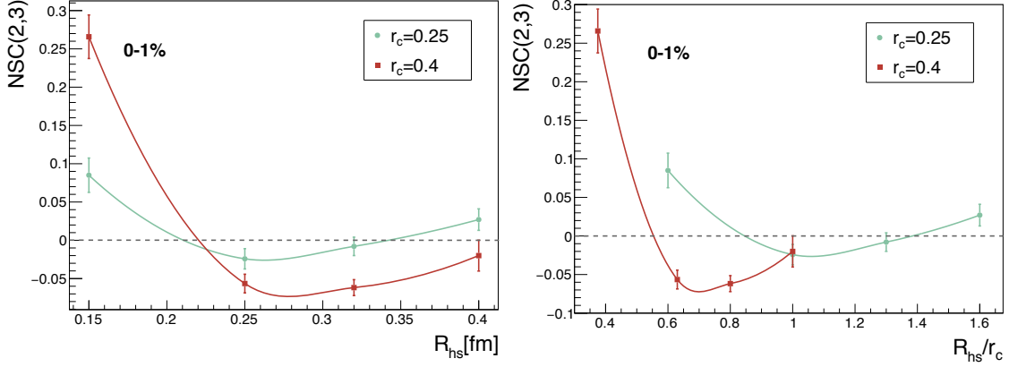
Figure 5.24: Average value of NSC(2,3) for two different values of the repulsive distance: r_c = 0.25 fm (filled green circles) and r_c = 0.4 fm (filled red squares) as a function of the radius of the hot spot (left) and the ratio R_{hs}/r_c (right).
