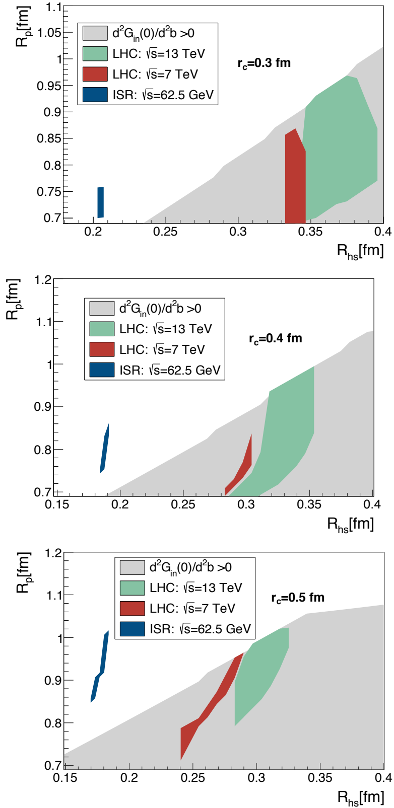
Figure 3.7: Hollowness region (filled-grey) and phenomenologically compatible regions with ISR and LHC data in the (R_p, R_{hs}) -plane for r_c = 0.3 (top), 0.4 fm (middle) and 0.5 fm (bottom).
