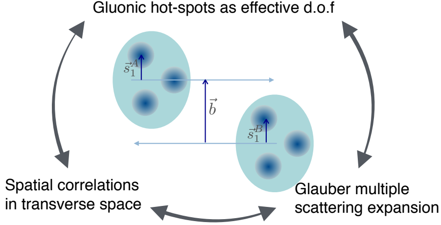
Figure 3.4: Sketch of the main ingredients of our description of proton-proton interactions.
