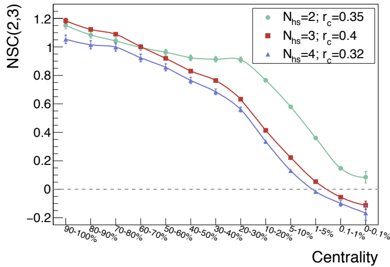
Figure 5.25: Average value of NSC(2,3) as a function of the centrality range in the correlated scenario for N_{hs} = 2 (filled green circles), N_{hs} = 3 (filled red squares) and N_{hs} = 4 (filled violet triangles). The error bars represent statistical uncertainties.
