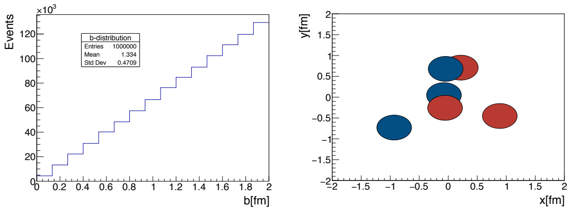
Figure 5.1: Left: impact parameter distribution as given by Eq. (5.1). Right: Typical event for p+p with the target constituents in red and the projectile ones in blue.
