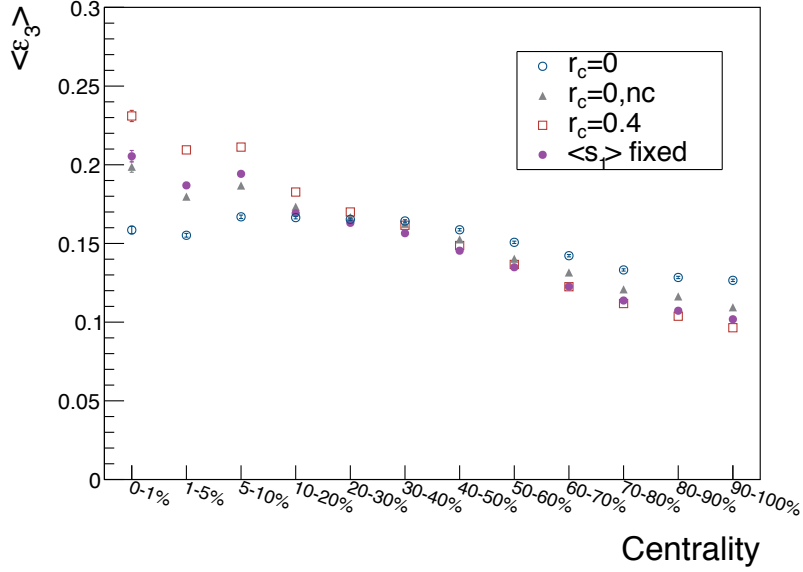
Figure 5.12: Average values of the triangularity, \varepsilon_3 , for r_c = 0 (blue empty circle), r_c = 0.4 fm (red empty square), r_c = 0, nc (grey filled triangle) and \langle s_1 \rangle fixed (purple filled circle) as a function of the centrality range.
