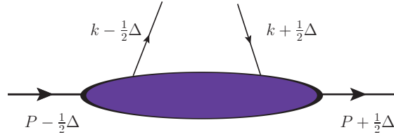
Figure 2.2: Kinematics for the quark Wigner distribution in terms of k , the quark momentum, P , the proton momentum, and \Delta , the momentum transferred to the proton.
