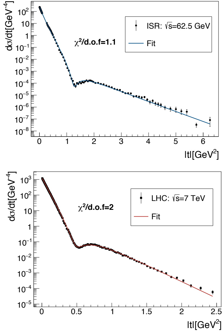
Figure 3.2: Fit to d\sigma_{\text{el}}/dt with the parametrization given in Eq. (3.14) for \sqrt{s} = 62.5 GeV (top) and \sqrt{s} = 7 TeV (bottom). The error bars account for statistical uncertainties. \chi^2(\alpha) = \sum_{i=1}^n (f(x_i, \alpha) - e_i)^2 / \sigma_i^2 where f is the theoretical parameterization that depends on the vector of free parameters being fitted \alpha and e_i are the individual measurements with uncertainties \sigma_i .
