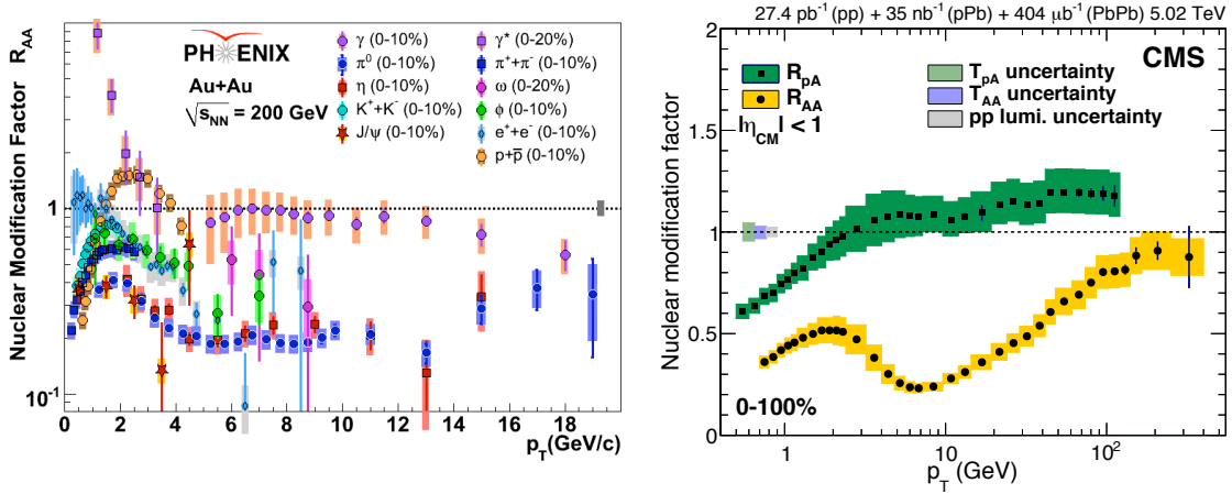
Figure 4.8: Nuclear modification factor at RHIC energies for different particles and centralities (left) and at LHC for Pb+Pb and p+Pb collision systems (right). Figures extracted from [151, 150].
