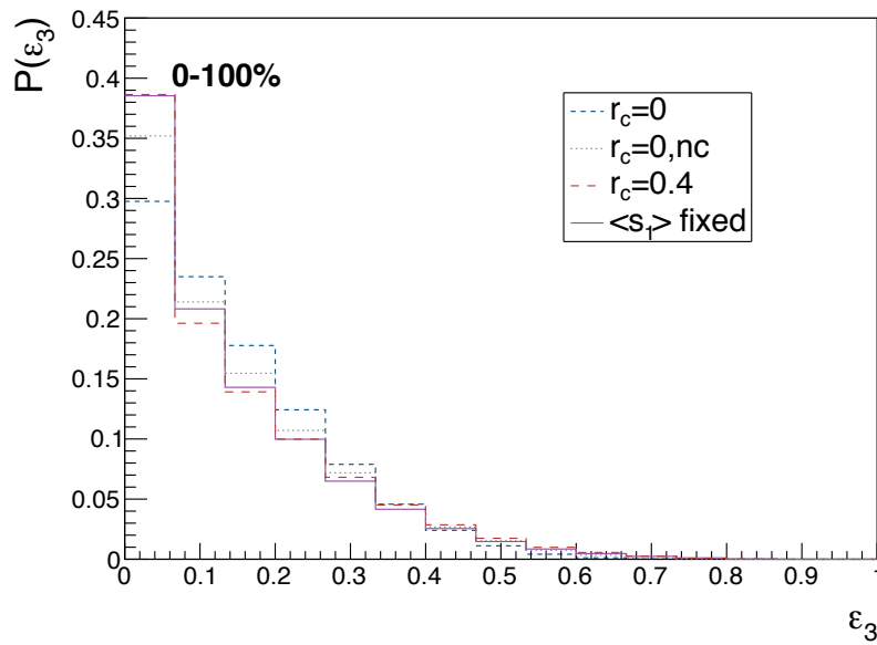
Figure 5.8: Probability distribution of the triangularity, \varepsilon_3 , for r_c = 0 (blue short-dashed line), r_c = 0.4 fm (red long-dashed line), r_c = 0, nc (grey dotted line) and \langle s_1 \rangle fixed (purple solid line).
