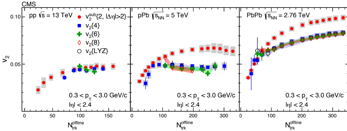
Figure 4.12: Integrated elliptic flow of unidentified charge particles as a function of the multiplicity. Figure extracted from [171].
