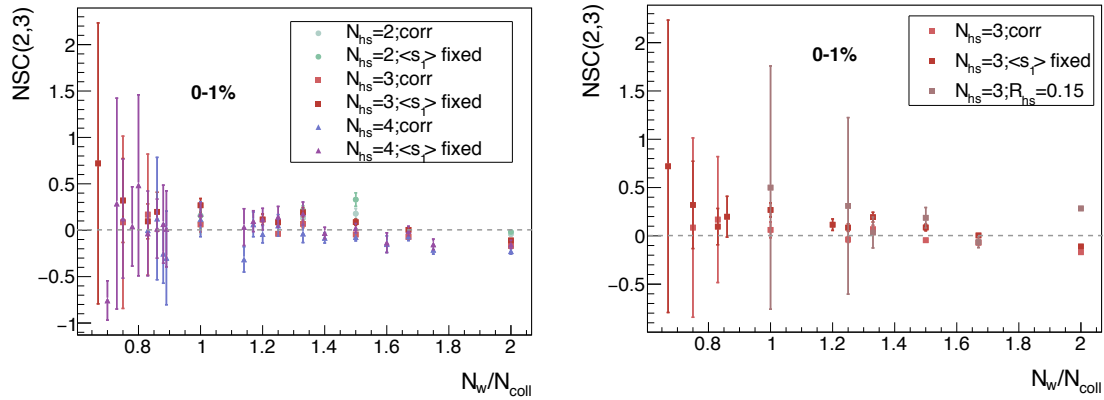
Figure 5.27: Average value of NSC(2,3) as a function of N_w/N_{coll} . Left: N_{hs} = (2, 3, 4) for the correlated and uncorrelated scenarios. Right: N_{hs} = 3 for the \langle s_1 \rangle fixed case and the correlated one with two different values of R_{hs} = (0.15, 0.32) .
