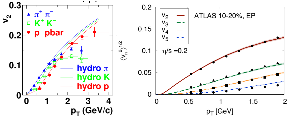
Figure 4.10: Left: elliptic flow measured by PHENIX in Au+Au collision at \sqrt{s_{NN}} = 200 GeV compared to a hydrodynamic calculation [155, 156]. Right: anisotropic flow coefficients measured by ATLAS in Pb+Pb collisions at \sqrt{s_{NN}} = 2.76 TeV compared to IP-Glasma+viscous fluid dynamics simulation [157].
