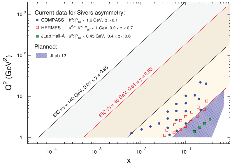
Figure 2.14: Kinematic coverage in the (x, Q^2) -plane expected in the Electron Ion Collider compared to other existing experiments for Sidis asymmetry. Figure extracted from [25].
