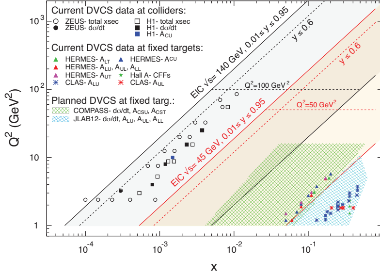
Figure 2.16: Kinematic coverage in the (x, Q^2) -plane expected in the Electron Ion Collider compared to other existing experiments for DVCS. Figure extracted from [25].
