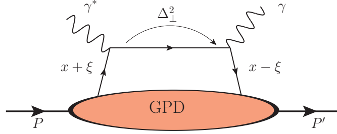
Figure 2.15: Kinematics of Deeply-virtual Compton Scattering.
