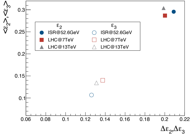
Figure 5.14: Average values of \varepsilon_2 (filled markers) and \varepsilon_3 (empty markers) for \sqrt{s} = 52.6 GeV (blue filled/empty circles), 7 TeV (red filled/empty squares) and 13 TeV (grey filled/empty triangles) as a function of their standard deviation. These energies correspond to ISR and Runs I-II of the LHC, respectively.
