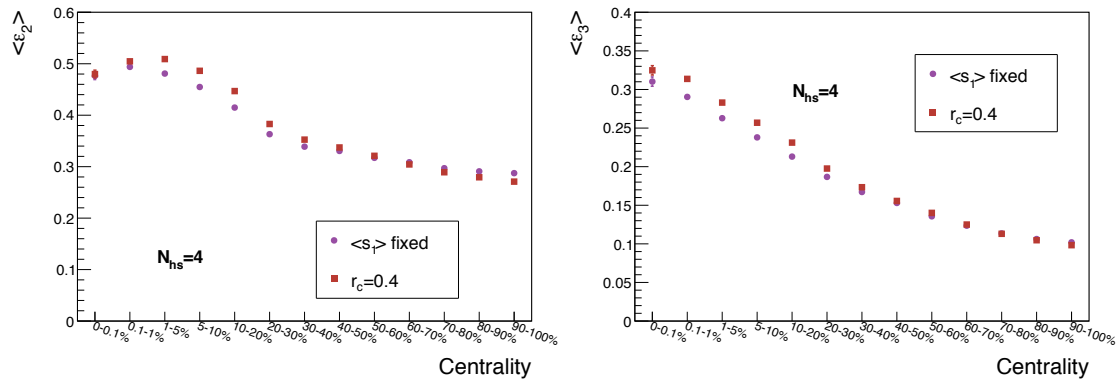
Figure 5.17: Average values of the eccentricity, \varepsilon_2 , (left) and the triangularity, \varepsilon_3 , (right) for N_{hs}=4 as a function of the centrality range.
