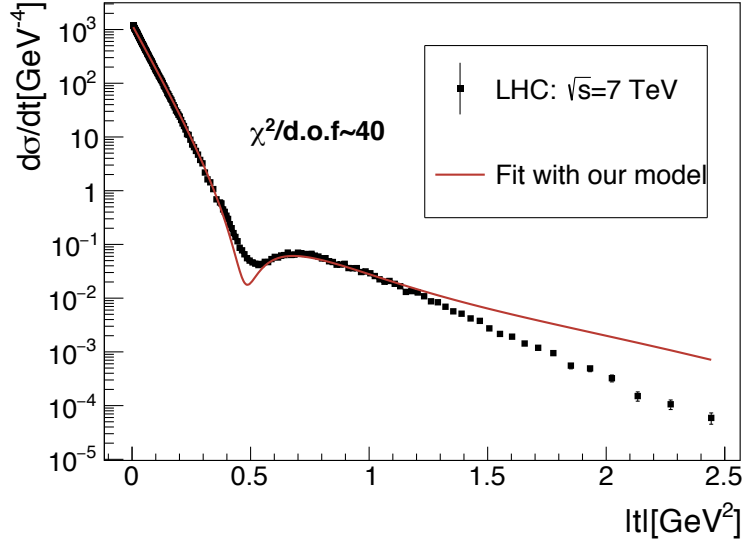
Figure 3.9: Fit to the differential elastic cross section using the parametrization of T_{\text{el}}(t) given by our model.
