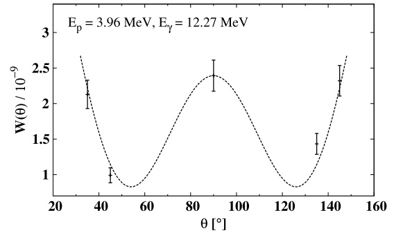
Fig. 2. Angular distribution for the \gamma_0 transition with an energy of E_\gamma = 12.27 MeV in ^{90}\text{Zr} for an incident proton energy of E_p = 3.96 MeV. The dashed line corresponds to the sum of Legendre polynomials fitted to the experimental W(\theta) values.
