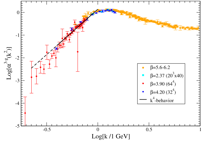
Fig. 1. The MOM three-gluon coupling defined in Eq. (7) obtained from all the different quenched lattice simulations described in the text. (For interpretation of the references to color in this figure, the reader is referred to the web version of this article.)
