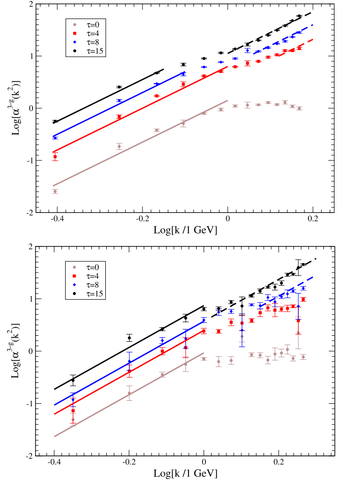
Fig. 2. The MOM three-gluon coupling defined in Eq. (7) obtained from quenched data with \beta = 4.20 (top panel) and unquenched with \beta = 1.95 (bottom panel) lattice simulations at different flow times.
