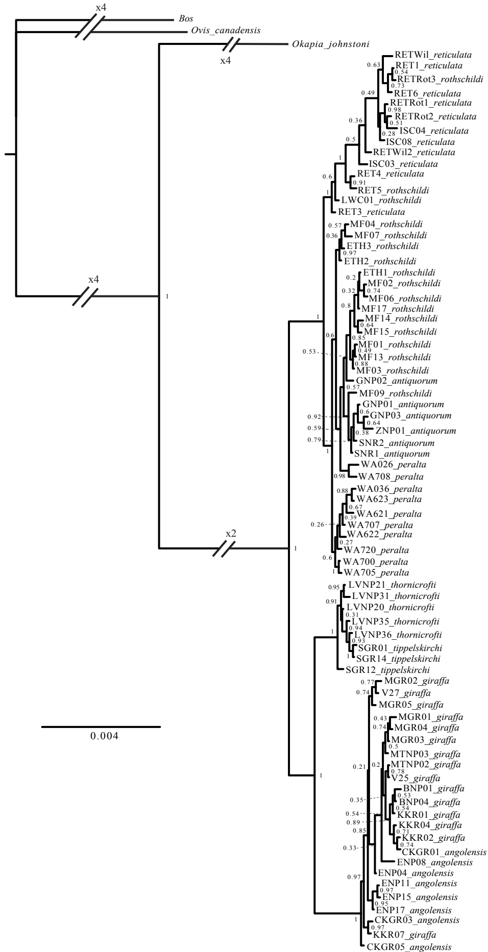
Supplementary file 6. Bayesian tree from the analysis of the concatenated alignment of 21 nuclear markers for 75 giraffes (17.275 bp) and three outgroup taxa. The posterior probability values are indicated for each node.
