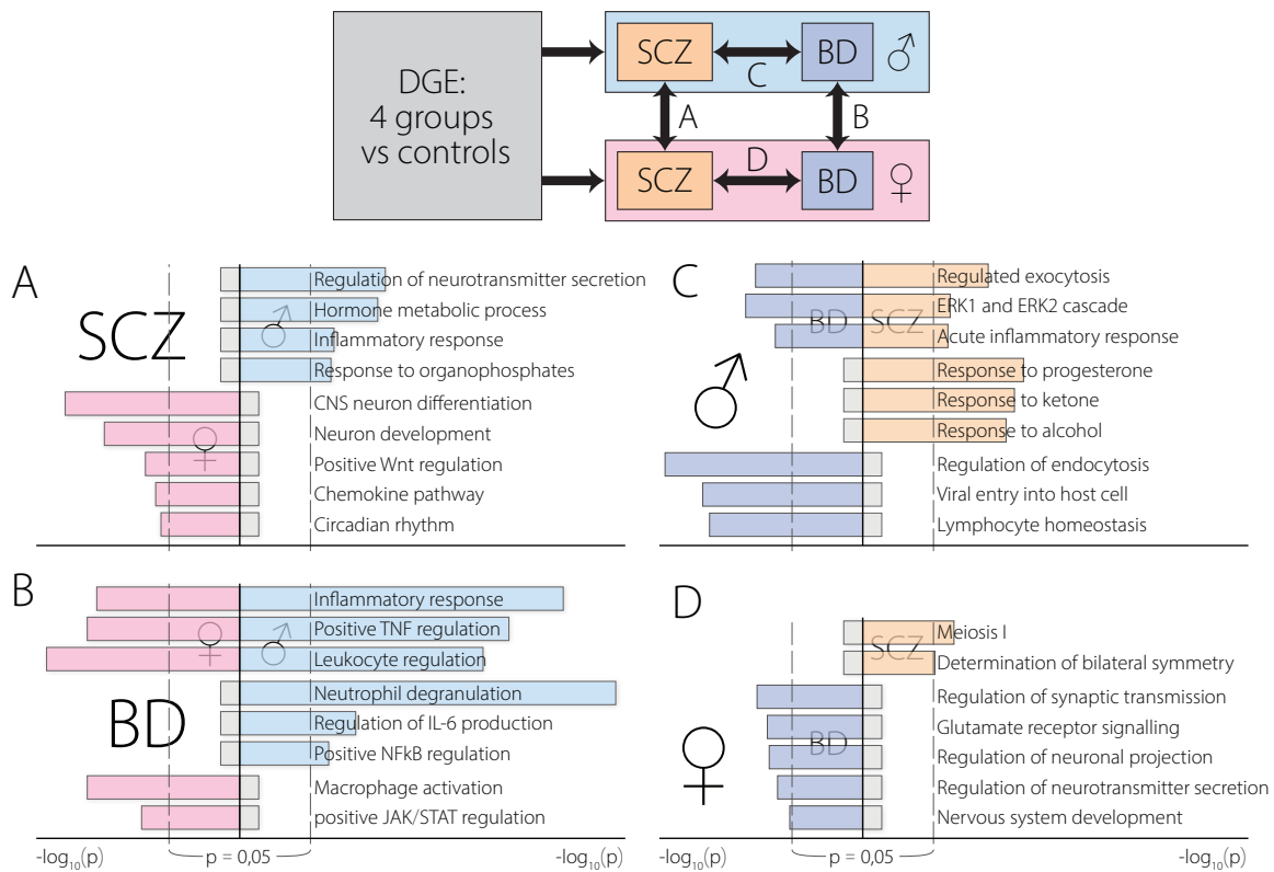
Figure 3.12: GO Enrichment of Diverging Genes. Results of differential gene expression were dually compared: SCZ versus BD and male versus female (indicated by colours). GO enrichment of the top 100 distinguishing genes in one dimension was compared with the other for each pair of combinations. A) SCZ-biased genes diverge between males and females. B) BD-biased genes share immunological ontology in both males and females. C) Male-biased genes share immunological ontology in BD and SCZ. D) Female-biased genes diverge between SCZ and BD.
