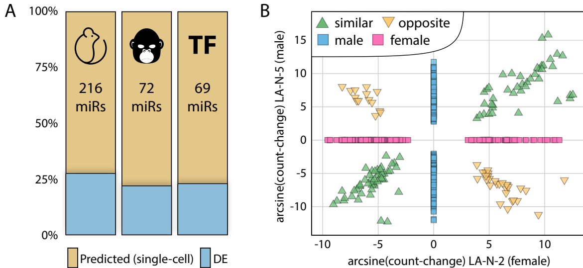
Figure 3.7: Differentially Expressed microRNAs in LA-N-2 and LA-N-5. A) Differential expression in sequencing of LA-N-2 and LA-N-5 identified approximately 25% of miRNAs predicted by permutation analysis of single cells expressing cholinergic markers (compare Figure 3.2 E) in all miRNA subgroups (evolutionarily conserved, primate-specific, and TF-targeting). B) Differentially expressed miRNAs in LA-N-2 and LA-N-5 can be stratified into four groups by their expression changes: miRNAs only differentially expressed in LA-N-2 (pink) or LA-N-5 (blue), miRNAs changed in similar direction in both cell lines (green) and miRNAs changed inversely between cell lines (yellow). Notably, the changes in expression as measured by count-change in similarly as well as inversely changed miRNAs both correlate well.
