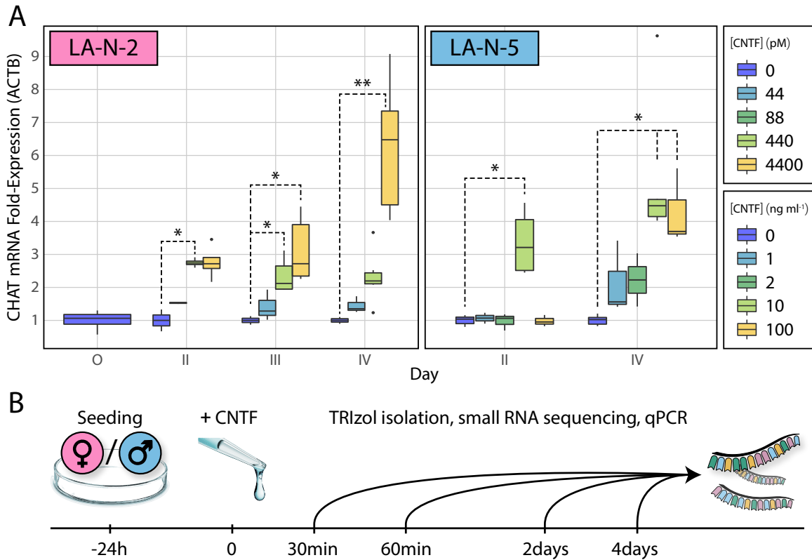
Figure 3.4: Time-dose curve of CNTF-mediated differentiation of LA-N-2 and LA-N-5. A) Cells were stimulated with varying doses of CNTF, and lysed at various time points to determine CHAT mRNA levels via qPCR. Expression ( \Delta\Delta C_t ) was normalised to house-keeping genes (ACTB, GAPDH, RPLP0) and to control sample without CNTF to determine fold-changes. LA-N-5 reacts strongest to a concentration of 10 ng ml -1 , while LA-N-2 reacts strongest to 100 ng ml -1 . *: p < 0.05, **: p < 0.001 B) Cells were seeded at ~2E05 cells/well in a 12-well-plate. After 24h, CNTF was added to the existing medium as quickly as possible to avoid disturbance. Cells were lysed in situ at time points 30 minutes, 60 minutes, 48 hours, and 96 hours using TRIzol for downstream RNA processing.
