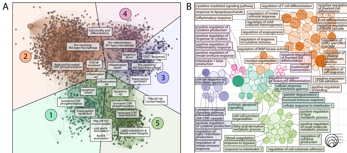
Figure 5.7: Comparison of Annotated Feedforward Loop Network and t-SNE Visualisation of Module GO Terms. A) Reproduction of Figure 4.12, colours have been adapted to allow module comparison between A and B. Displayed is the network of all CD14 + -specific FFLs, stratified into five modules, and overlaid with module-specific GO analysis results. B) Reproduction of Figure 4.11 B. Displayed is the t-SNE-based visualisation of all module-specific GO terms from the CD14 + FFL-network (A), coloured by module. The distance between nodes is based on amount of shared genes between terms, depth of colour represents significance level, size of node represents number of genes in term.
