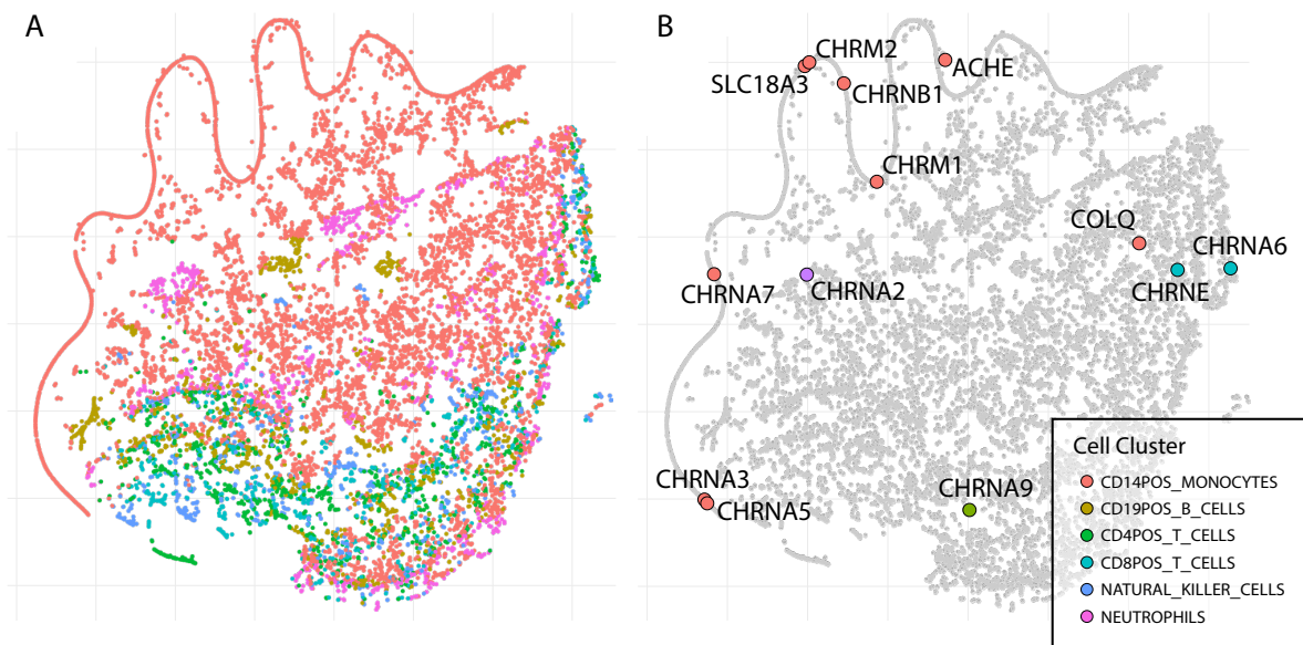
Figure 4.6: Large RNA Expression Patterns in Blood-Borne Cells. Expression derived from transcriptional activity in blood-borne cell types in the Marbach dataset 118 was visualised via t-SNE. The input matrix comprised all 14 280 detected genes in 6 types of blood-borne immune cells. Genes were plotted on the first two t-SNE dimensions and coloured by the cell type of their highest expression, i.e., the highest cumulative transcriptional activity of all active TFs. A) Complete t-SNE shows a gradient of expression across the different cell types, with much expression in CD14 + monocytes and T-cells. B) Highlighting of cholinergic core genes reveals an enrichment in close compartments of CD14 + monocytes. The vesicular ACh-transporter SLC18A3 can serve as substitute for the main cholinergic marker, CHAT, as discussed in Section 2.2.3.
