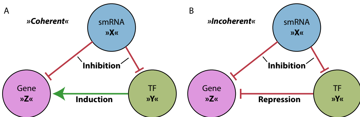
Figure 4.9: Small RNA Feedforward Loop Theory. The figure represents the two cases of smRNA FFLs most accessible to current analysis methods, i.e., the cases of smRNA ( X ) targeting of TF ( Y ) and ultimate gene ( Z ). A) Basic coherent smRNA FFL. The smRNA ( X ) inhibits both the TF as well as the ultimate gene target. Since the TF ( Y ) is an activator of target gene ( Z ) expression, smRNA regulation has the same direct and indirect effect on ultimate gene expression. B) Basic incoherent smRNA FFL. The smRNA ( X ) has a direct suppressive effect on the target gene ( Z ), but the simultaneous suppression of the TF ( Y ), which in turn represses the target gene ( Z ), leads to elevation of target gene expression, ameliorating or even inverting the direct effect.
