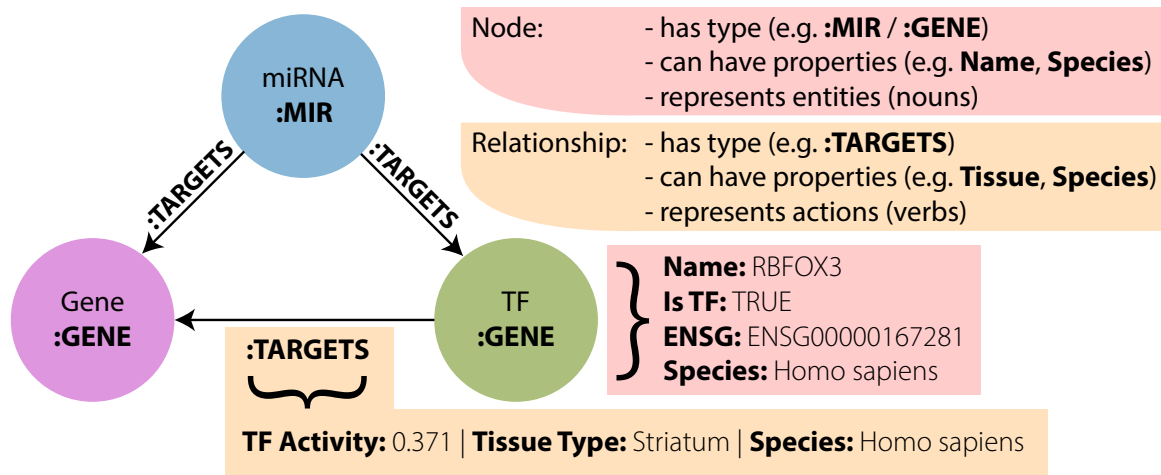
Figure 2.1: Organisation of a Graph Database. A graph consists of two basic building blocks: Nodes , representing entities, and edges , representing connections between entities. Each database entry (node or edge) is an instance of a particular type and can possess an arbitrary amount of properties detailing its specifics.
