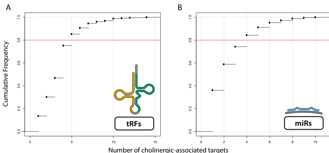
Figure 4.1: Cholinergic-associated Small RNA ECDF Curves. Cholinergic association was tested using miRNeo targeting data of miRNAs and tRFs. To assess the best-suited threshold for defining cholinergic association, empirical cumulative density functions were calculated for the number of cholinergic-associated (CA) genes targeted by each unique smRNA. A ) Cumulative frequency of number of CA genes targeted by tRFs. Threshold of 80% (red line) is passed at five CA genes targeted. B ) Cumulative frequency of number of CA genes targeted by miRNAs. Threshold of 80% (red line) is passed at four CA genes targeted.
