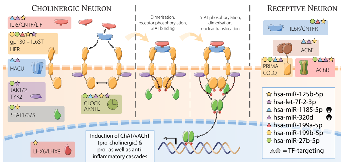
Figure 5.5: The Cholinergic/Neurokine miRNA Interface. The neurokinins, such as CNTF, LIF, and IL-6, signal through a combination of soluble and membrane-bound receptors. Activation of a transmembrane neurokine receptor is usually followed by JAK recruitment and phosphorylation, and successively by STAT activation and translocation to the nucleus. Gp130-family neurokine, cholinergic, and circadian signalling pathways are controlled by primate-specific and evolutionarily conserved miRNAs. miRNA targeting of individual genes (indicated by coloured symbols) yields complex transcriptional interactions. Several miRNAs directly targeting the cholinergic pathway also target TFs controlling this pathway (circles and triangles).
