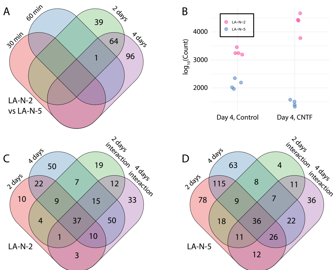
Figure 3.9: miRNAs Differentially Expressed Between LA-N-2 and LA-N-5. Application of a design model formula which includes an interaction term enables display of the influence of the male or female genotype on differential miRNA expression. A) Venn diagram of miRNAs differentially expressed between LA-N-2 and LA-N-5 at all four time points. B) Counts plot of normalized raw expression values of hsa-miR-615-3p. Exemplary of a high influence of genotype on the differential expression caused by CNTF differentiation, hsa-miR-615-3p is more highly expressed in the female LA-N-2 and elevated after four days of CNTF-induced differentiation, while in the male LA-N-5, it is expressed slightly lower and suppressed upon differentiation. C) Venn diagram comparing late differential expression in LA-N-2 with late time points of differential expression between LA-N-2 and LA-N-5. All possible combinations exist, however, there are miRNAs affected by genotype that are not differentially expressed in the simple model. D) Venn diagram comparing late differential expression in LA-N-5 with late time points of differential expression between LA-N-2 and LA-N-5. Essentially similar to C , but with partly higher quantities of DE miRNAs.
