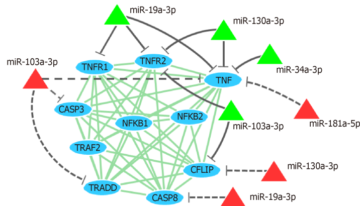
Figure 5.2: Interaction network showing miRNAs and their predicted and validated targets. The protein interaction network (light gray lines) shows the interaction between proteins (ellipses) encoded by tumor necrosis factor- \alpha pathway genes. Green triangles and solid gray lines represent miRNAs and validated target genes, respectively; red triangles and dotted gray lines represent predicted relationship between miRNA and target genes, respectively. TNF: Tumor necrosis factor. Image and caption from Rossi et al. 306
