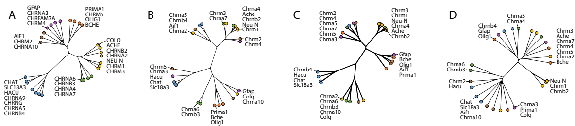
Figure 3.3: Clusters of Cholinergic Genes in Single-Cell Sequencing. Cholinergic genes were clustered using Bray-Curtis dissimilarity in four public data sets of single-cell sequencing. The displayed dendrograms visualise the distance between the genes across all samples. Gene clusters were coloured by grouping in Darmanis et al. 138 (A). Notably, genes clustered according to their biological function, for instance, CHAT , vAChT and HACU always are closely associated (blue), as are the genes comprising the putative »cholinceptive« neuron (yellow). A) Single-cell sequencing of the human developing neocortex. 138 B) Clustered single-cell sequences from transgenic mouse somatosensory cortex and hippocampus. 140 C) Clustered single-cell sequences from transgenic mouse somatosensory cortex and hippocampus. 139 D) Single-nucleus sequencing of adult mouse hippocampus. 141 Marker genes are: NeuN - neurons; OLIG1 - oligodendrocytes; AIF1 - microglia; GFAP - astrocytes.
