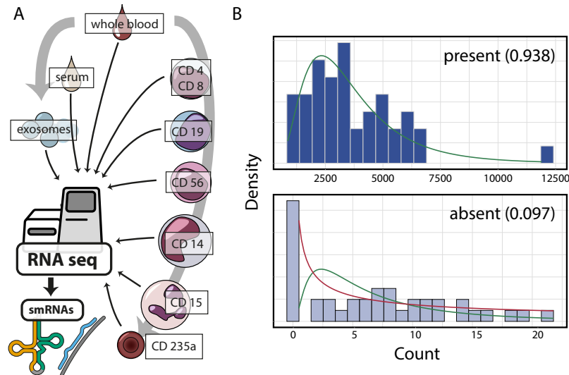
Figure 4.4: Small RNA Sequencing of Sorted Cell Types of the Blood and Definition of Presence/Absence. A) Data deposited by Juzenas et al. 208 include smRNA-information on CD4 + T-helper cells, CD8 + cytotoxic T-cells, CD14 + monocytes, CD15 + neutrophils, CD19 + B-cells, CD56 + natural killer cells, CD235a + erythrocytes, serum, exosomes, and whole blood. Raw data were re-analysed to yield miRNA- and tRF-expression levels. B) Definition of presence or absence of small RNA molecules from RNA-sequencing data is based on log-normality of count data, irrespective of expression levels. Log-normal distributions were calculated using the mean and standard deviation of expression levels (green lines) and compared to the actual distribution via the Kolmogorov-Smirnov test. Presence (upper example) was assumed at a relatively stringent level of p > 0.1 . The red line indicates a power-law distribution in comparison (absence, lower example).
