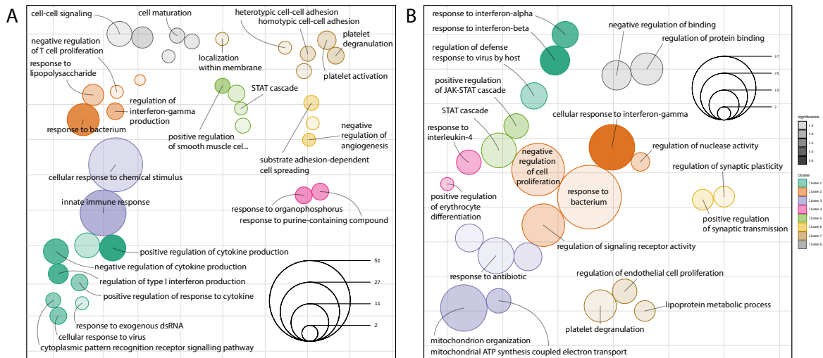
Figure 4.2: Large RNA Differential Expression Gene Ontology Enrichment. GO terms from enrichment analysis were projected on a 2D map via t-distributed stochastic neighbour embedding (t-SNE) analysis of their shared significant genes. Size of circle indicates number of significant genes in term, depth of colour indicates p-value (all p < 0.05 ). A) t-SNE visualisation of GO terms of DE genes with LFC > 1.4 shows 36 terms in eight clusters. Immunological terms (left-hand side) and circulatory terms (right-hand side) are predominant. B) t-SNE visualisation of 24 GO terms of top 100 genes measured by count-change corroborate immunological changes in stroke patient blood differential gene expression.
