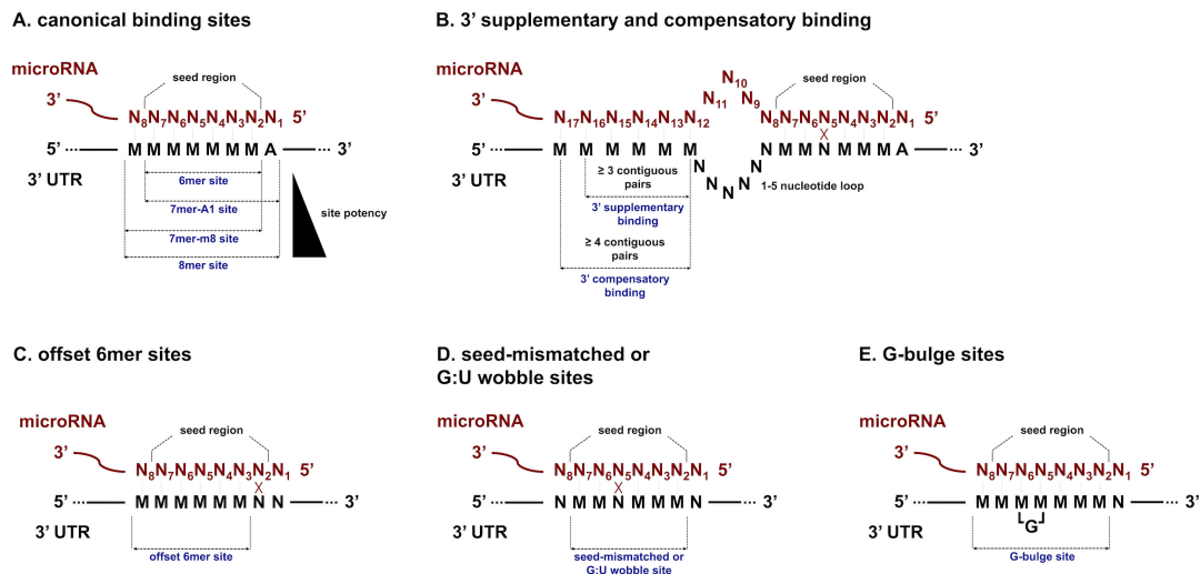
Figure 1.5: miRNA Binding Modes. miRNAs can bind to their target transcripts via a range of binding modes. N: any nucleotide; M: matching nucleotide. A) Simple seed matching of complementary bases (indicated by grey lines) is called canonical binding. Canonical sites can have different lengths and starting points. B) Seed pairing can be supplemented by complementarity in the 3' region of the miRNA, often after a »bridge« of non-complementary bases. This is particularly relevant in case of a mismatch in the seed (indicated by red »X«). Possible but less frequent are also C) offset 6-mer sites, D) seed-mismatched or G:U wobble sites, and E) G-bulge sites. Figure modified from van Peer et al. 94
