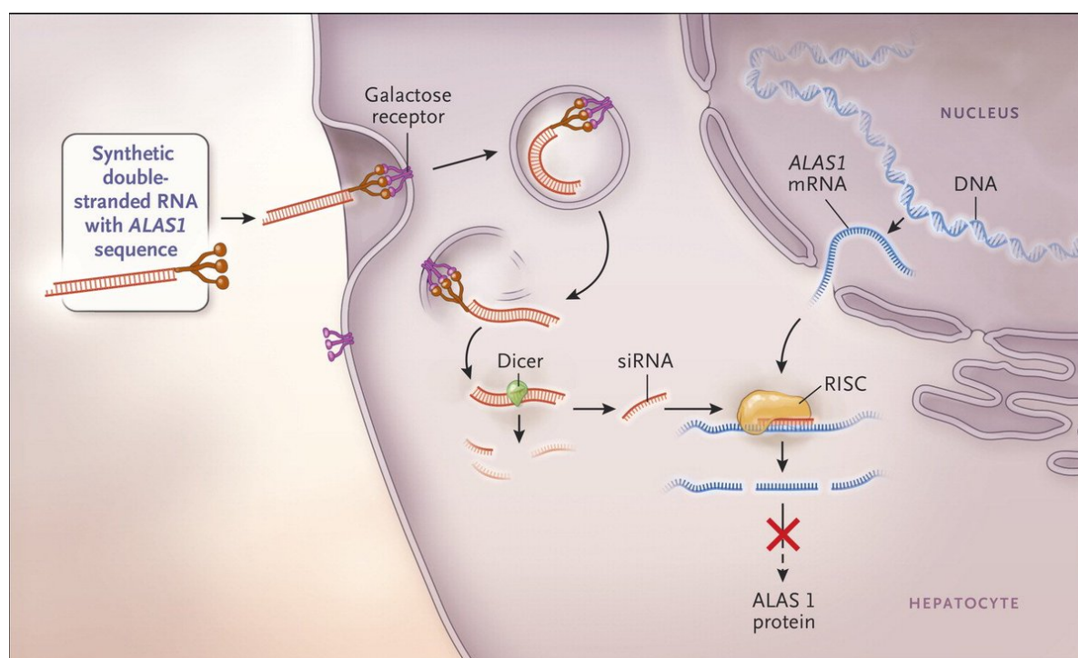
Figure 5.9: The Mechanism of Small Interfering RNA (siRNA) Therapy. Synthetic double-stranded RNA containing an ALAS1-specific sequence is derivatized with N-acetylgalactosamine to target the asialoorosomuroid (galactose) receptor, which is expressed nearly exclusively on hepatocytes. Within the hepatocyte, the RNA is processed into approximately 20-bp fragments by a cellular enzyme (dicer), and then separated into single strands. The strand that is complementary to ALAS1 (the guide strand) binds to cellular ALAS1 messenger RNA (mRNA) and enters the RNA-induced silencing complex (RISC), where the new double-stranded RNA is cleaved by a group of factors that include argonaute, a ribonuclease. The result is a reduction in the level of delta ALA synthase 1 protein and decreased production of ALA. Image and caption by Dr. Gerald Diaz. 347
