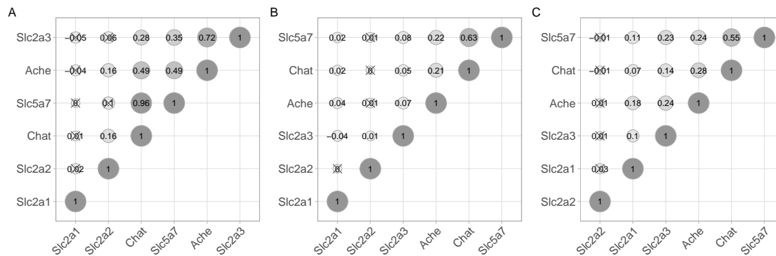
Figure 5.3: Correlation between CHAT and SLC5A7 in Nervous Cells. CHAT: choline acetyltransferase, SLC5A7: high affinity choline transporter (also known as CHT1), SLC2A1-3: passive glucose transporters. Size and depth of colour of circles denote strength of correlation (Pearson's product-moment correlation coefficient, PPMCC), numbers denote PPMCC (range: -1 to 1). Non-significant correlation coefficients ( p > 0.05 ) are crossed out. Rows and columns are ordered by hierarchical clustering, representing similarity of PPMCC values (Euclidian distance). (A) Correlation of transcripts in all tissues (cell-type-level) of the murine nervous system. (B) Correlation in all neurons (single-cell-level) of the murine nervous system. (C) Correlation in cholinergic neurons (single-cell-level) as determined by expression of the vesicular ACh-transporter, SLC18A3. Modified from Yuliani et al. 308
