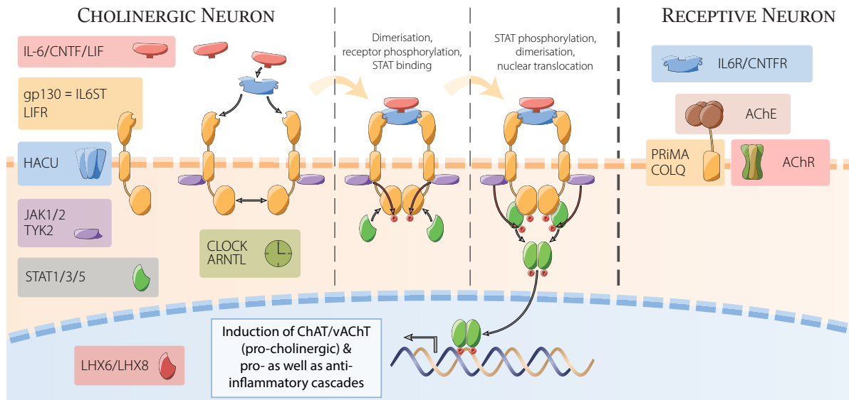
Figure 1.3: The Neurokine Pathway. The neurokines, such as CNTF, LIF, and IL-6, signal through a combination of soluble and membrane-bound receptors. Activation of a transmembrane neurokine receptor is usually followed by JAK recruitment and phosphorylation, and successively by STAT activation and translocation to the nucleus. Other aspects of the figure refer to the probable distinction between the cholinergic neuron (left side) and the »cholinceptive neuron« (right side), the latter of which possesses ACh receptors and AChE for degradation of the transmitter, and which may also produce soluble neurokine receptors. The phenotype of cholinergic cells is controlled by cholinergic-specific transcriptional regulators such as LHX6 and LHX8, circadian regulators such as CLOCK and ARNTL, and by inducible and broad transcriptional regulation via the JAK/STAT pathway.
