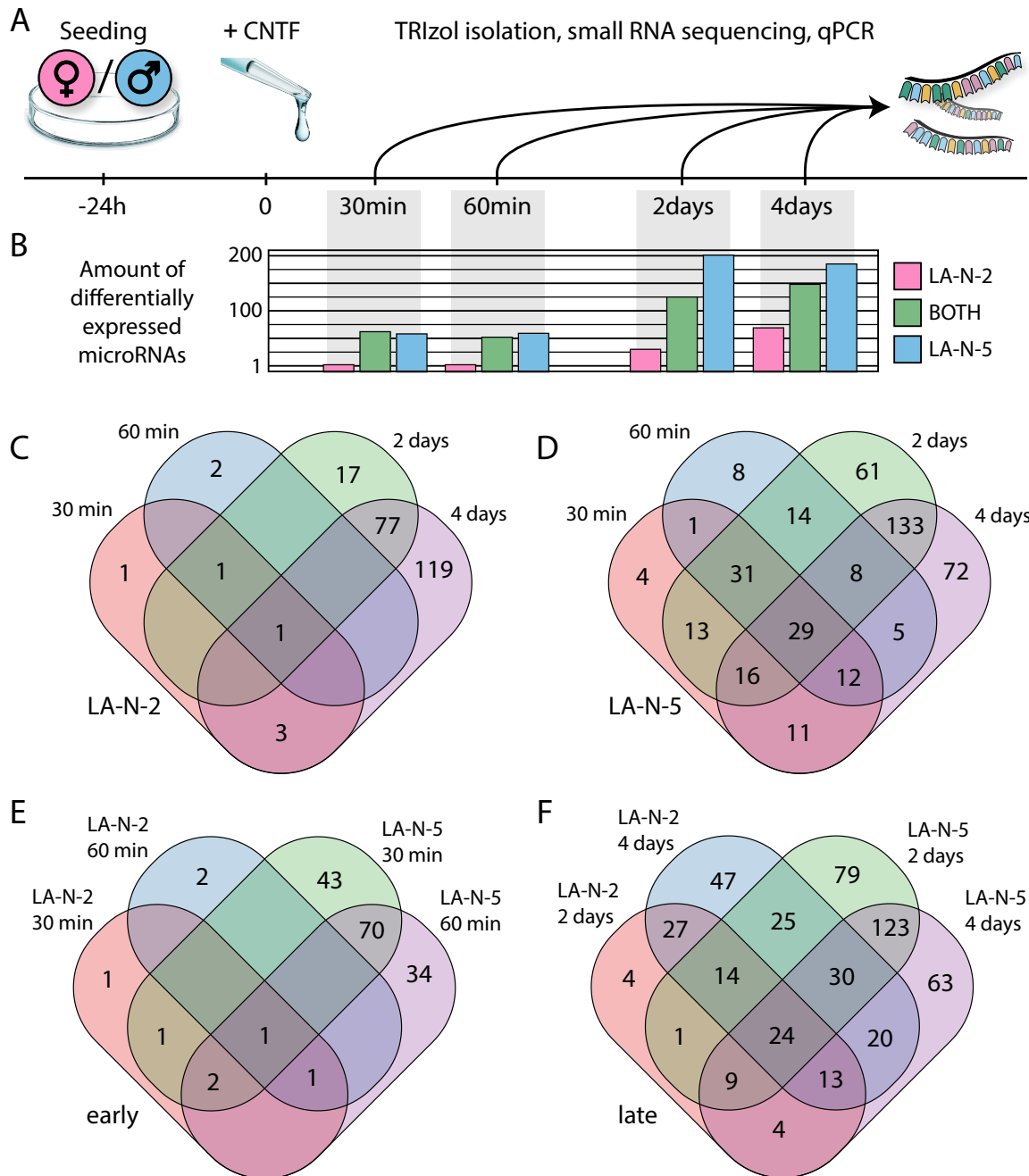
Figure 3.8: LA-N-2 / LA-N-5 Timeline and Differential Expression. A ) Experimental timeline of CNTF differentiation. B ) Bar plot of differentially expressed (DE) miRNAs per time point, divided by cell line where differential expression was measured (LA-N-2 only, LA-N-5 only, or both). C ) Venn diagram of DE miRNAs in LA-N-2, divided by time point. Few early DE miRNAs, and continually more the longer differentiation lasts. D ) Venn diagram of DE miRNAs in LA-N-5, divided by time point. Similar in pattern to C , but more pronounced in numbers. E ) Intersection of early time points in LA-N-2 and LA-N-5. Despite the low differential expression in LA-N-2, there is overlap. F ) Intersection of late time points in LA-N-2 and LA-N-5. Overlap is pronounced and complex, however, there are also cell line-exclusive miRNAs.
