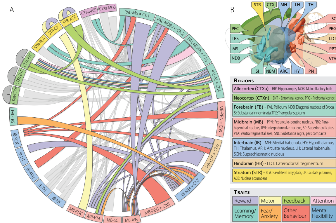
Figure 1.1: Cholinergic Projections in the CNS. Cholinergic systems are implicated in many diverse functional categories. A) The bulk of cholinergic projection neurons stems from one of the eight cholinergic nuclei, Ch1-Ch8 (right side of ideogram). They innervate wide areas of the mammalian CNS, and in turn receive incoming connections from all around the brain (left side of ideogram). Efferent connections are indicated by a small gap between ideogram and connector, in the first clockwise half of each ideogram component, afferent connection by a large gap, in the second half. A number of projections has been associated with specific functions, as implicated by the colours of the connectors. Two populations of cholinergic interneurons have been identified, in the striatum and the neocortex (outside of ideogram). B) Brain region and trait colour legend for A).
