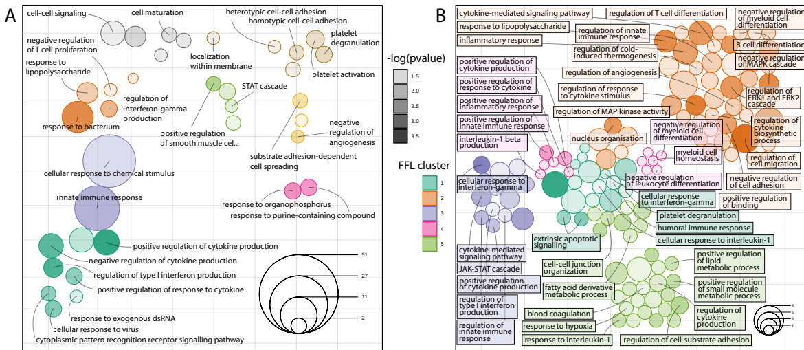
Figure 4.11: FFL module Gene Ontology Enrichment Increases Informative Resolution. A comparison between GO enrichment performed on (A) differentially expressed (DE) genes and (B) DE genes classified by FFL network modules shows similar biological processes but increased information depth. Size denotes number of significant genes in term, depth of colour indicates p-value (all p < 0.05 ). A) Differentially expressed genes with absolute \log_2 fold change > 1.4 are enriched in processes of immunity and circulation. Cluster colour derived from t-SNE similarity. Reproduction of Figure 4.2. B) t-SNE mapping of GO terms derived from analysis of single FFL modules shows details of involvement with immune processes and basic cellular function. Colour indicates original FFL module (see text). The middle cluster, comprised of parts from all modules surrounding module 1, may signify an »area of cooperation« between the modules.
