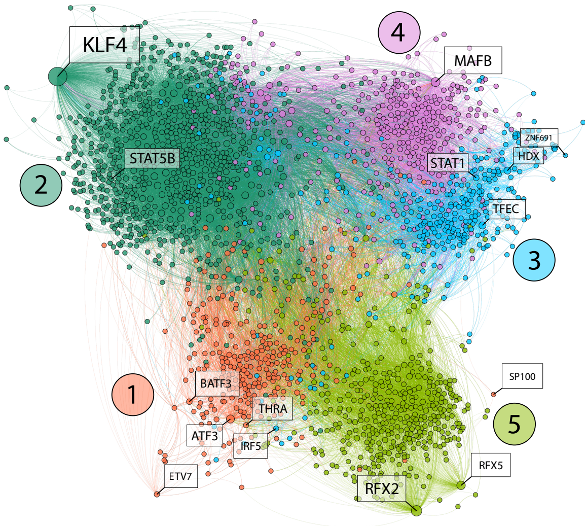
Figure 4.10: Complete Feedforward Loop Network of Differentially Expressed Transcription Factors in CD14 + Monocytes. Feedforward loops (FFLs) were created by miRNeo query of transcriptional interaction of transcription factors (TFs), miRNAs, and tRFs towards all genes, but limited to FFLs of which the regulatory elements (TFs and smRNAs) were present and active in CD14 + monocytes, and additionally filtered for the top 10% TF→gene relationships by activity. The resulting network was assembled in a force-directed 2D-projection and analysed to yield modularity information. The algorithm identified 5 distinct modules of small and large RNA FFLs, indicated by colours and numbers in circles. TFs differentially expressed in stroke patient blood are marked with a name tag (node size denotes differential expression count-change of TFs).
