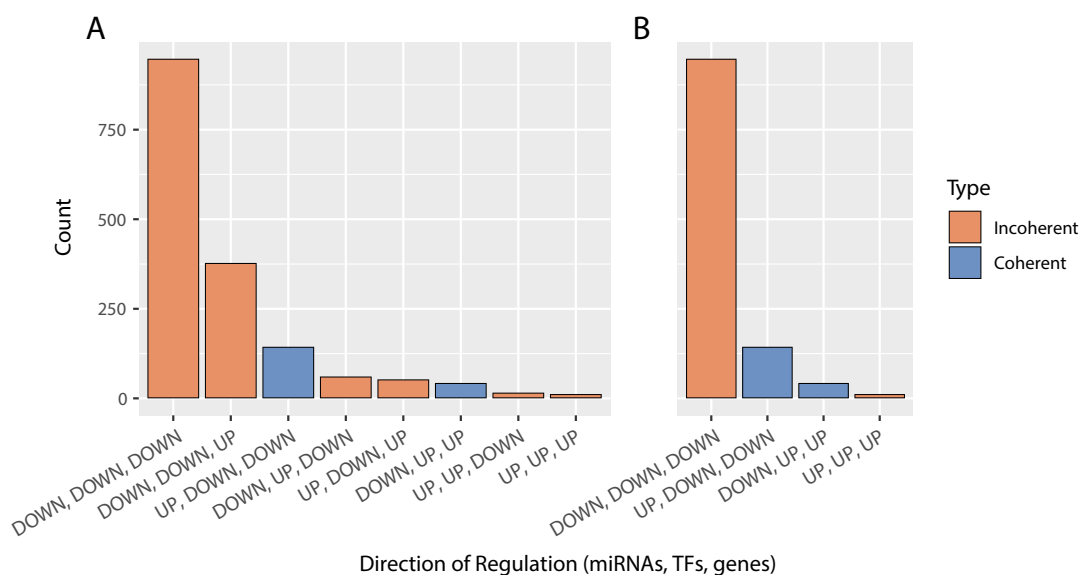
Figure 5.6: Coherence of miRNA Feedforward Loops. Individual FFLs were classified based on the direction of regulation of each of their components (miRNAs, TFs, and non-TF genes) in the blood of stroke patients, as determined via RNA-seq. Barplots represent the count of each class of FFL, colour denotes coherence. Incoherent FFLs dominate quantitatively. A) Barplot of all possible types of FFLs. B) Barplots of FFLs only with coherent TF → gene relationships (both either up- or down-regulated).
