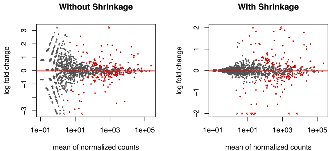
Figure 3.6: MD Plot Shrinkage Comparison. A mean-difference plot (MD Plot) is a plot of log-intensity ratios (differences, »M-values«) versus log-intensity averages (means, »A-values«); it is synonymous with »MA Plot«. The DESeq2 function plotMD shows the log fold changes attributable to a given variable over the mean of normalised counts for all the samples in the data set. Points are coloured red if the adjusted p value is less than 0.1. Points which fall out of the window are plotted as open triangles pointing either up or down. The left plot is generated from the standard linear model, the plot on the right is corrected by the »apeglm« algorithm 168 to reduce noise in the low-count fragments (data from LA-N-2 CNTF vs control on day 4).
