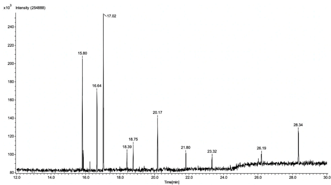
Figure S1. GC-MS chromatogram of H-Anvi extract
