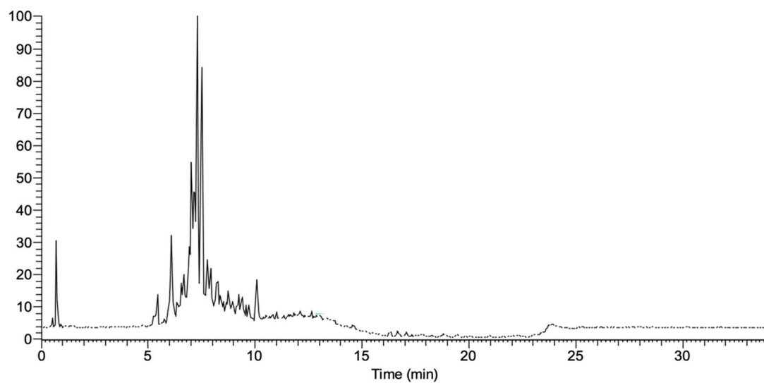
Figure S2. HPLC chromatogram of E-Anvi extract
