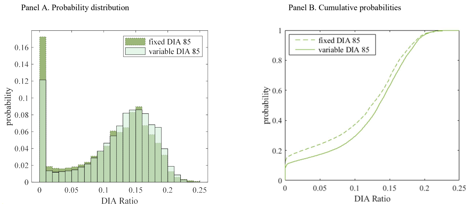
Figure 5: Distribution of optimal DIA ratios with fixed vs variable deferred annuities
