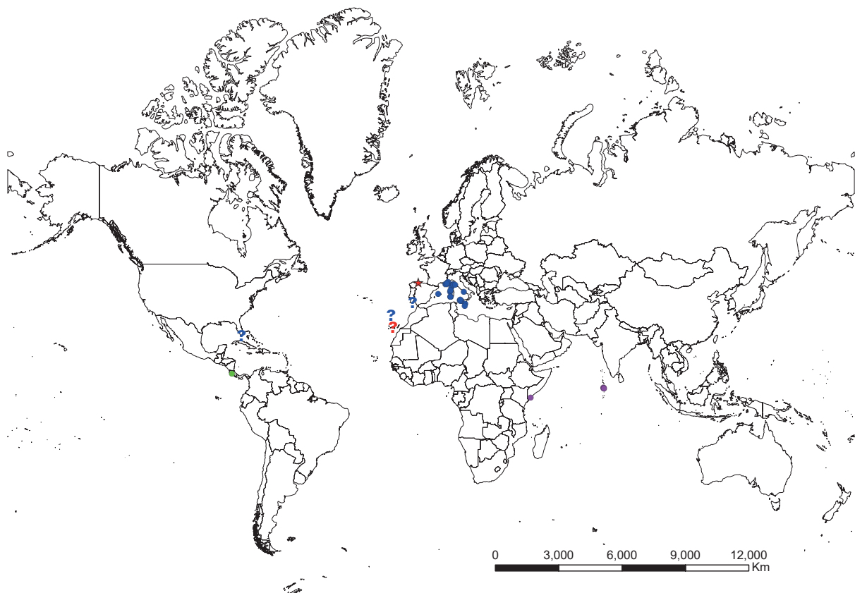
Fig. 7. Distribution of different species of Buchnerillo Verhoeff, 1942: B. litoralis Verhoeff, 1942 (●), unconfirmed records of B. litoralis (?), B. oceanicus Ferrara, 1974 (●), B. neotropialis Taiti, Montesanto & Vargas, 2018 (●), B. atlanticus sp. nov. (★) and unconfirmed records of B. atlanticus sp. nov. (?).
