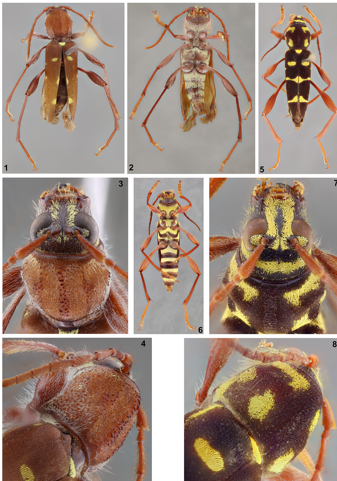
Figures 1–8. Cotyclytus spp. 1–4) Cotyclytus parumnotatus (Zajciw, 1963), neotype male: 1) Dorsal habitus; 2) Ventral habitus; 3) Head and pronotum, frontal view; 4) Head and pronotum, oblique view. 5–8) Cotyclytus stillatus (Aurivillius, 1909), male from Bolivia: 5) Dorsal habitus; 6) Ventral habitus; 7) Head and pronotum, frontal view; 8) Head and pronotum, oblique view.
