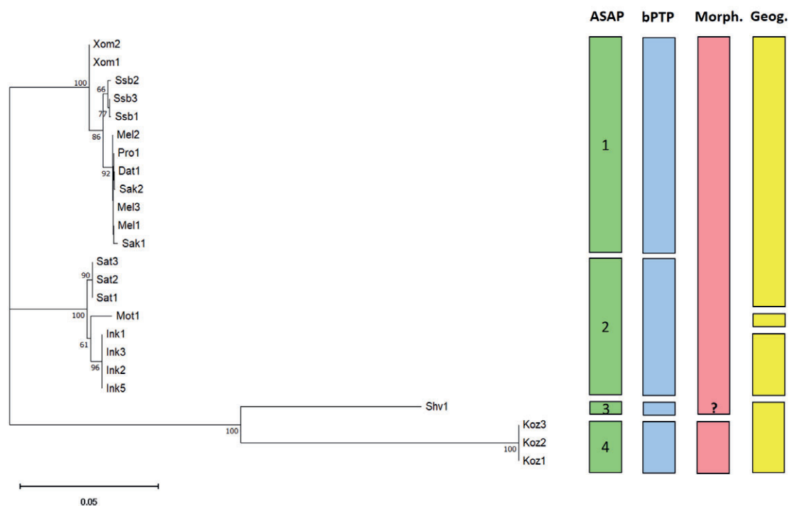
Fig. 2. A neighbour-joining tree (NJ) with species delimitation of Georgian cave populations of Deuteraphorura Absolon, 1901 based on COI molecular marker, morphology and geographic location in karst areas. Numbers and coloured columns indicate groups (species) identified by particular methods ASAP (Assemble Species by Automatic Partitioning) and bPTP (Bayesian Poisson tree processes). The question mark (?) indicates ambiguous result in Shvilobisa Cave due to low number of studied specimens. For abbreviations of caves in the NJ tree see Table 1.
