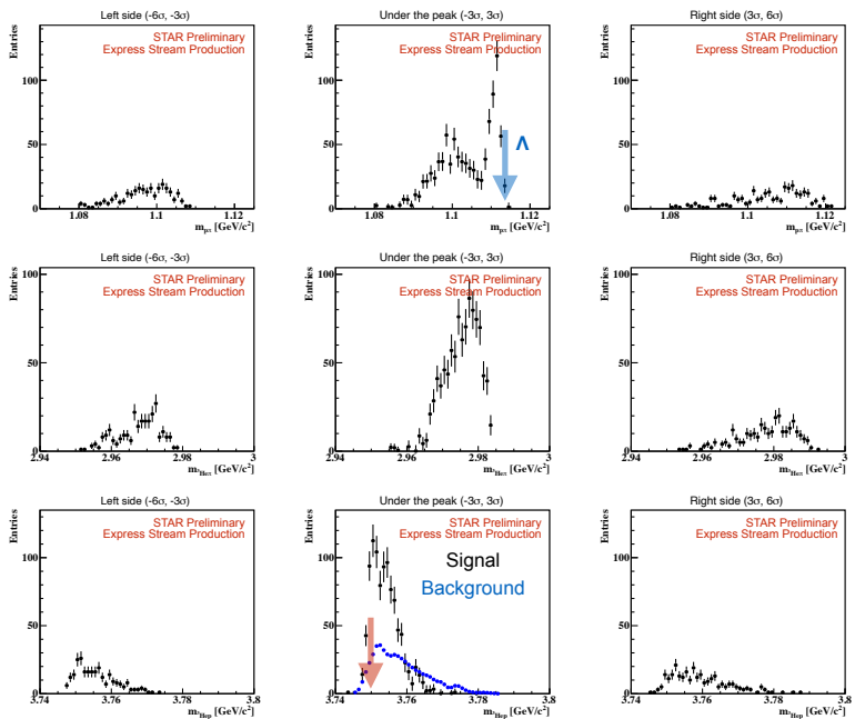
Figure 5. Projections of the Dalitz plots for the decay {}^4_{\Lambda}\text{He} \rightarrow {}^3\text{He} + p + \pi^- . The complex structure in the signal in the p\pi^- projection can be explained as a possible spin effect. In the nucleus-p combination, the signal and the background show different behavior. There can be seen a hint of two-body {}^4\text{Li} \pi^- decay ( {}^4\text{Li} (J^P = 2^-) : M = 3.75 \text{ GeV}/c^2 , \sigma = 8.7 \text{ MeV}/c^2 ).
