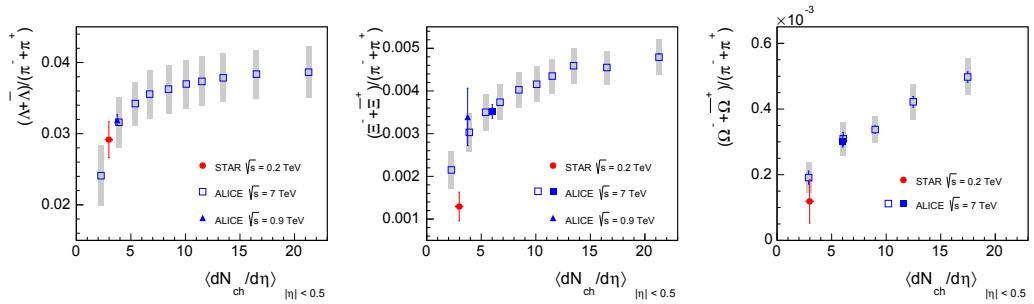
Figure 5. The yield ratios of strange particles to pions measured in multiplicity selected pp collisions at \sqrt{s} = 7 TeV [11] and in minimum bias pp collisions measured at various energies by ALICE [12, 13] and STAR [14, 15] as a function of dN_{ch}/d\eta .
