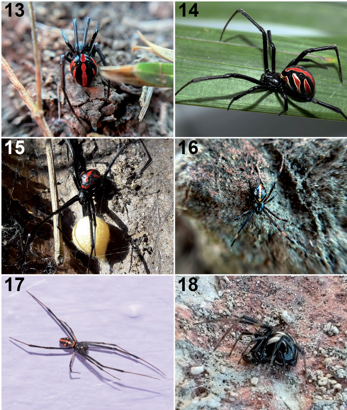
Figs 13–18. Live females (13–15) and males (16–18) of Latrodectus occidentalis Valdez-Mondragón sp. nov. 13, 16. Salvatierra, Guanajuato, Mexico. 14. Camichines, Cocula, Jalisco, Mexico (type locality). 15. Hostotipaquillo, Jalisco, Mexico. 17. 1 km North of San Nicolás de Ibarra, Jalisco, Mexico. 18. “Las Letras”, Pénjamo, Guanajuato, Mexico. Photographs 13, 16, 18 by Cabrera-Espinosa (2021). Photograph 14 by Navarro-Rodríguez I. (2021). Photograph 15 by Valdez-Mondragon A. Photograph 17 by Mamole in https://www.naturalista.mx/observations/126985294
