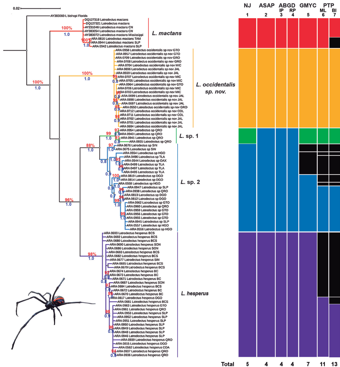
Fig. 3. Bayesian Inference tree (BI) constructed with the concatenated matrix ( COI + ITS2 ) of barcode sequences of Latrodectus Walckenaer, 1805 from Mexico. Branch colors indicate putative species and correspond to vertical bars, which represent different species delimitation methods used for their validation. Numbers below bars represent the number of species recovered in each species delimitation method (not considering the outgroup: L. bishopi ): 1: Neighbor-Joining (NJ); 2: ASAP; 3: ABGD with initial partitions (IP); 4: ABGD with recursive partitions (RP); 5: GMYC; 6: bPTP with ML; 7: bPTP with IB; Numbers above branches are bootstrap support values under NJ (>50% significant), number below branches are posterior probabilities (PP) support values under BI (>95% significant).
