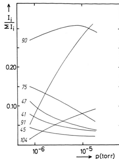
Fig. 3. Mass-corrected relative intensities of the major ions in the ICR spectrum of (CH_3)_3PCH_2 as a function of the total pressure.
