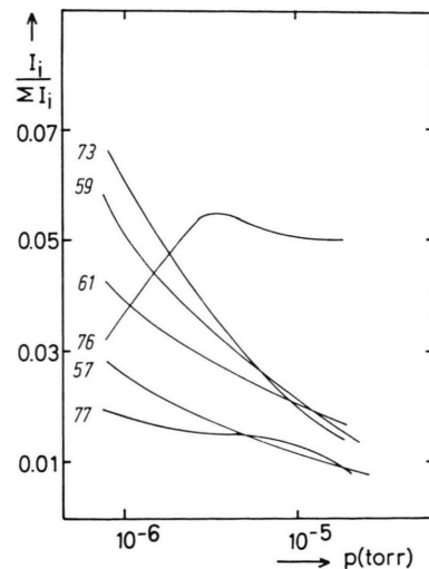
Fig. 4. Mass-corrected relative intensities of the medium abundant ion in the ICR spectrum of (CH_3)_3PCH_2 as a function of the total pressure.
