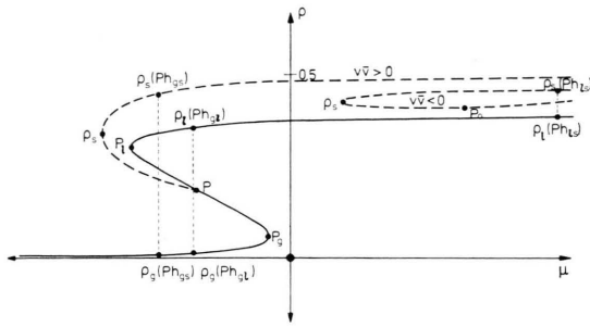
Fig. 5. q(\mu) -isotherms of the lattice gas with attractive total interaction ( v > 0 ) at low temperatures. — fluid phases; - - - - solid phases for v\bar{v} \geq 0 .
