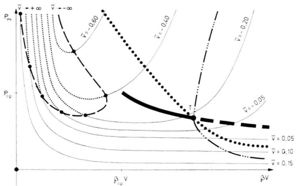
Fig. 7. The pressure p_{ph} of the lattice gas on the curves of coexistence as a function of \beta v , for attractive total particle interaction ( v > 0 ), for the two- and three dimensional lattice.
