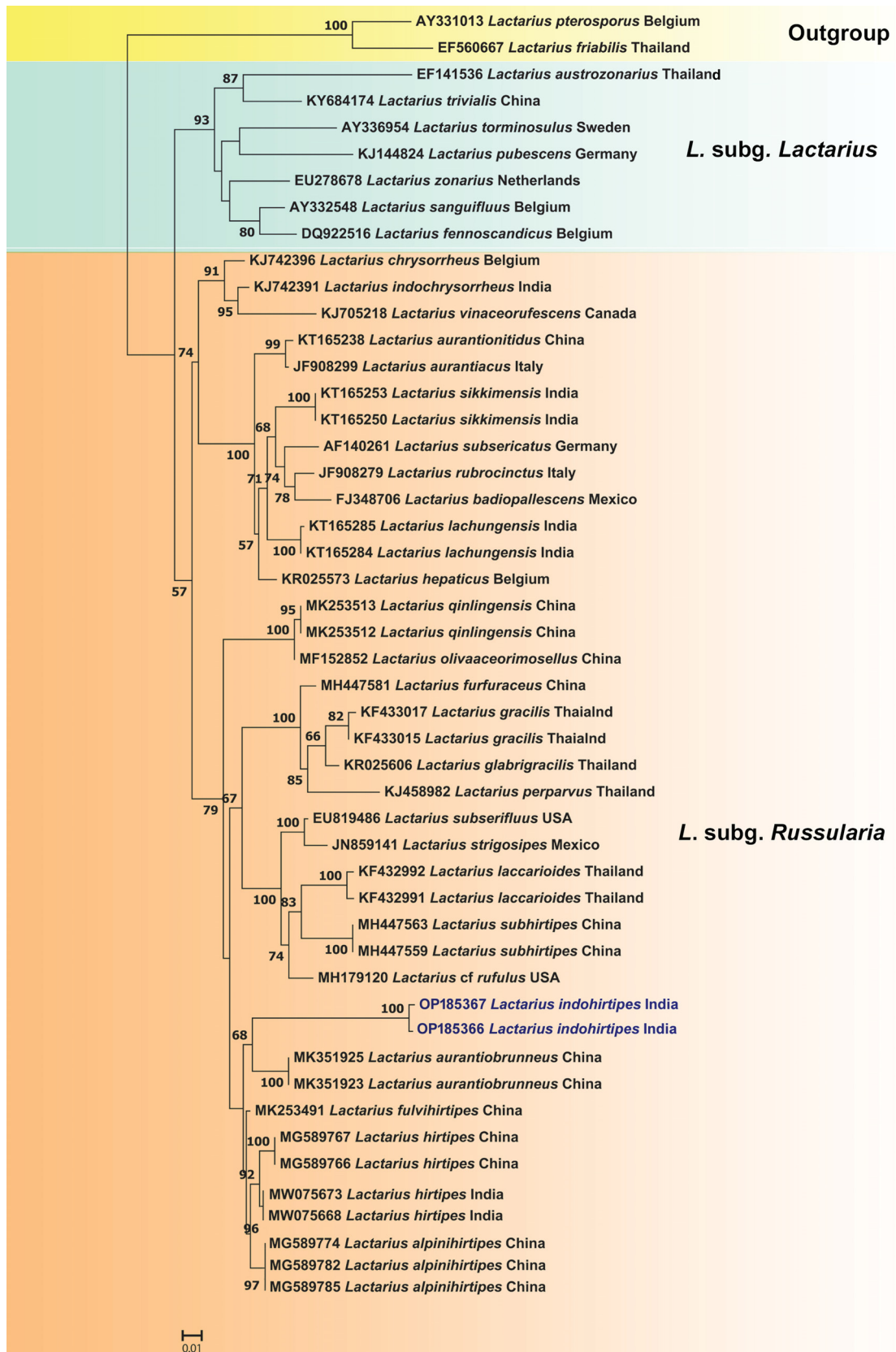
Fig. 1. ML phylogram (RAxML) inferred from the nrITS alignment. Lactarius indohirtipes K.Verma, Uniyal & Mehmood sp. nov. is highlighted in bold blue.
