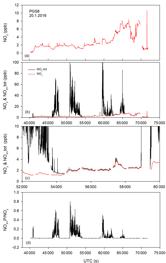
Figure 11. POLSTRACC flight on 20 January 2016. During this flight, particulate nitrate was observed. (a) Gas-phase NO_y , (b) total nitrate (including particulate nitrate) and gas-phase nitrate, (c) same as (b) but with a smaller time interval, and (d) ratio of particulate nitrate (corrected for enhancement) to gas-phase nitrate.
