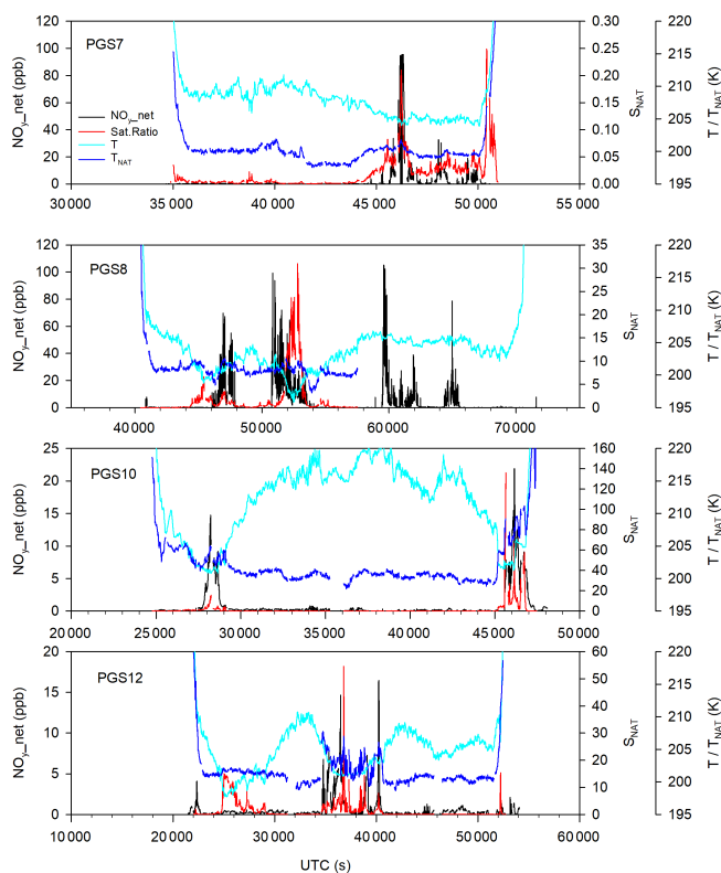
Figure 13. \text{NO}_y net, ambient temperature, saturation ratio, and T_{\text{NAT}} for all flights where particulate nitrate was observed. During the second half of the flight, PGS flight 8 the NAT saturation temperature, T_{\text{NAT}} , could not be calculated because of missing data.
