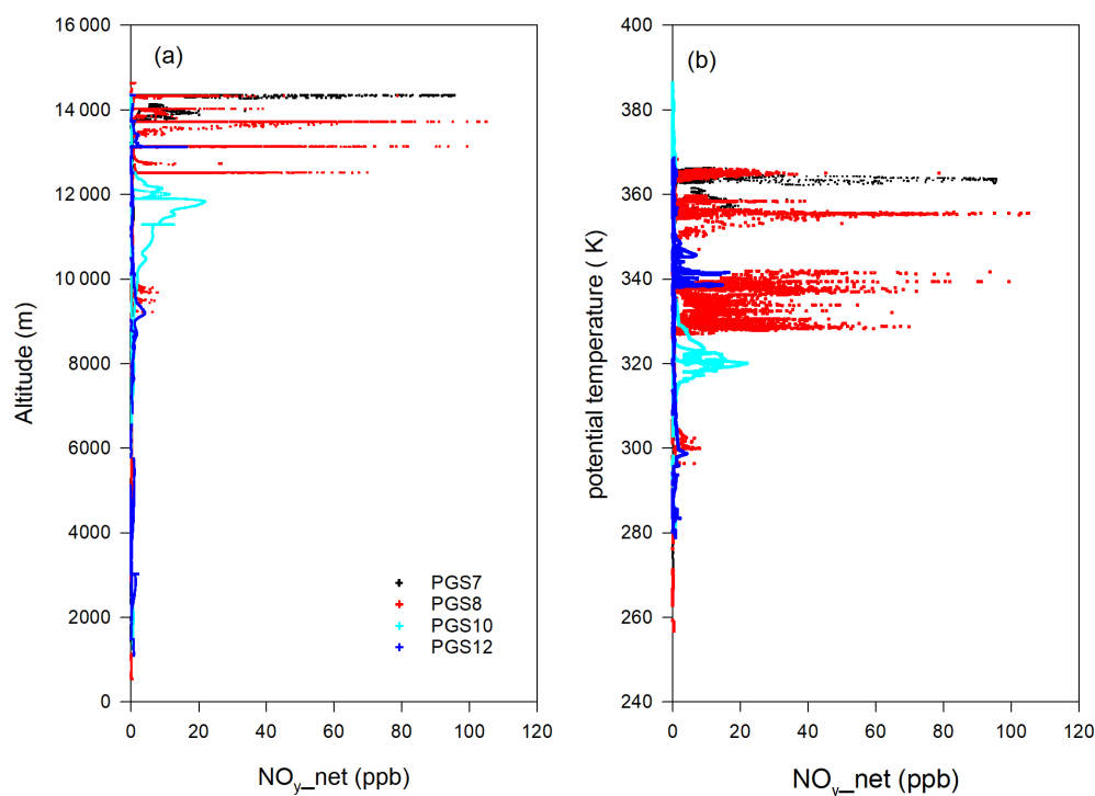
Figure 12. \text{NO}_y\text{-net} versus altitude (a) and \text{NO}_y\text{-net} versus potential temperature (b) for all flights with the occurrence of particulate nitrate (18, 20, 25, 31 January 2016).
