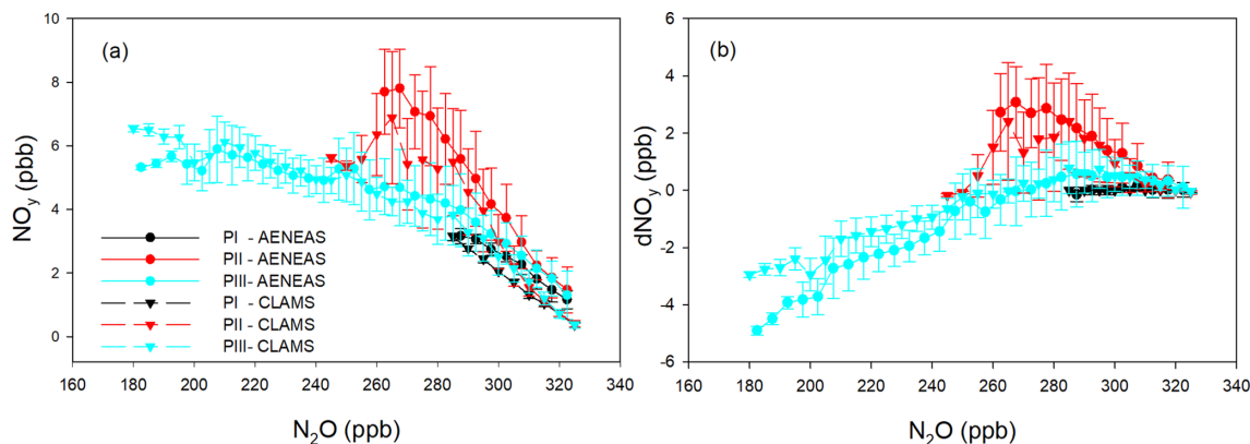
Figure 17. (a) \text{NO}_y and (b) d\text{NO}_y averaged over 5 ppb \text{N}_2\text{O} intervals along with standard deviations for the three mission phases. Observed values (circles) are shown along with values from the CLaMS model simulation (triangles).
