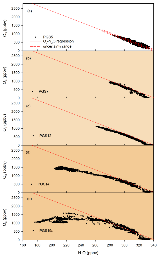
Figure 10. O_3 versus N_2O for selected flights (same as in Fig. 6) in three observational phases. Early winter: PGS flight 5 – 21 December 2015, mid-winter: PGS flight 7 – 18 January 2016 and PGS flight 12 – 31 January 2016, late winter: PGS flight 14 – 26 February 2016 and PGS flight 19a – 13 March 2016. Additionally, the regression line resulting from the December flight is given. The uncertainty range of the regression is indicated by dashed lines.
