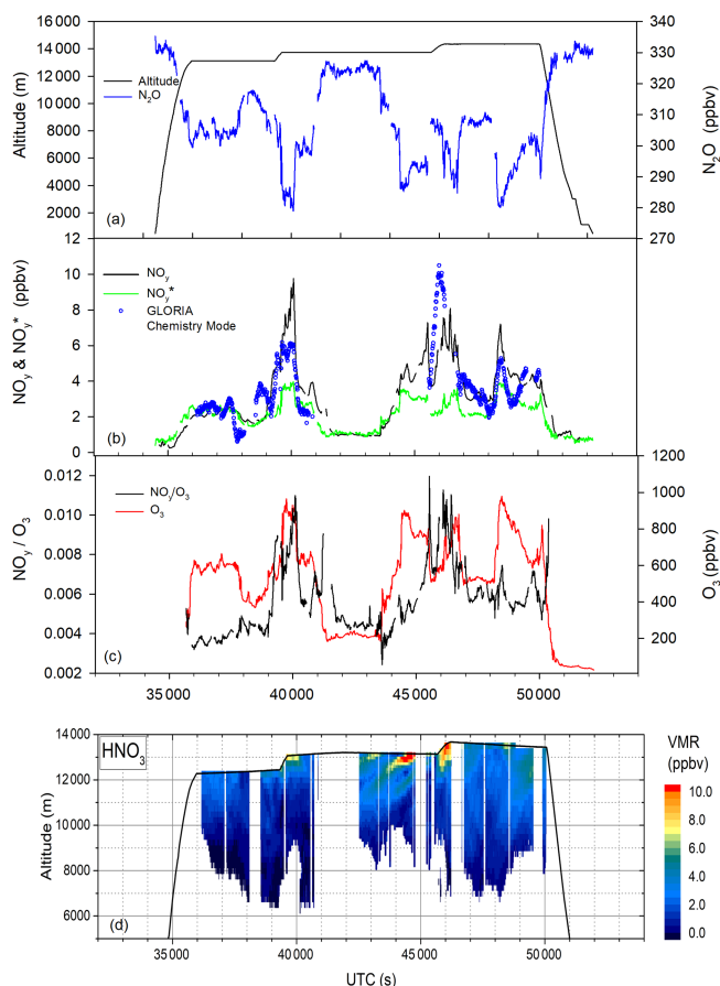
Figure 2. PGS flight 7 on 18 January 2016. (a) Altitude and N 2 O; (b) NO y (observed), NO y * (calculated), and HNO 3 (GLORIA instrument); (c) NO y /O 3 ratio and O 3 ; and (d) HNO 3 observed with GLORIA.
