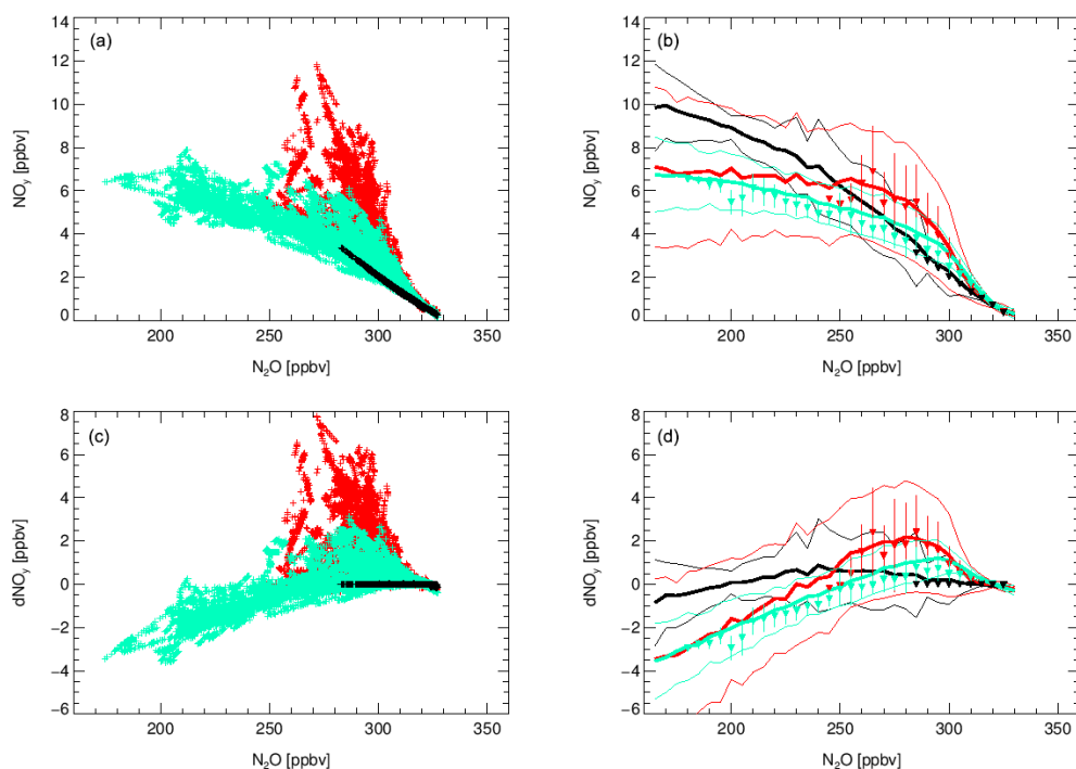
Figure 16. Correlations of \text{NO}_y (a, b) and d\text{NO}_y (c, d) with \text{N}_2\text{O} from CLaMS simulations. The left panels show all dates in different colours for the three campaign phases. Data within 5 min of the times 31 January 2016 14:17 and 13 March 2016 11:20 UTC are omitted (see text). The right panels show the averages for \text{N}_2\text{O} bins \pm 1\sigma standard deviations of these values as filled triangles with error bar signs. Also shown are the vortex average correlation for central dates of the campaign phases as thick coloured lines, \pm 1\sigma standard deviation is indicated as thin coloured lines.
