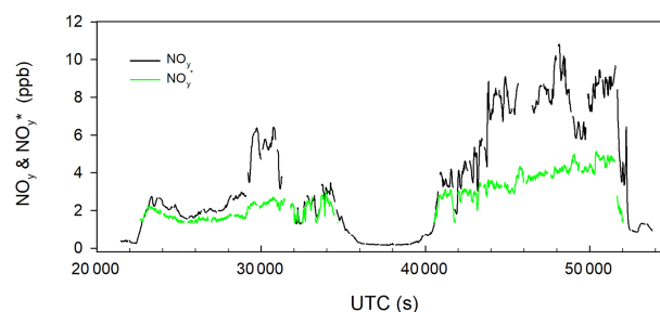
Figure 3. PGS flight 12 on 31 January 2016. NO y (observed) and NO y * (calculated).
