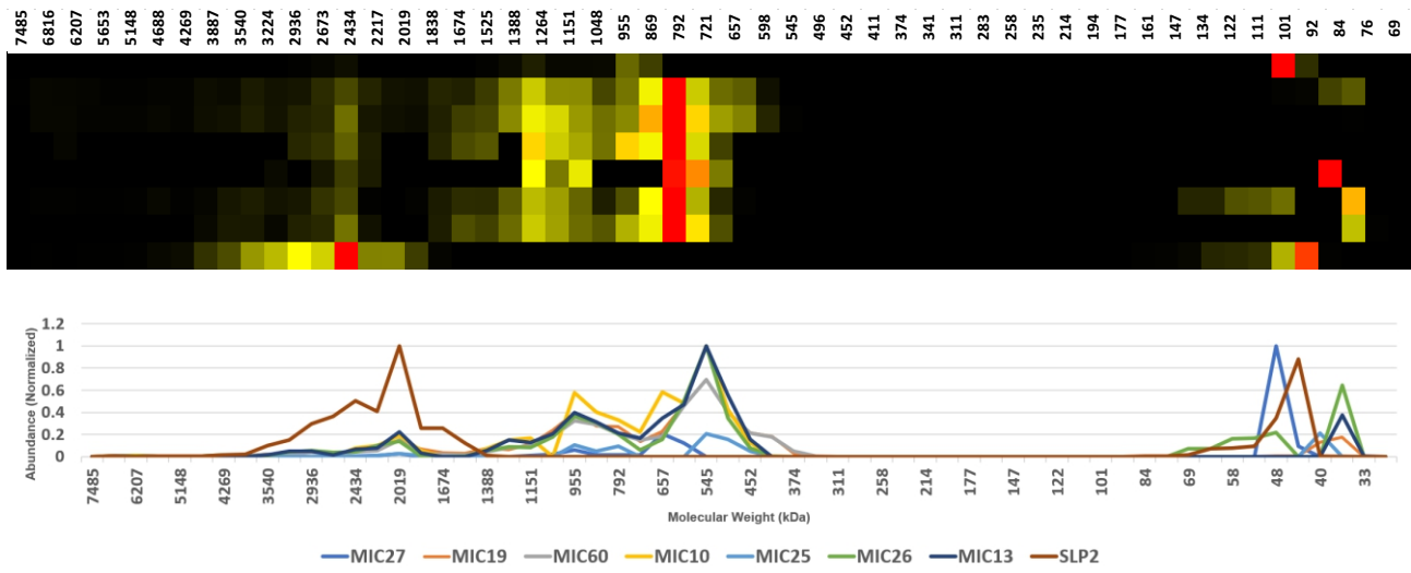
Supplementary Figure 1. A heatmap and graph represent the normalized occurrence of SLP2 and MICOS subunits in complexome profiling data obtained from the HEK293 cells studied previously (Anand et al., 2016). SLP2 co-clustered with high molecular weight MICOS complex around 2000 kDa.
