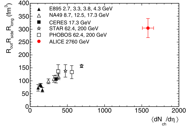
Fig. 4. Product of the three pion HBT radii at k_T = 0.3 GeV/c. The ALICE result (red filled dot) is compared to those obtained for central gold and lead collisions at lower energies at the AGS [35], SPS [36–38], and RHIC [39–42,30,43]. (For interpretation of the references to color in this figure legend, the reader is referred to the web version of this Letter.)
