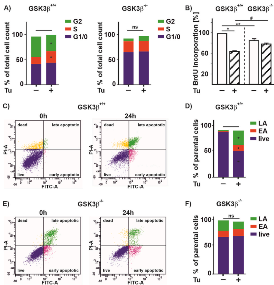
Fig. 8. Lack of GSK3 \beta affects proliferation and apoptosis upon tunicamycin treatment (A) Cell cycle distribution of GSK3 \beta^{+/+} MEFs and GSK3 \beta^{-/-} MEFs upon Tu (10 \mu g/ml) treatment for 24 h. G1/0 phase (blue fraction), S phase (red fraction), and G2 phase (green fraction). (B) BrdU incorporation in GSK3 \beta^{+/+} and GSK3 \beta^{-/-} cells, *significance GSK3 \beta^{+/+} vs GSK3 \beta^{+/+} + Tu, **significance GSK3 \beta^{+/+} vs GSK3 \beta^{-/-} , #significance GSK3 \beta^{+/+} + Tu vs GSK3 \beta^{-/-} + Tu, p \leq 0.05 , n = 4 . (C, E) Histograms of apoptosis in GSK3 \beta^{+/+} and GSK3 \beta^{-/-} cells was assessed by Annexin-V/PI staining and measured by flow cytometry. (D, F) Quantification of apoptosis in GSK3 \beta^{+/+} and GSK3 \beta^{-/-} . Live cells (blue fraction), early apoptotic cells (red fraction; EA), and late apoptotic cells (green fraction; LA), *significance GSK3 \beta^{+/+} vs GSK3 \beta^{+/+} + Tu, p \leq 0.05 , n = 4 . (For interpretation of the references to colour in this figure legend, the reader is referred to the Web version of this article.)
