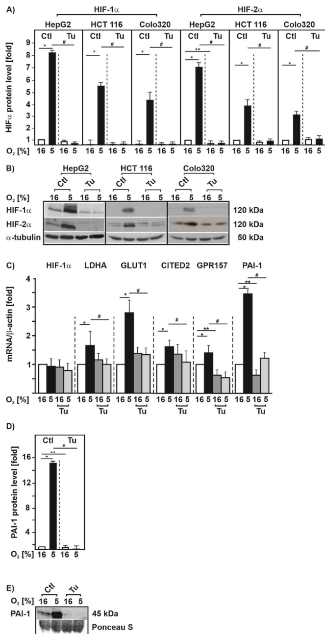
Fig. 2. ER stress inhibits hypoxia-dependent induction of HIF-1 \alpha and HIF-2 \alpha as well as HIF target gene expression
