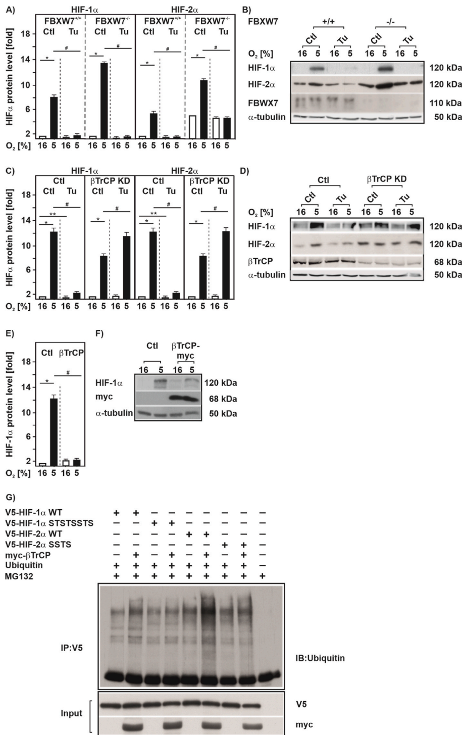
Fig. 7. Tunicamycin downregulates HIF-1 \alpha in a \beta TrCP-dependent manner (A) FBXW7 +/+ and FBXW7 -/- were cultured under normoxia (16% O 2 ) for 24 h, then treated with Tu (10 \mu g/ml) and further cultured either under normoxia or hypoxia (5% O 2 ) for 4 h. HIF-1 \alpha protein levels measured by Western blot under normoxia (16% O 2 ) were set to 1. *significance 16% O 2 vs 5% O 2 ; #significance 5% O 2 vs 5% O 2 + Tu, p \leq 0.05, n = 3. (C) MDA-MB 231 cells with an inducible \beta TrCP knock-down were cultured for 24 h under normoxia (16% O 2 ) and treated with IPTG (1 mM) for 72 h prior to treatment with Tu (10 \mu g/ml). HIF-1 \alpha protein levels measured under normoxia (16% O 2 ) were set to 1. *significance 16% O 2 vs 5% O 2 ; **significance 16% O 2 vs 16% O 2 + Tu, #significance 5% O 2 vs 5% O 2 + Tu, p \leq 0.05, n = 3. (B, D) Representative Western blots of total protein analyzed with antibodies against HIF-1 \alpha , HIF-2 \alpha , FBXW7, \beta TrCP and \alpha -tubulin. (E) HEK 293 cells transfected myc-tagged wild-type \beta TrCP were cultured either under normoxia or hypoxia (5% O 2 ) for 4 h. HIF-1 \alpha protein levels measured by Western blot under normoxia (16% O 2 ) were set to 1. *significance 16% O 2 vs 5% O 2 ; #significance 5% O 2 vs 5% O 2 + Tu, p \leq 0.05, n = 3. (F) Representative Western blot. 100 \mu g of total protein were analyzed with antibodies against HIF-1 \alpha , myc-Tag and \alpha -tubulin. (G) Ubiquitylation assay. Ubiquitylated proteins are visualized by immunoblot (IB) analysis of anti-V5 immunoprecipitates (IP) and input from MG132 treated HEK 293 cells cotransfected with expression vectors for the V5-tagged full-length wild-type HIF-1 \alpha (WT), mutant HIF-1 \alpha (STSTSSTS), wild-type HIF-2 \alpha (WT), mutant HIF-2 \alpha (SSTS), and myc-tagged- \beta TrCP or ubiquitin.
