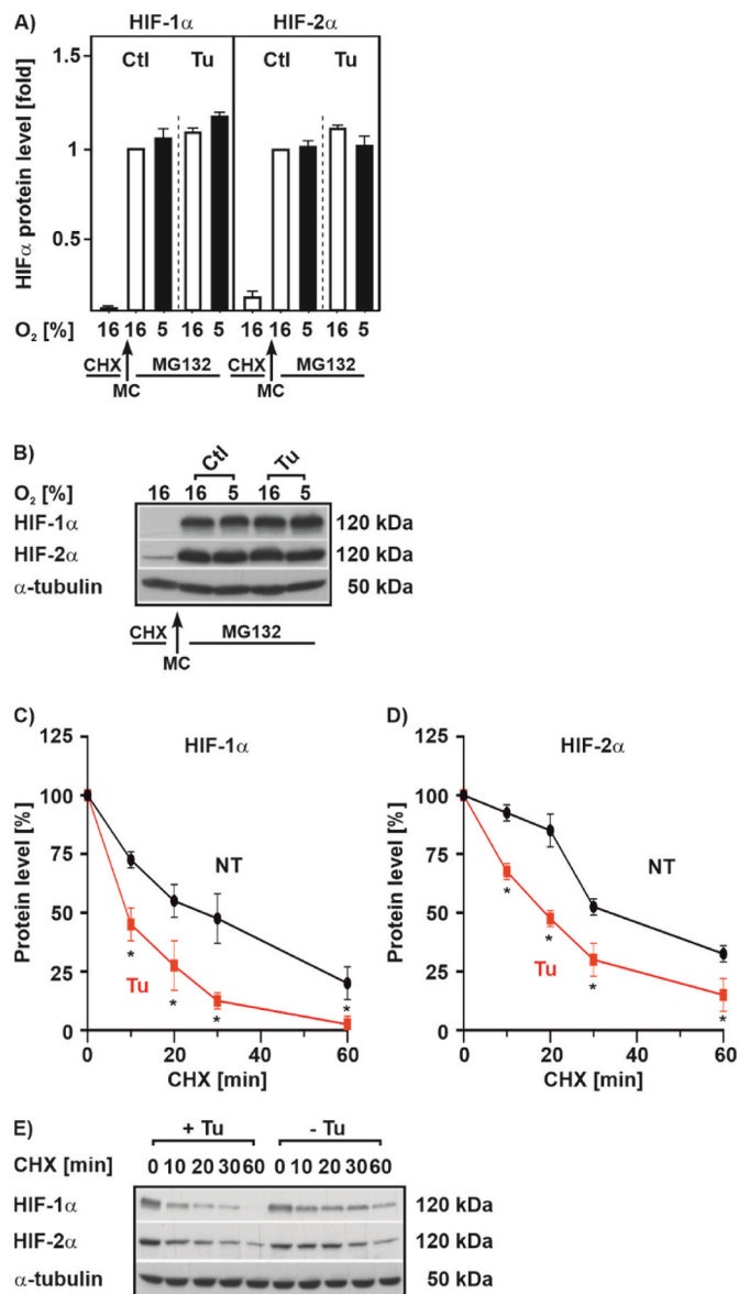
Fig. 5. Tunicamycin shortens HIF \alpha half-life but does not affect translation (A) HEK 293 cells were cultured for 4 h under normoxia (16% O 2 ) or hypoxia (5% O 2 ) in the presence of cycloheximide (CHX; 50 \mu M). Then, protein synthesis was restarted by a medium change (MC, fresh medium without cycloheximide) but containing MG132 (50 \mu M) to prevent degradation of newly synthesized proteins. Culture was continued under normoxia (16% O 2 ) or hypoxia (5% O 2 ) in the absence or presence of Tu (10 \mu g/ml) for 4 h. In each experiment HIF-1 \alpha or HIF-2 \alpha levels under 16% O 2 were set to 1. n = 3. (B, E) Representative Western blot of total protein analyzed with antibodies against HIF-1 \alpha , HIF-2 \alpha and \alpha -tubulin. (C, D) HEK 293 cells were cultured under hypoxia 5% O 2 for 24 h and after inhibition of protein synthesis with cycloheximide (10 \mu g/ml), the HIF-1 \alpha or HIF-2 \alpha protein half-life was measured by Western blot analysis. The HIF-1 \alpha or HIF-2 \alpha protein levels at 0 min were set to 100%. *significant differences non-treated (NT) vs Tu, p \leq 0.05, n = 3.
