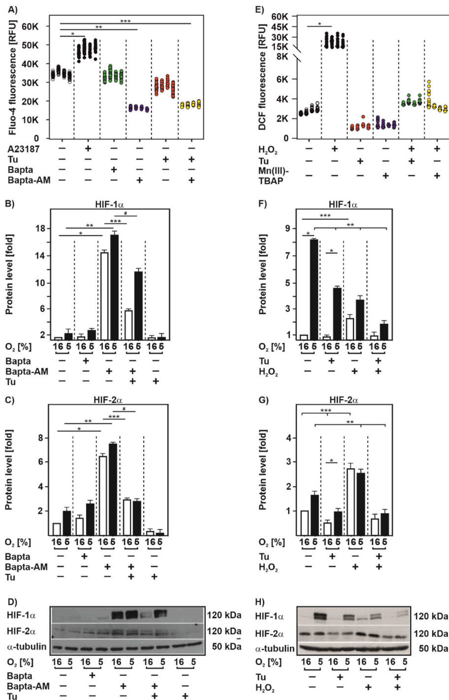
Fig. 4. HIF \alpha downregulation by tunicamycin occurs independent of Ca 2+ and ROS
