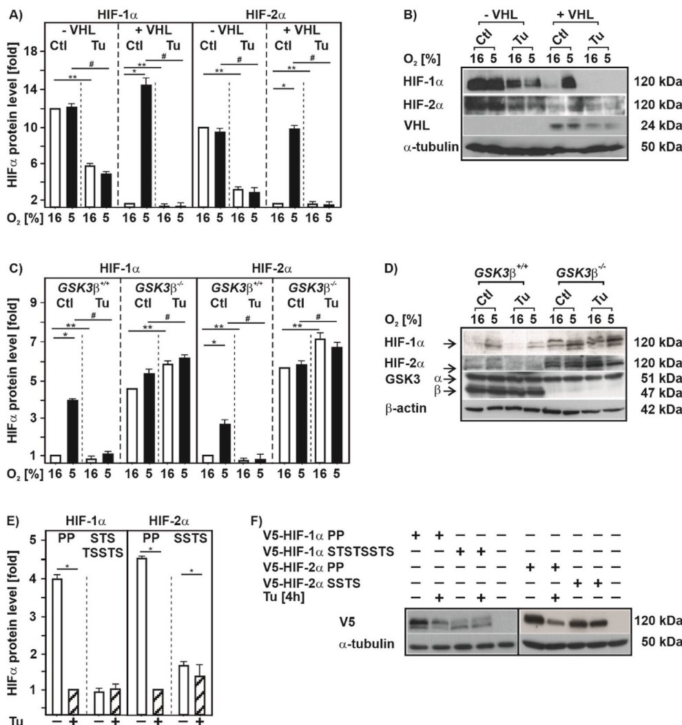
Fig. 6. Destabilization of HIF-1 \alpha and HIF-2 \alpha by tunicamycin is independent of VHL but dependent on GSK3 \beta (A, C) VHL-defective RCC4 cells (-VHL), the RCC4 cells with reintroduced VHL (+VHL), GSK3 \beta +/+ MEFs and GSK3 \beta -/- MEFs were cultured under normoxia (16% O 2 ) for 24 h, then treated with Tu (10 \mu g/ml) and further cultured under either normoxia or hypoxia (5% O 2 ) for 4 h. HIF-1 \alpha and HIF-2 \alpha levels measured under normoxia (16% O 2 ) were set to 1. *significance 16% O 2 vs 5% O 2 ; **significance 16% O 2 vs 16% O 2 + Tu, #significance 5% O 2 vs 5% O 2 + Tu, p \leq 0.05, n = 3. (B, D) Representative Western blots of total proteins analyzed with antibodies against HIF-1 \alpha , HIF-2 \alpha , VHL, GSK3 \alpha/\beta and \alpha -tubulin. (E) HEK 293 cells were transfected with expression vectors for V5-tagged full length HIF-1 \alpha mutants HIF-1 \alpha P402A/P564A (PP), HIF-1 \alpha T498V, S502A, S505A, T506A, S510A, S551A, T555V, S589A (STSTSSTS) or the full length HIF-2 \alpha mutants HIF-2 \alpha P405A, P531A (PP) and HIF-2 \alpha S475R, S477F, T481A, S484R (SSTS). After transfection, cells were treated with Tu (10 \mu g/ml) and further cultured under normoxia for 4 h. HIF \alpha protein levels measured by Western blot treated with Tu were set to 1. *significance non-treated vs + Tu, p \leq 0.05, n = 3. Note that the GSK3 site HIF1 \alpha STSTSSTS and HIF-2 \alpha SSTS mutants do not harbour mutations at the PP hydroxylation sites and are therefore less stabilized than the respective PP mutants. (F) Representative Western blots of total proteins analyzed with antibodies against V5 and \alpha -tubulin.
