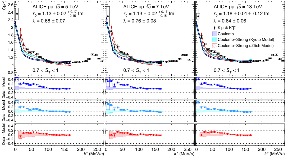
Fig. 2: (Color online) (K^-p \oplus K^+\bar{p}) correlation functions obtained from pp collisions at \sqrt{s} = 5 TeV (left), 7 TeV (middle) and 13 TeV (right) fitted with Eq. 1. The measurement is presented by the black markers, the vertical lines and the boxes represent the statistical and systematic uncertainties respectively. Three different potentials were considered: Coulomb potential (blue band), Kyoto model [44–48] (light blue band), Jülich model [49] where the physics masses of K^- and \bar{K}^0 are used [50] with the Coulomb interaction included (red band). In the bottom panels, differences between data and model are shown. The bands represent the systematic uncertainty related to the determination of the \lambda parameter and to the source radius.
