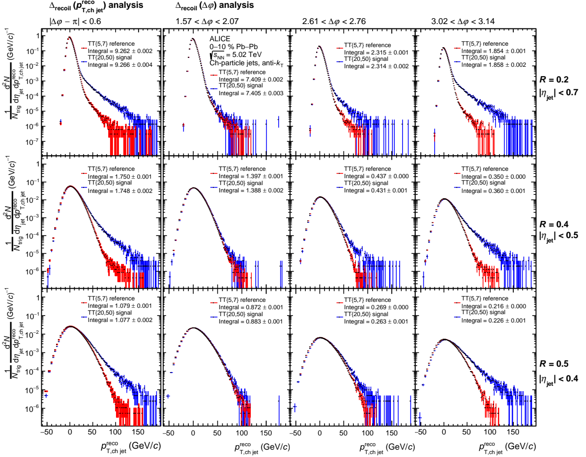
Figure 3: Trigger-normalized semi-inclusive recoil jet distributions for \text{TT}_{\text{sig}} and \text{TT}_{\text{ref}} -selected populations in central Pb–Pb collisions at \sqrt{s_{\text{NN}}} = 5.02 TeV, for R = 0.2 (upper panels), 0.4 (middle panels), and 0.5 (lower panels). The \Delta\phi correction (Sec. 4.1) has been applied to the \text{TT}_{\text{ref}} distributions. The left column shows distributions in the \Delta\phi acceptance of the \Delta_{\text{recoil}}(p_{\text{T, jet}}) analysis. The remaining columns show distributions in selected \Delta\phi bins for the \Delta_{\text{recoil}}(\Delta\phi) analysis, with the second column having the largest deviation from \Delta\phi = \pi and the rightmost column at \Delta\phi \sim \pi .
