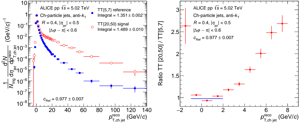
Figure 7: Left: trigger-normalized semi-inclusive recoil jet distributions with R = 0.4 for \text{TT}_{\text{sig}} and \text{TT}_{\text{ref}} -selected populations in pp collisions at \sqrt{s} = 5.02 TeV; Right: ratio of the two distributions. The horizontal blue line indicates the fit to the ratio close to p_{T, \text{ch jet}}^{\text{reco}} = 0 for the determination of c_{\text{Ref}} , the value of which is also given in the figures.
