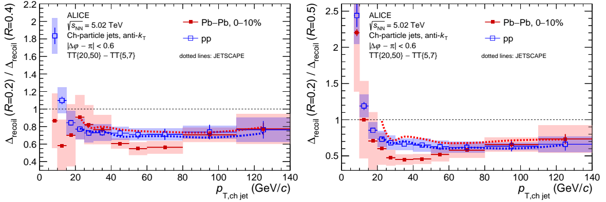
Figure 18: Ratio of \Delta_{\text{recoil}}(p_{T,\text{ch jet}}) distributions with different R for Pb–Pb collisions at \sqrt{s_{\text{NN}}} = 5.02 \text{ TeV} from the data in Fig. 13, together with the ratios for pp collisions from Fig. 17, for R = 0.2/R = 0.4 (left) and R = 0.2/R = 0.5 (right). The uncertainty in the ratio takes into account the correlation of uncertainties between numerator and denominator. JETSCAPE calculations for pp and Pb–Pb collisions are also shown.
