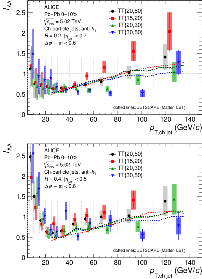
Figure 16: I_{AA}(p_{T,\text{ch jet}}) for R = 0.2 and 0.4 , for various TT_{\text{sig}} selections. The data points have been displaced for clarity, and the vertical dashed grey lines indicate the bin edges. JETSCAPE predictions for the corresponding TT_{\text{sig}} selections are also shown.
