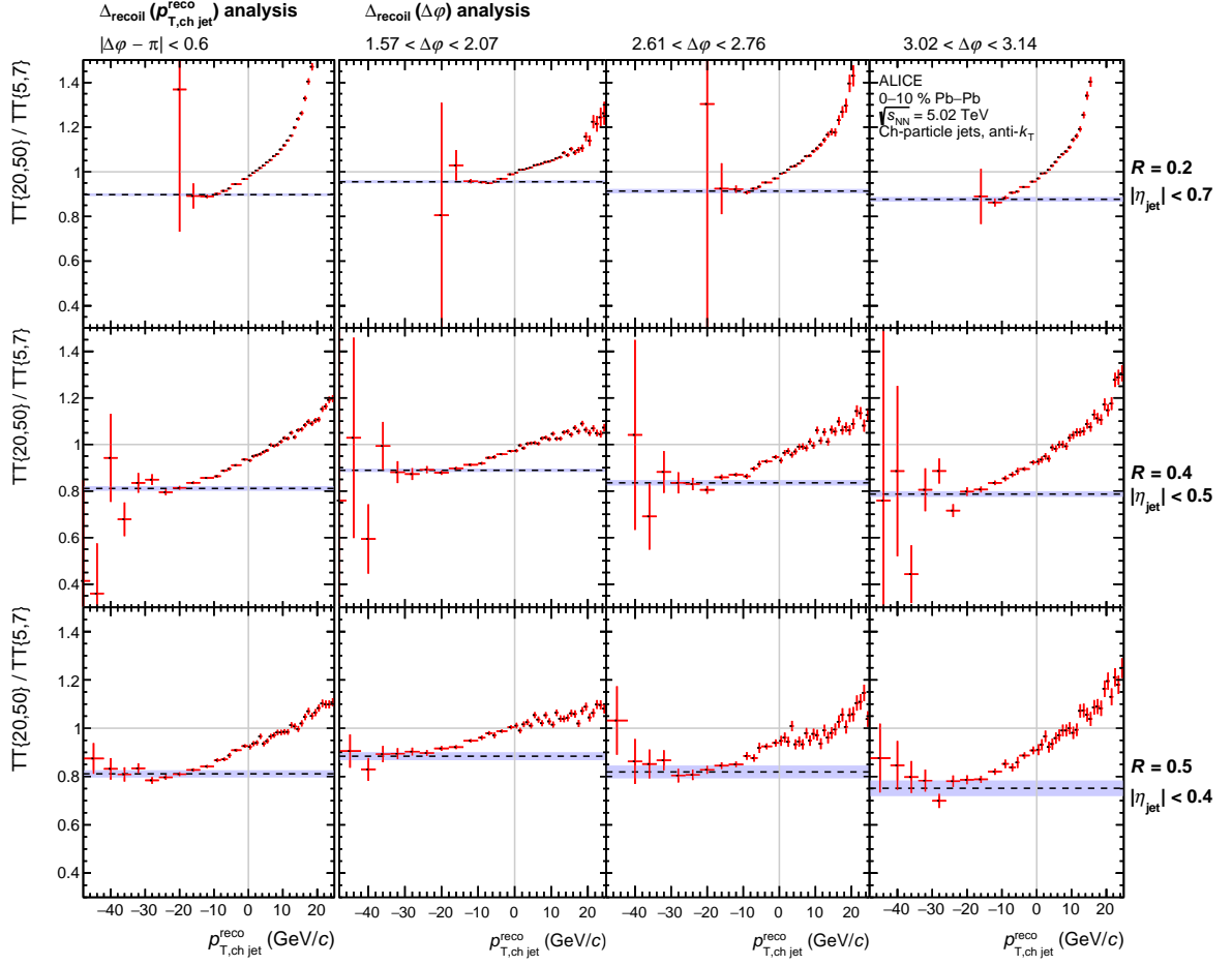
Figure 4: Ratio of TT_{\text{sig}} and TT_{\text{ref}} -selected distributions from Fig. 3, with the same panel layout. The horizontal dashed line and band show the value of c_{\text{Ref}} and its uncertainty. The vertical solid grey line is at p_{T,\text{ch jet}}^{\text{reco}} = 0 , and horizontal solid grey line is at unity. See text for details.
